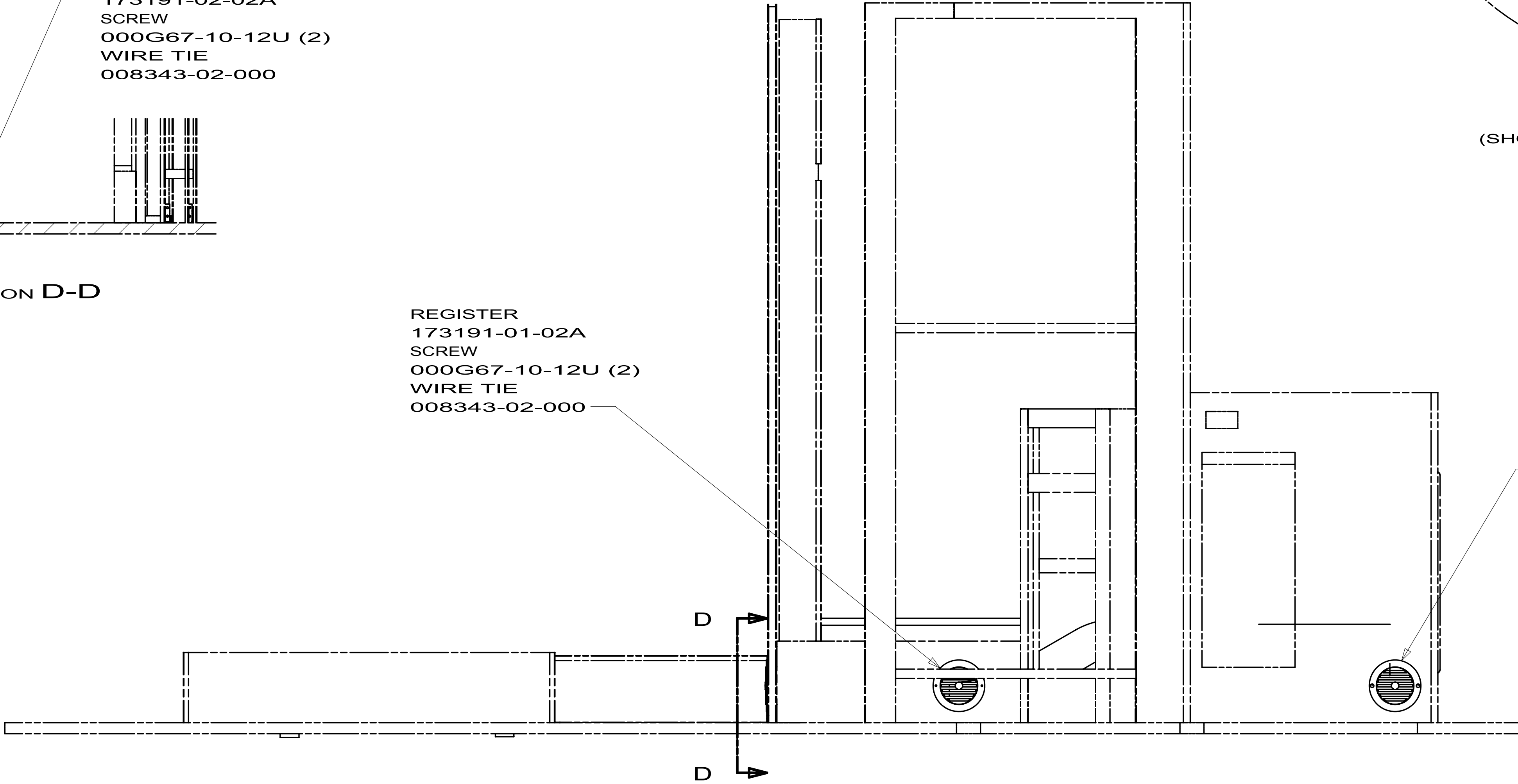
VIEW B
