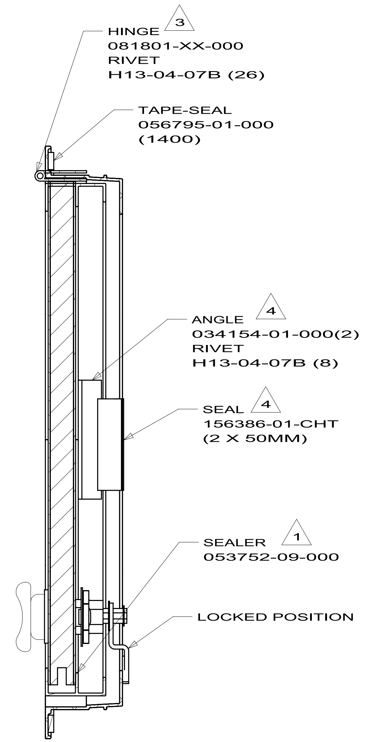
SECTION C-C
