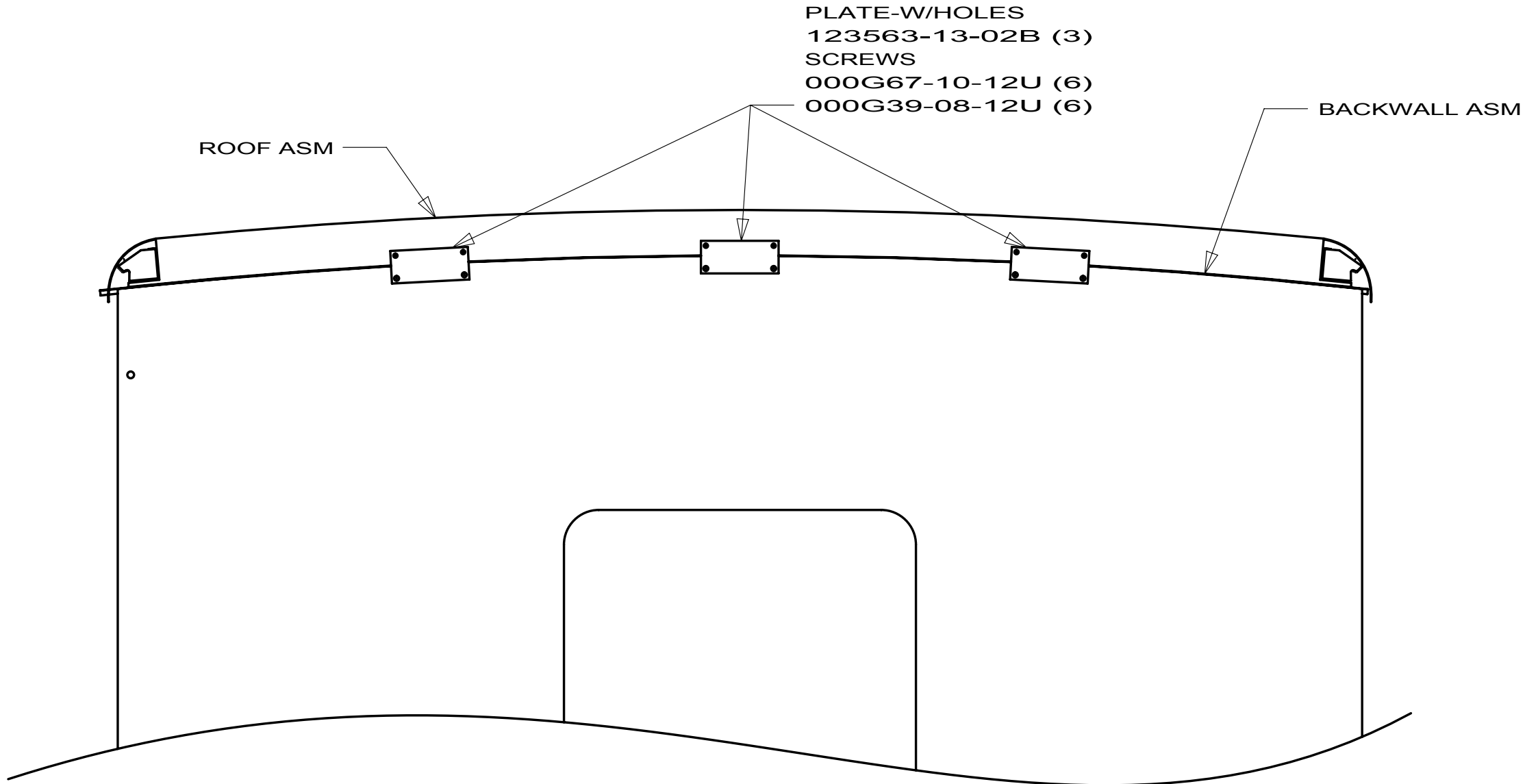
VIEW AB-AB
