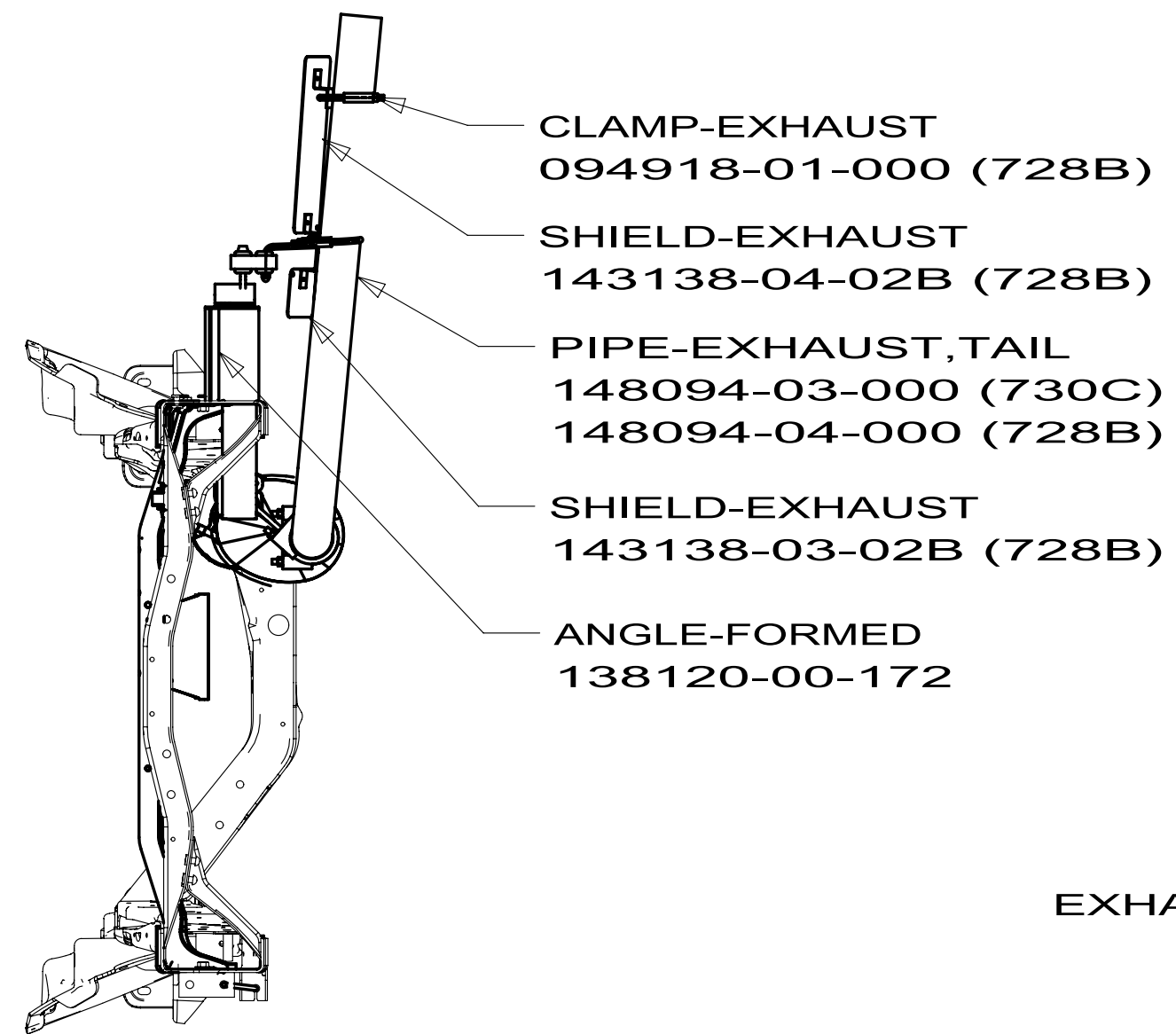
SECTION C-C (728B, 730C)
