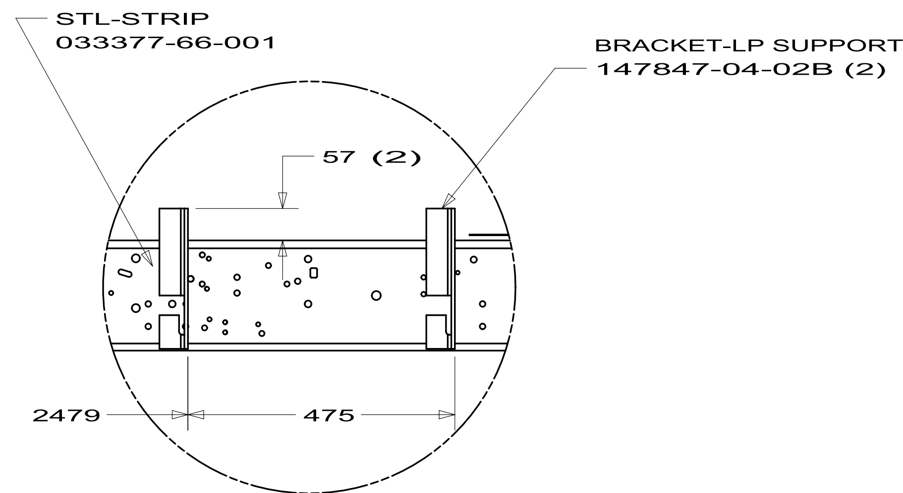
DETAIL BC
