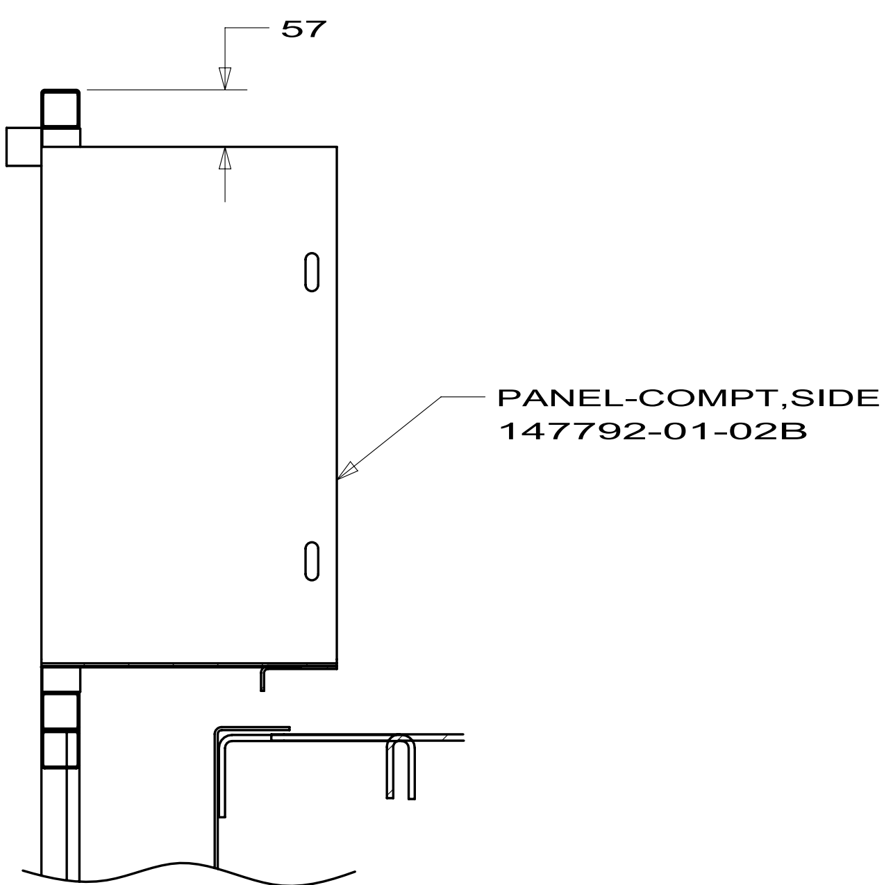
SECTION HA-HA
