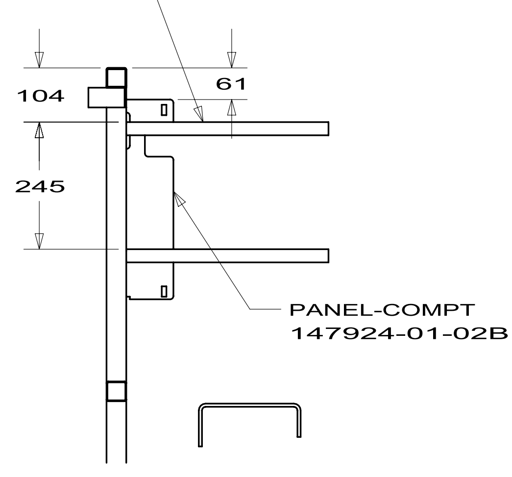
SECTION EE-EE
