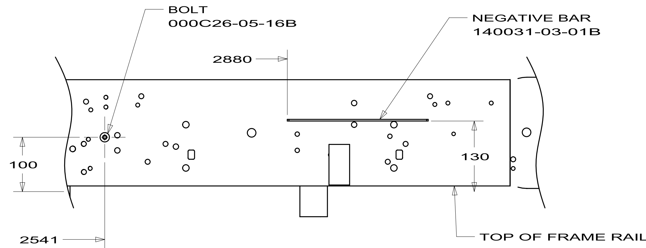
VIEW BD
