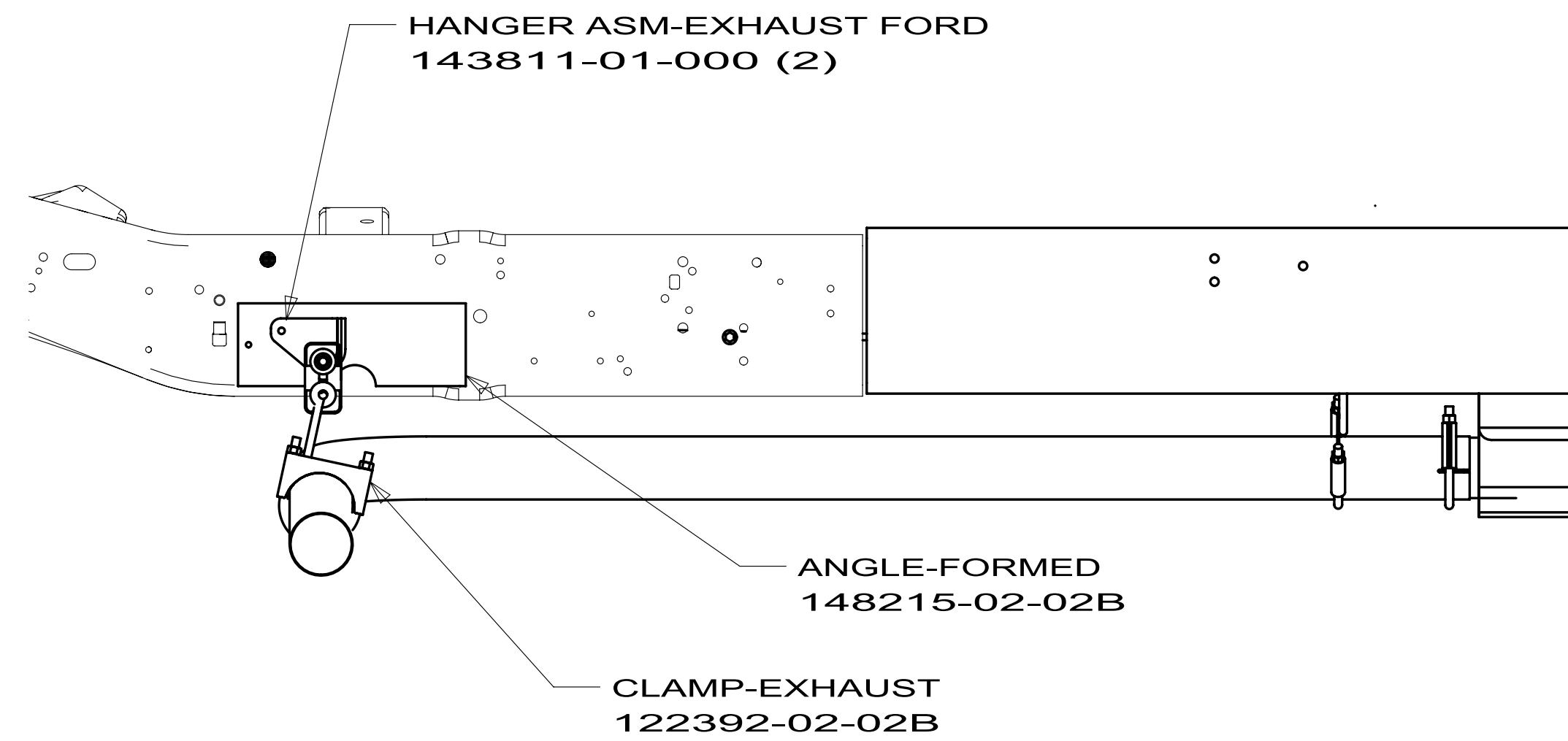
VIEW D
