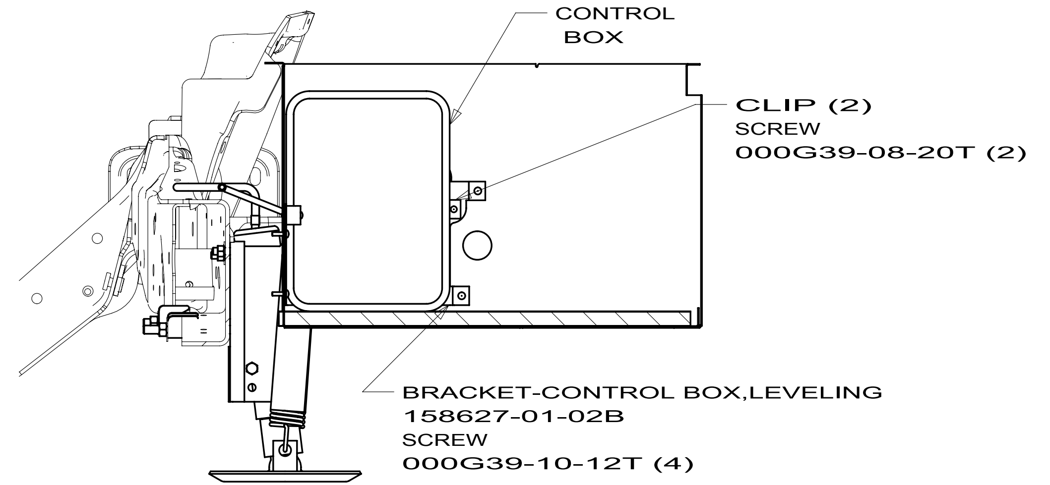
SECTION G-G
