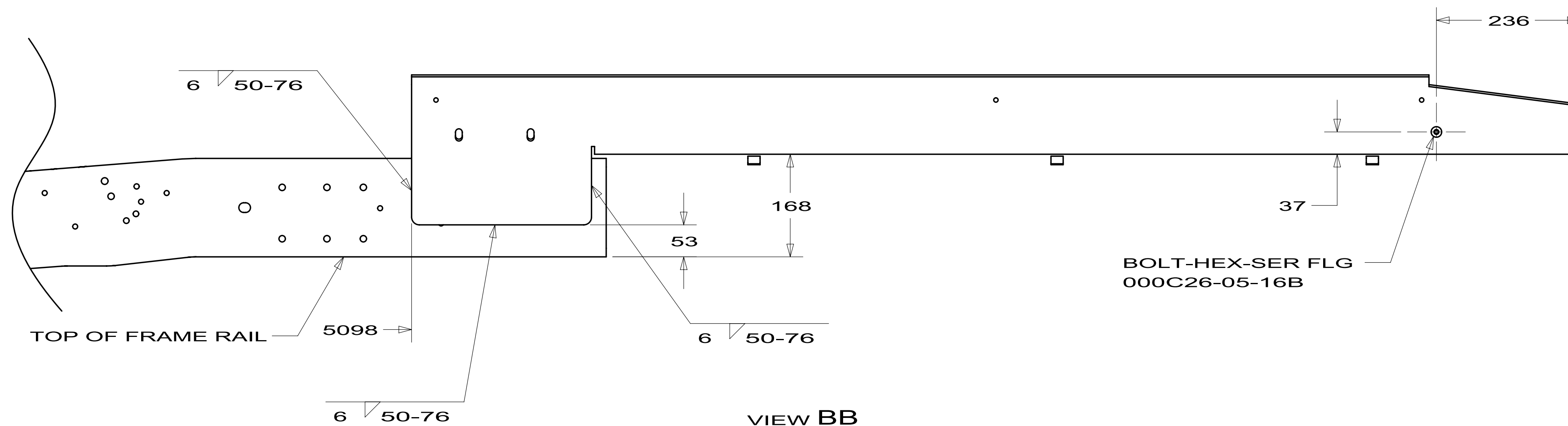
VIEW BB
