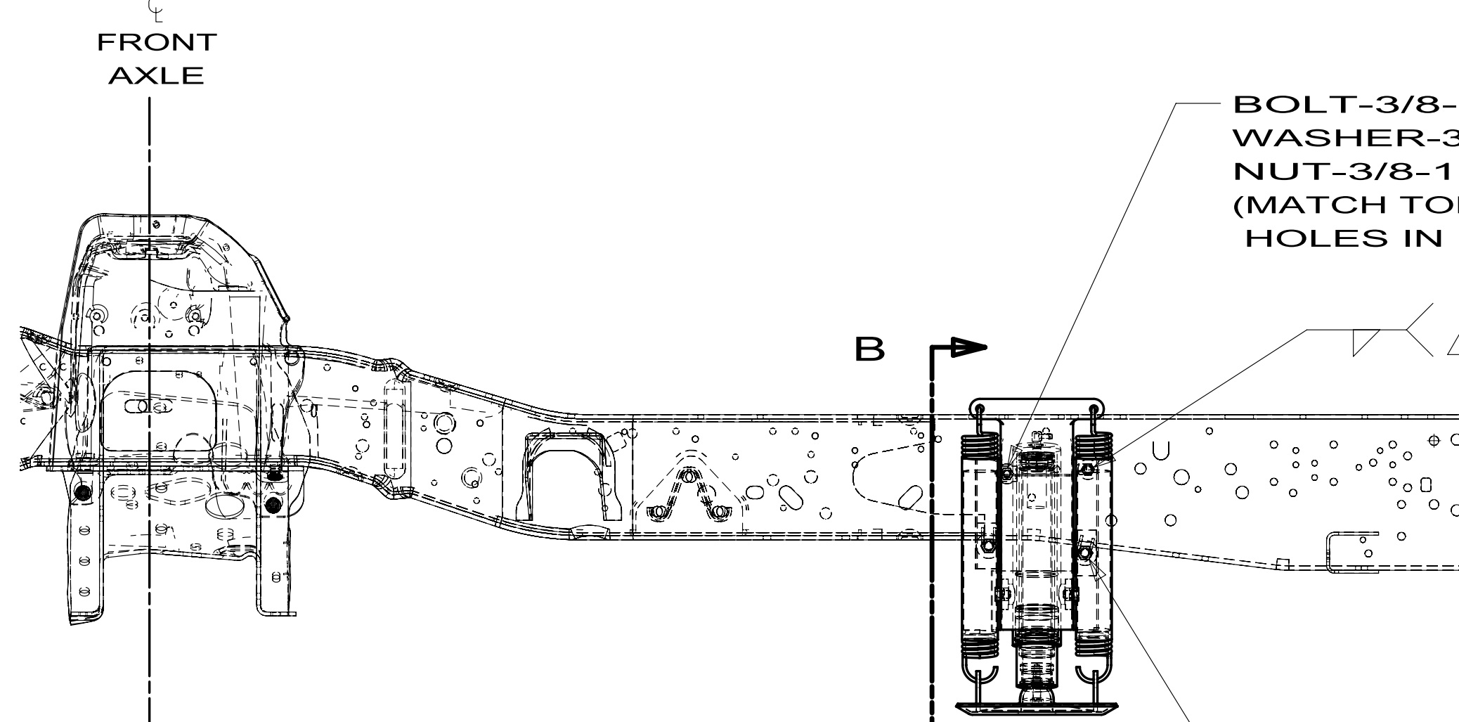
VIEW A FRONT JACKS
