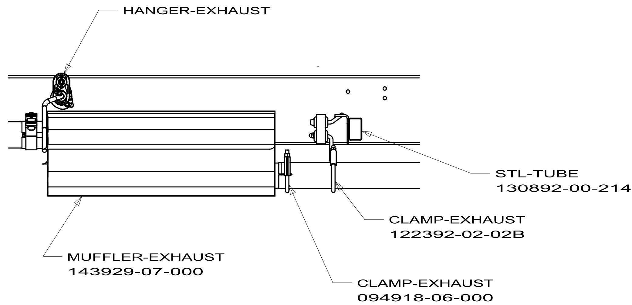
SECTION B-B
