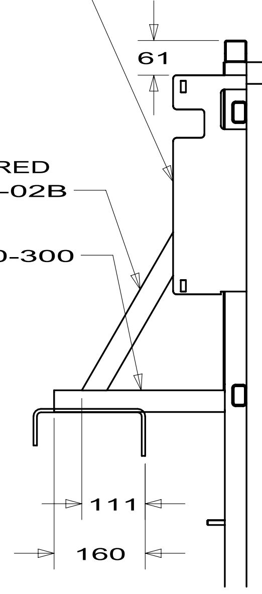
SECTION EL-EL
