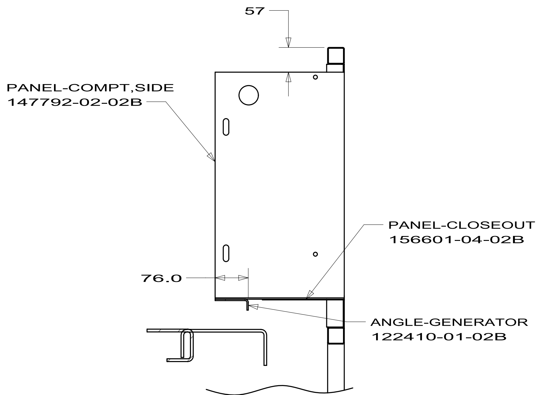
SECTION HB-HB
