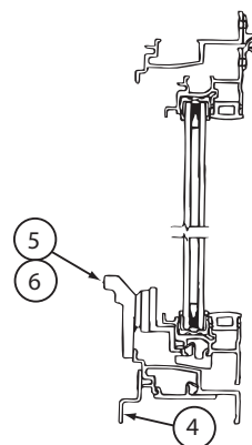
CROSS SECTION A-A
