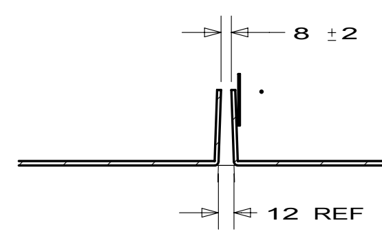
SECTION A-A (TYPICAL)
