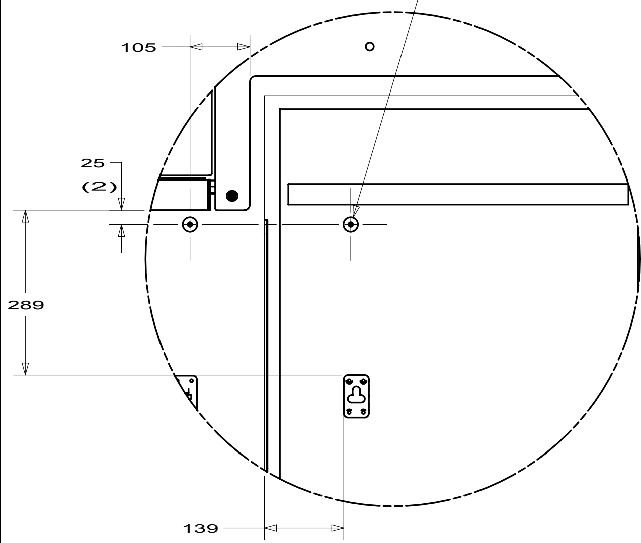
DETAIL B
