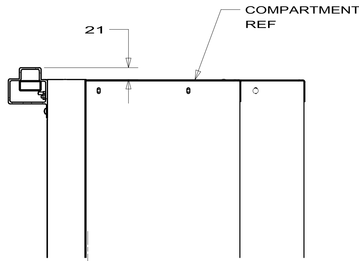
SECTION FJ-FJ (2 PLACES)
