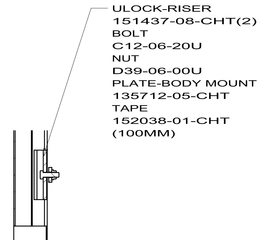
SECTION FF-FF (6 PLACES)
