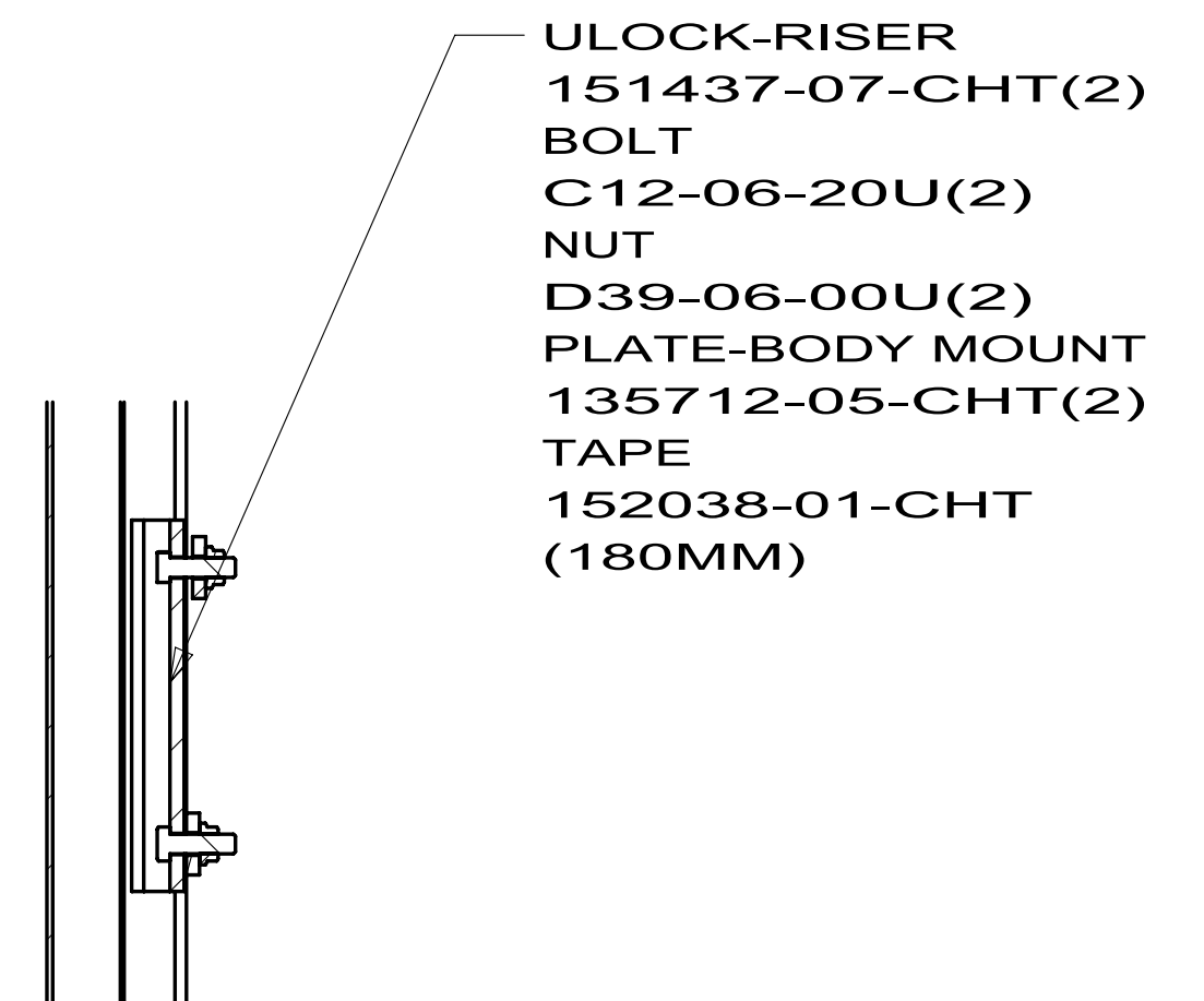
SECTION FG-FG (2 PLACES)
