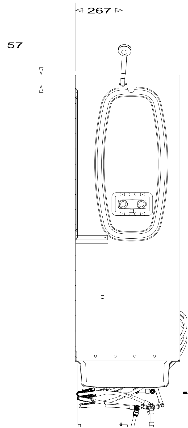
SECTION K-K
