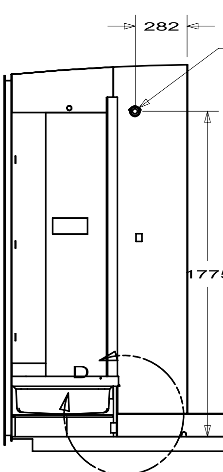
VIEW B
