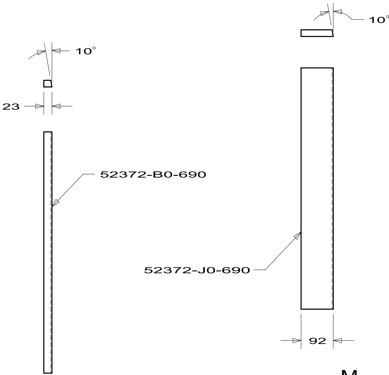
DETAIL M LUMBER 152053-25
