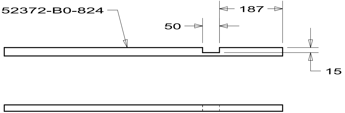
DETAIL B LUMBER 169998-17
