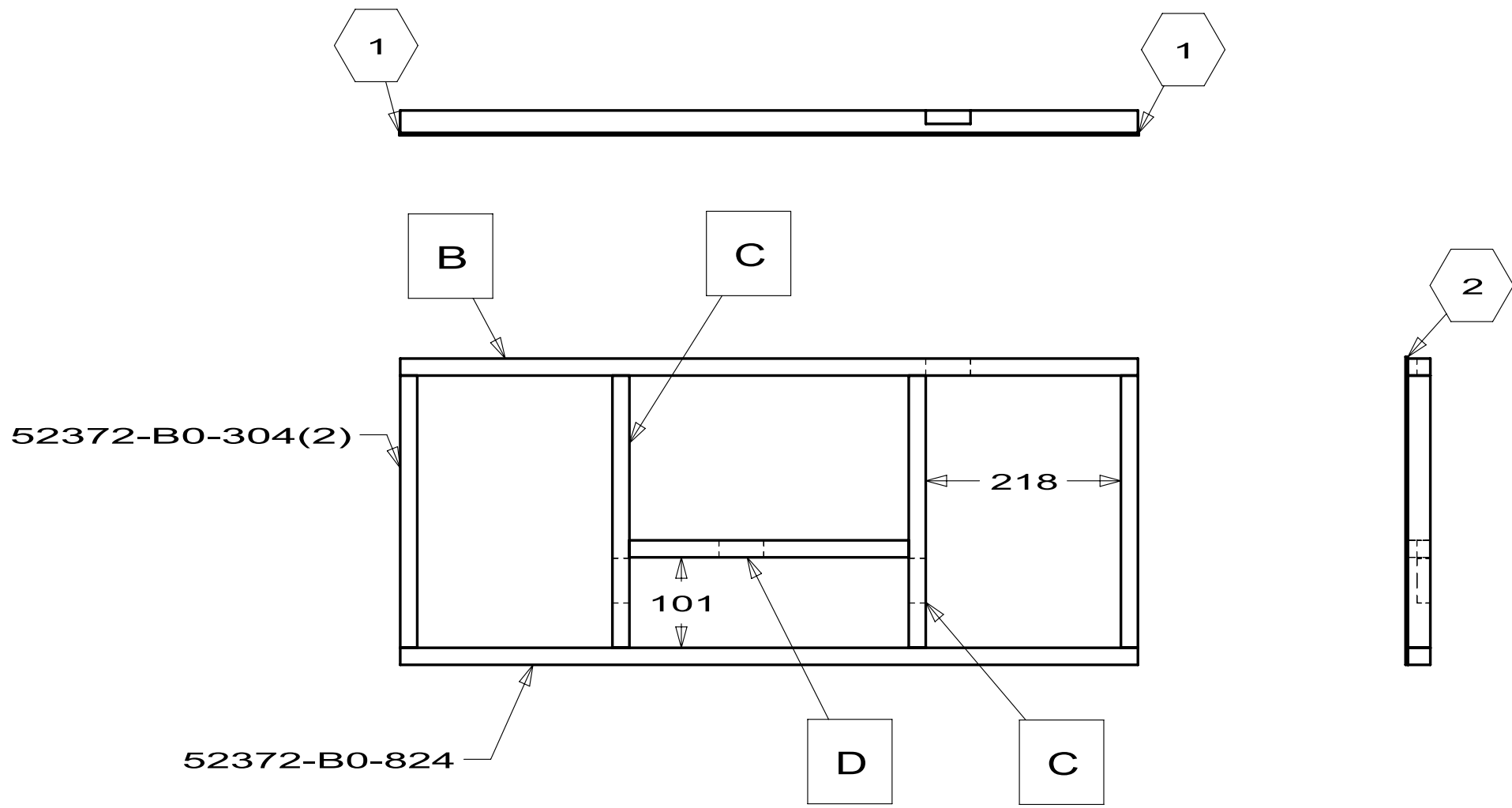
DETAIL A PANEL ASM 169998-11
