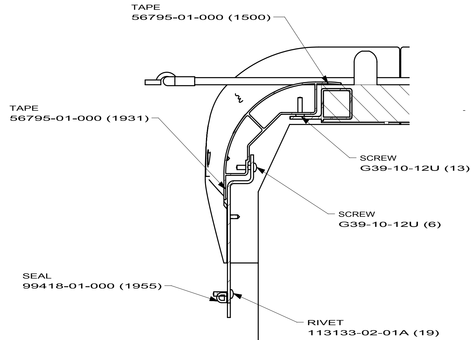
SECTION AF-AF
