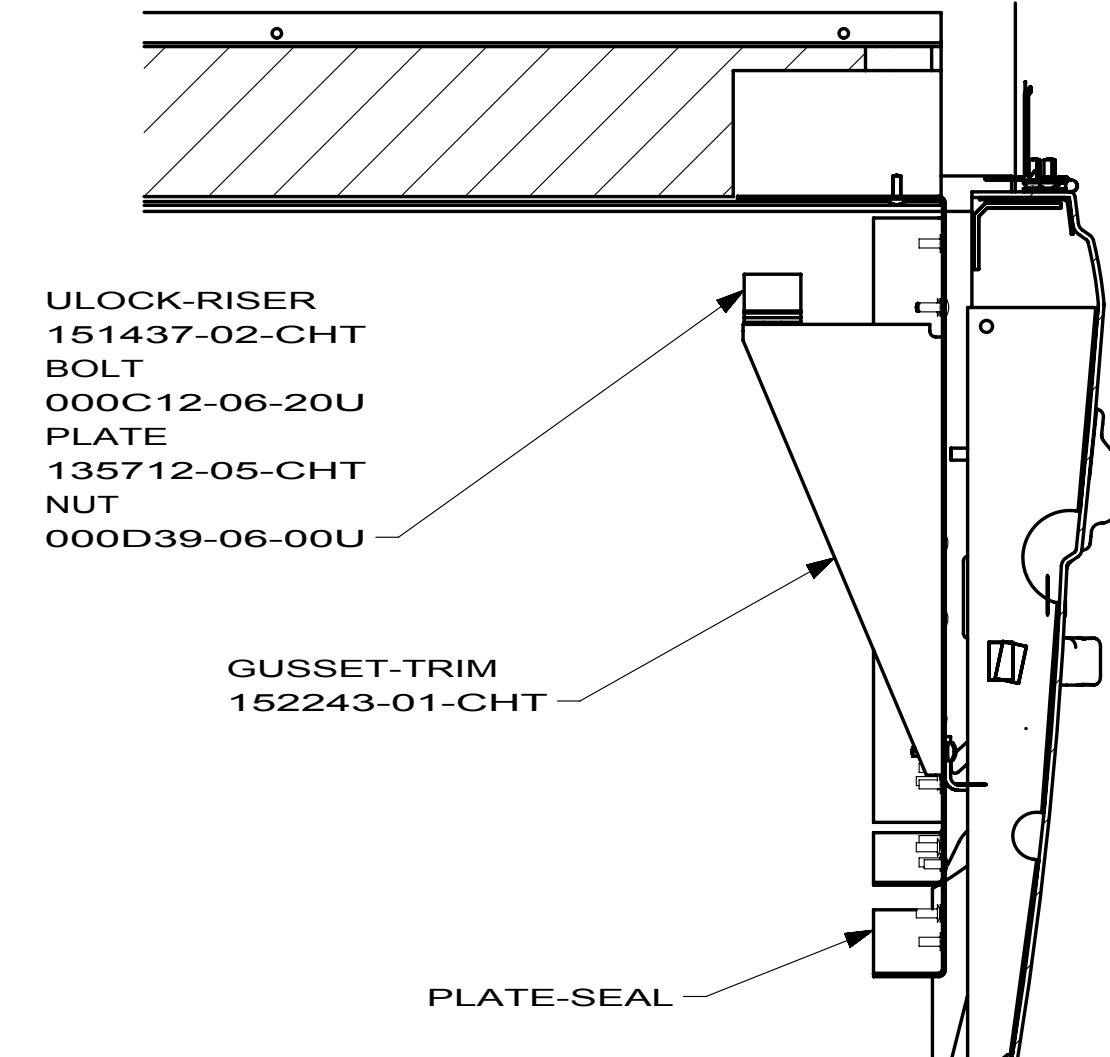
SECTION BJ-BJ
