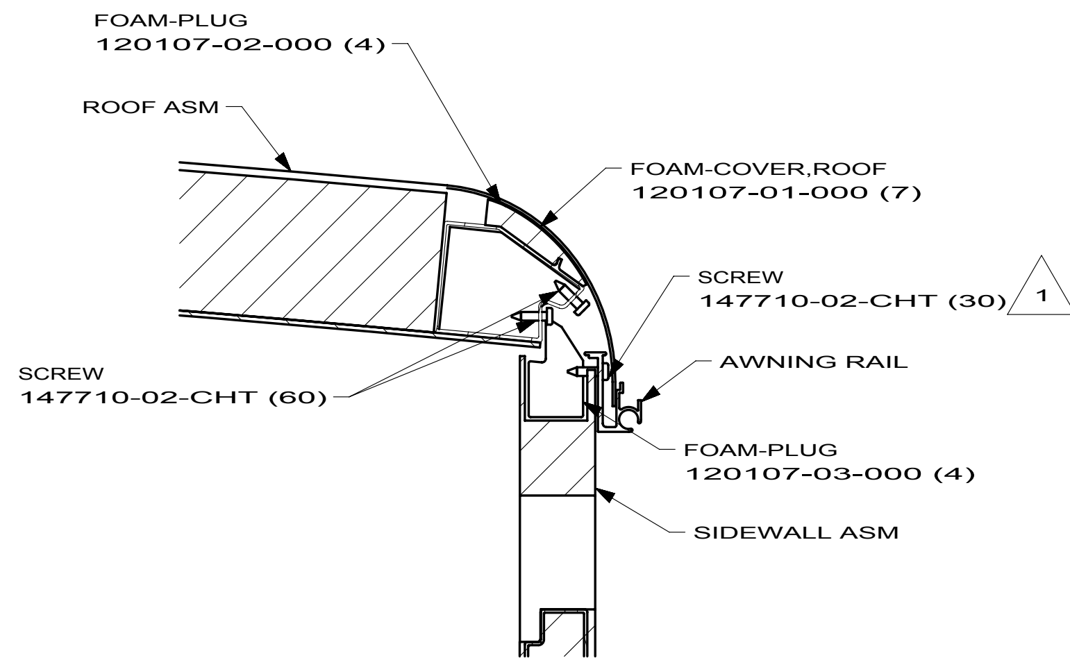
SECTION AC-AC
