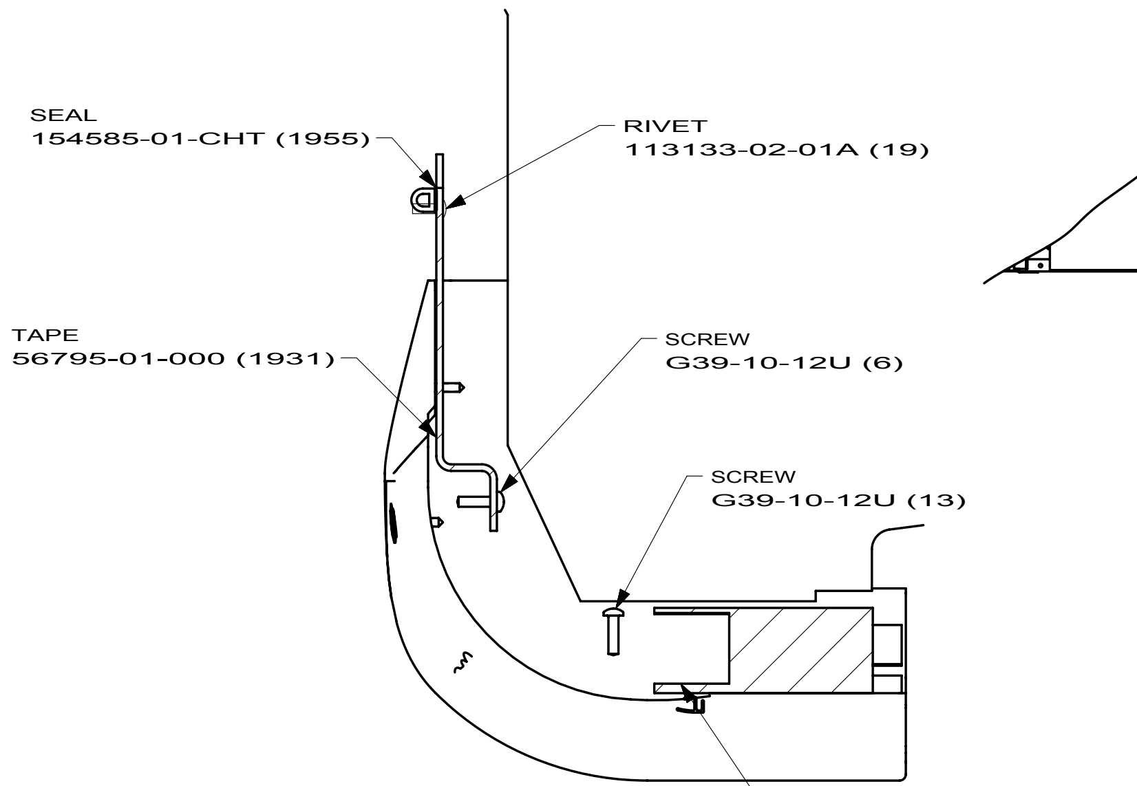
SECTION AD-AD
