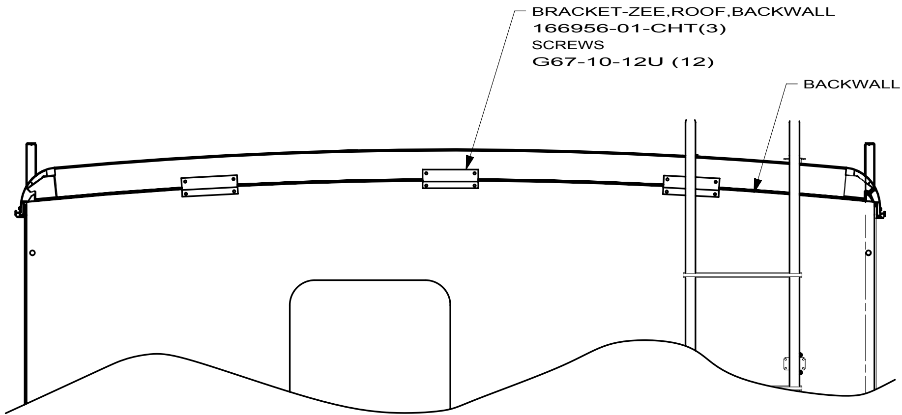
VIEW AB-AB
