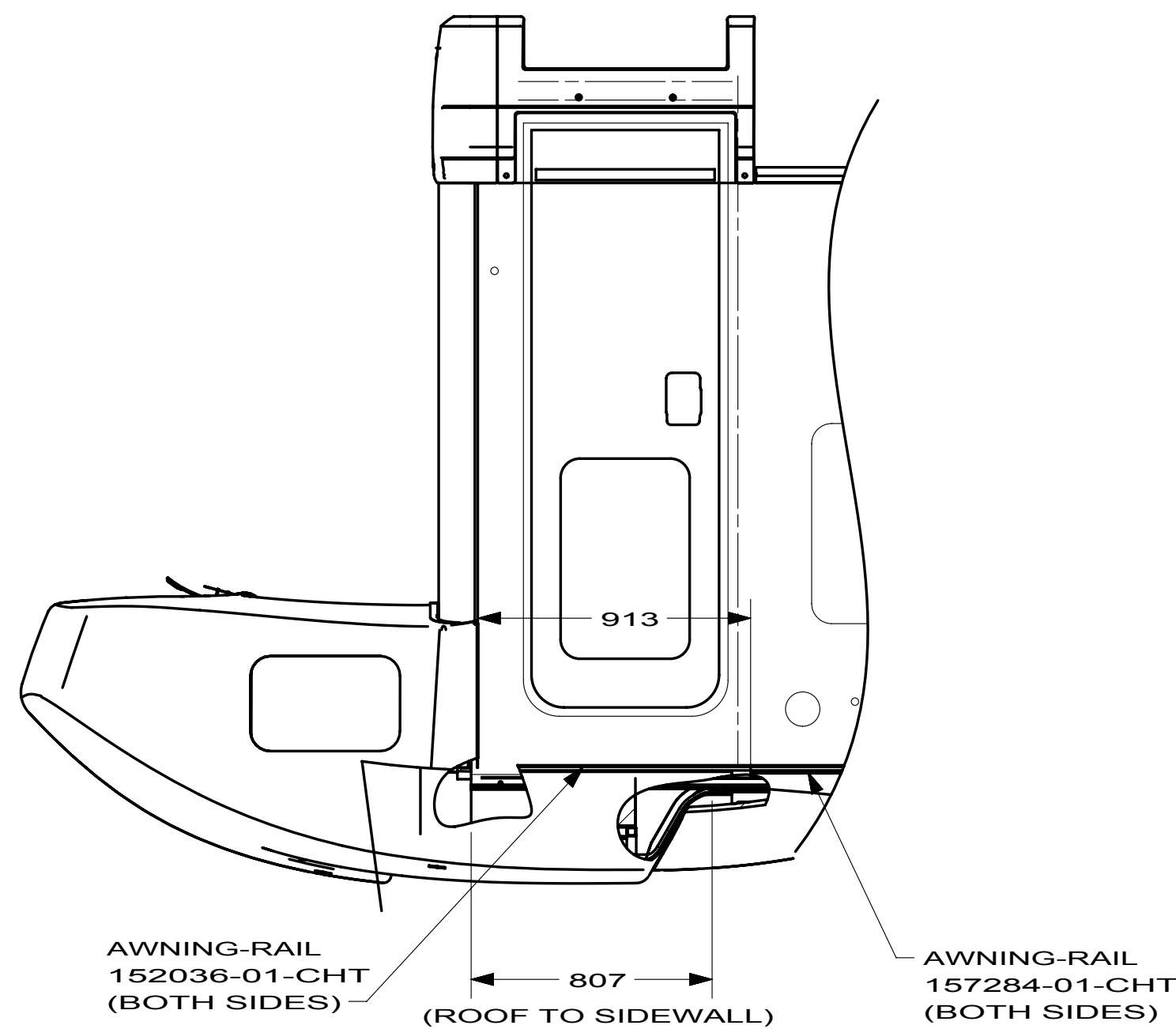
DETAIL AG
