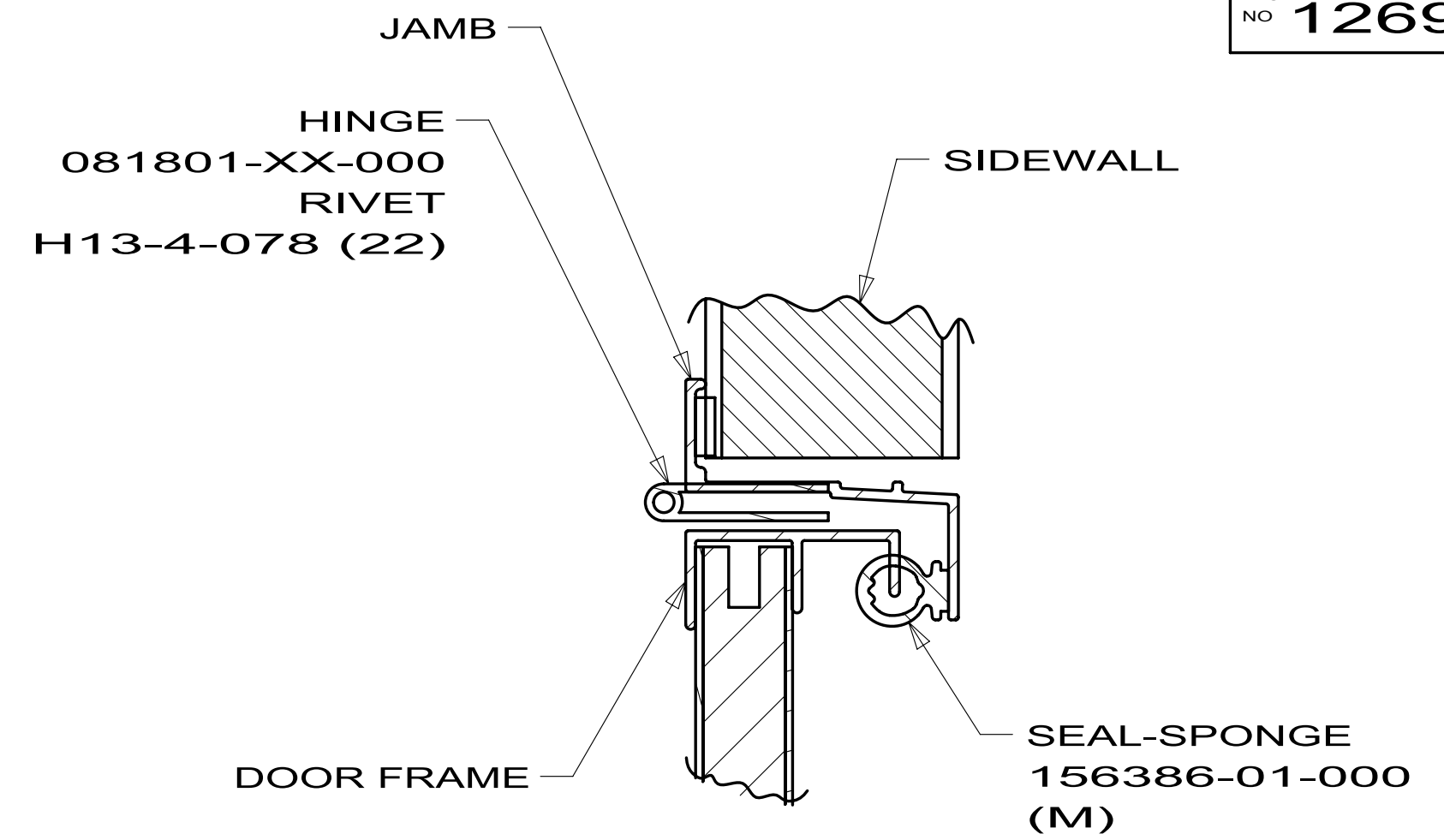
DETAIL Z
