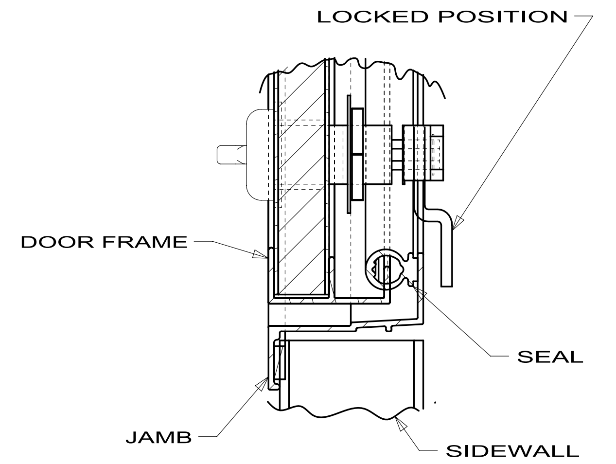
DETAIL F
