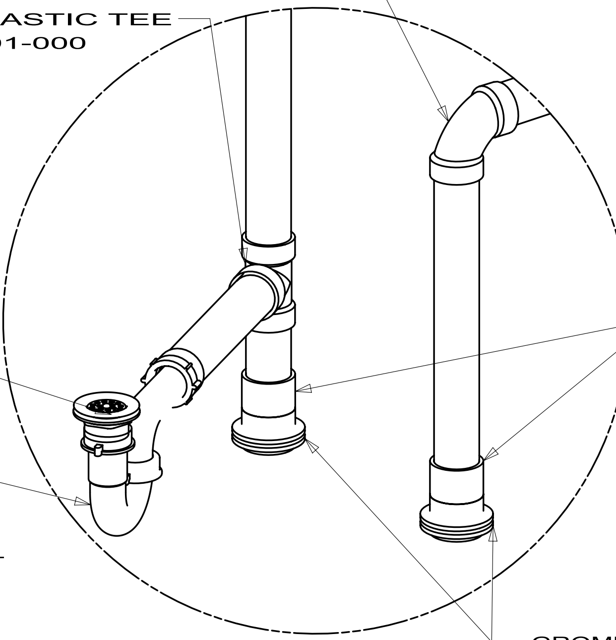
DETAIL D (SHOWN W/OUT CABINETS AND FLOOR)
