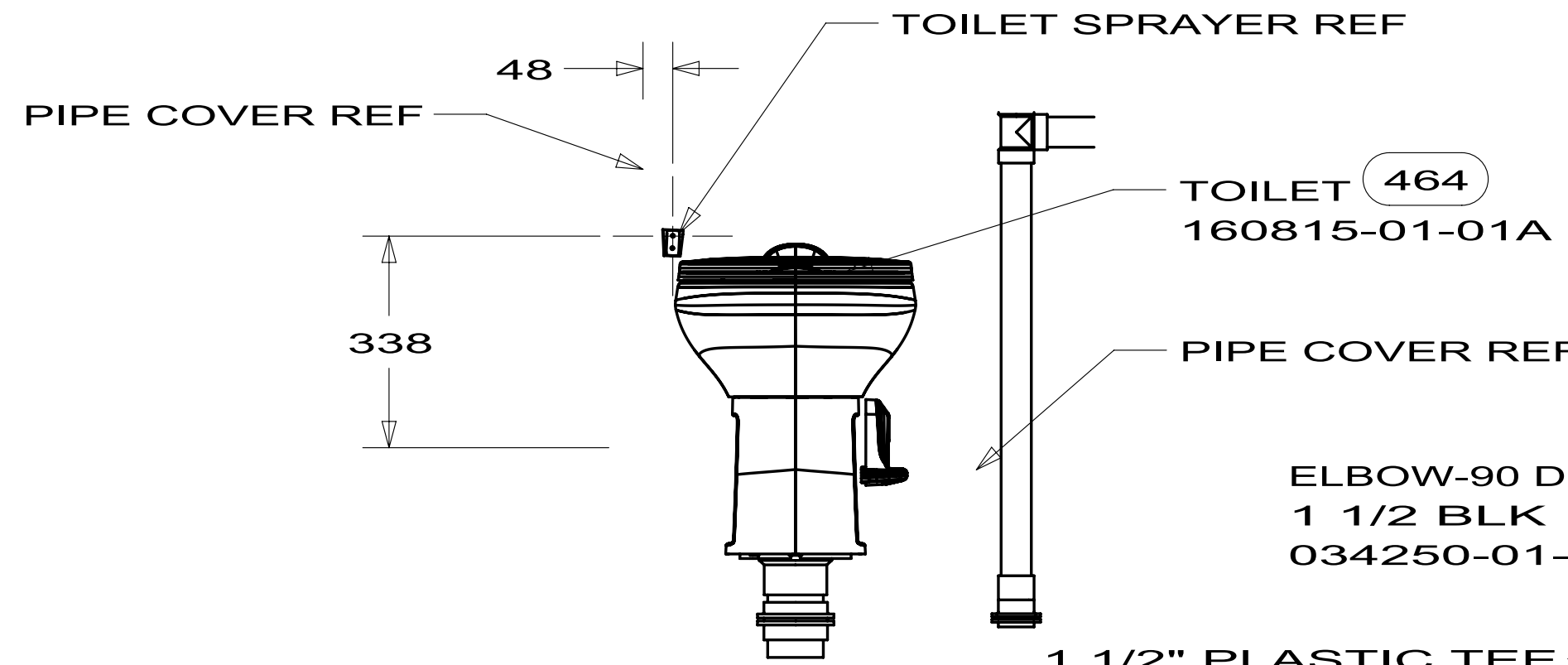
SECTION F-F
