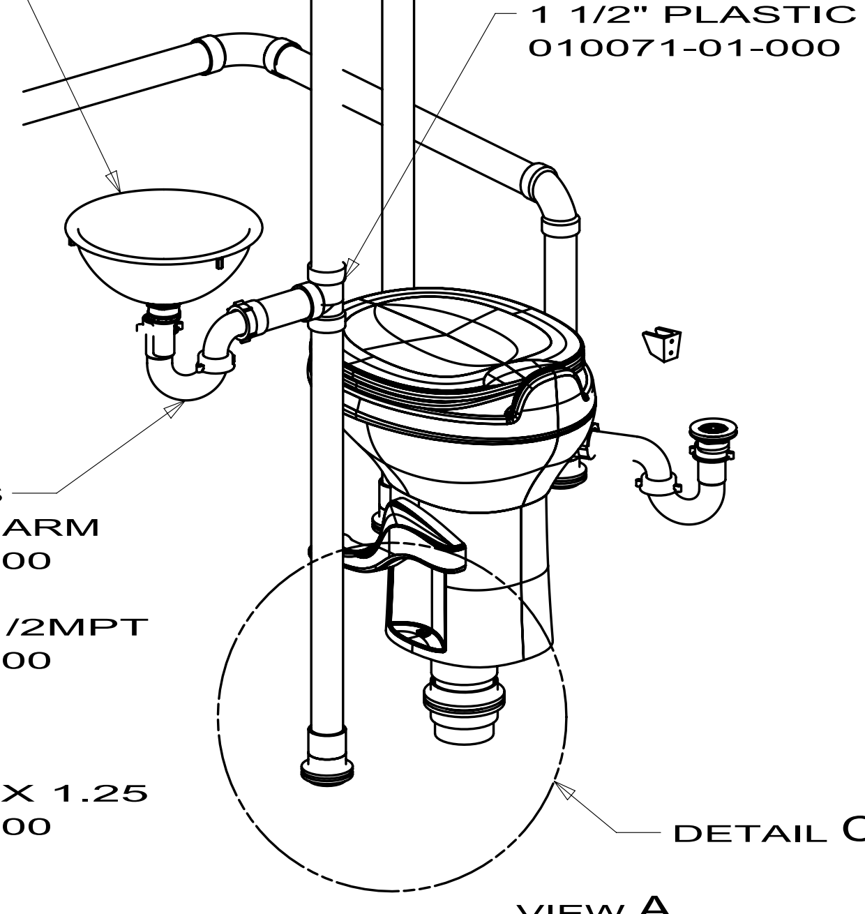
VIEW A
