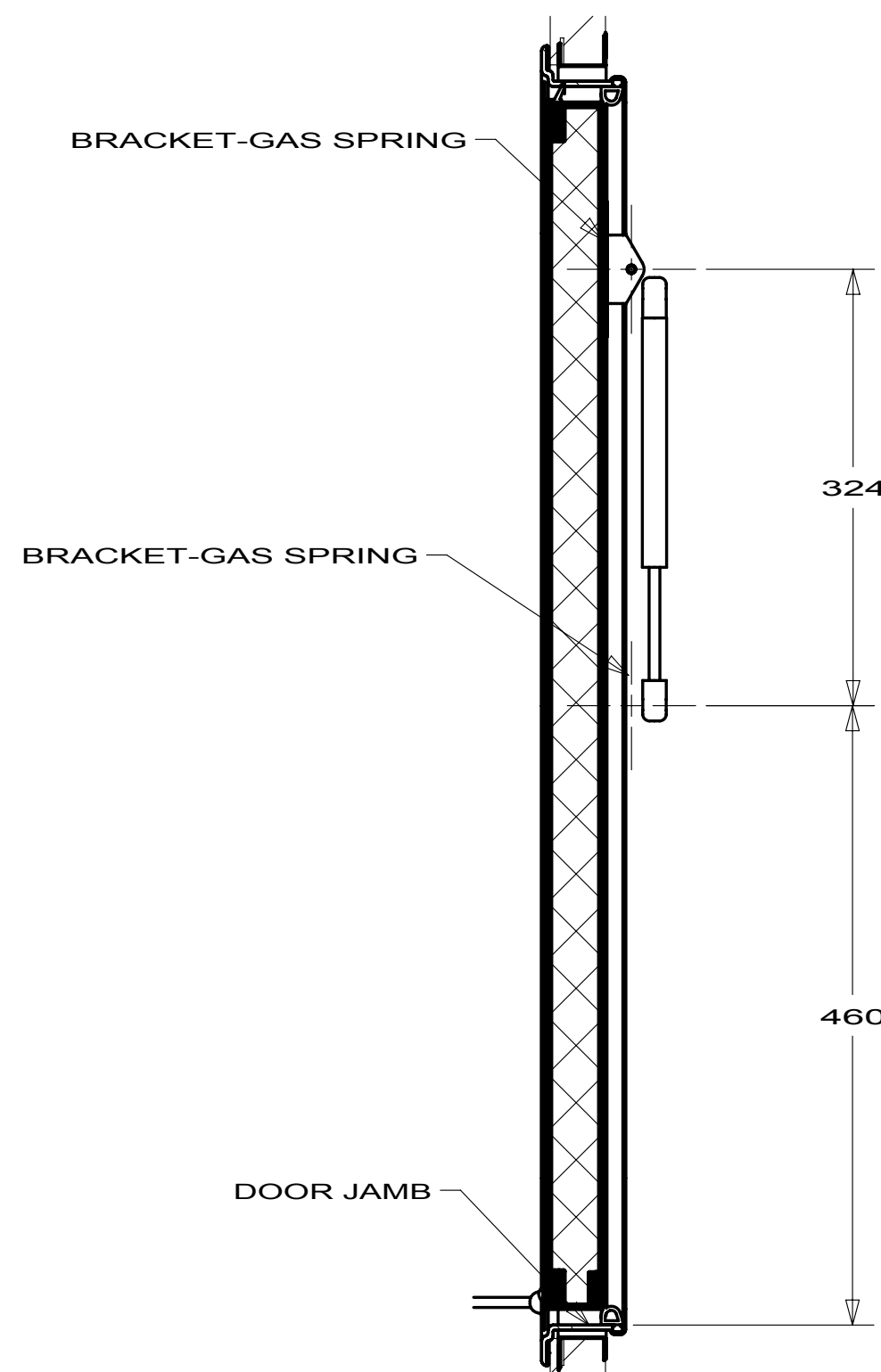
SECTION BD-BD
