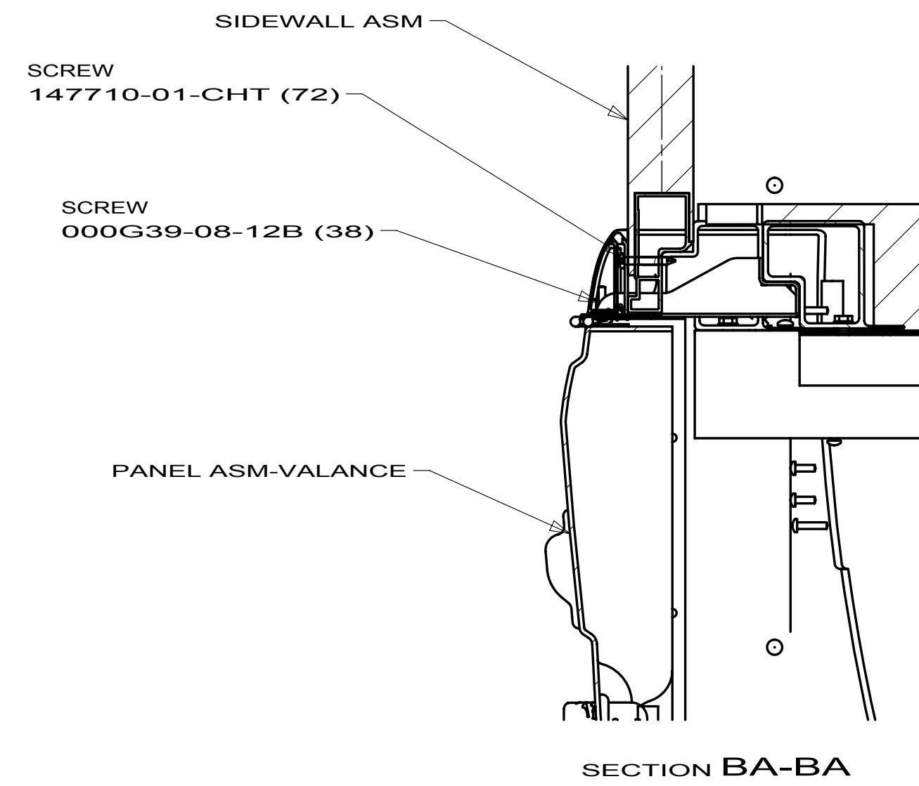
SECTION BA-BA
