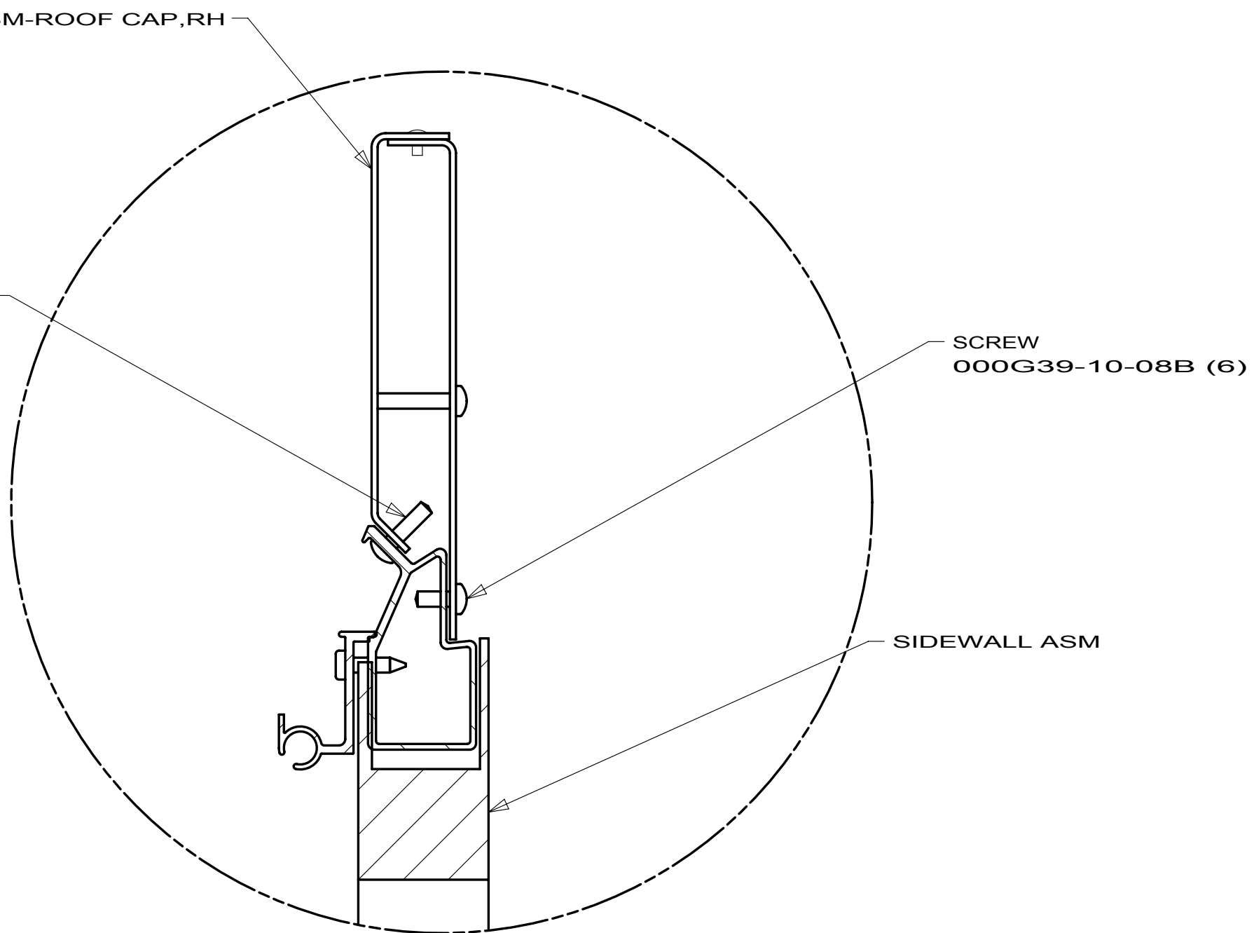
DETAIL AJ (RH SHOWN) (LH SIMILAR)
