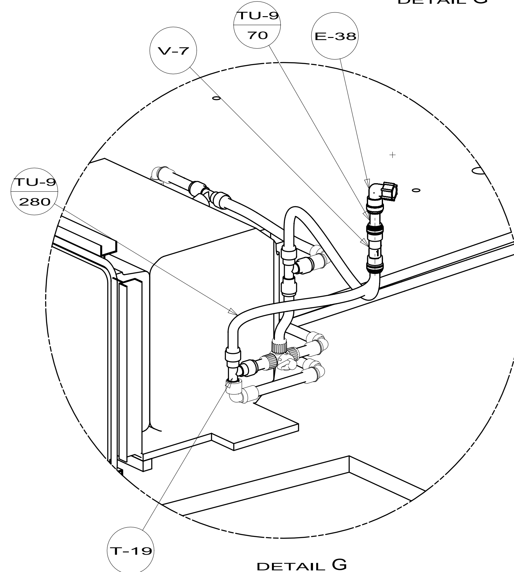
DETAIL G
