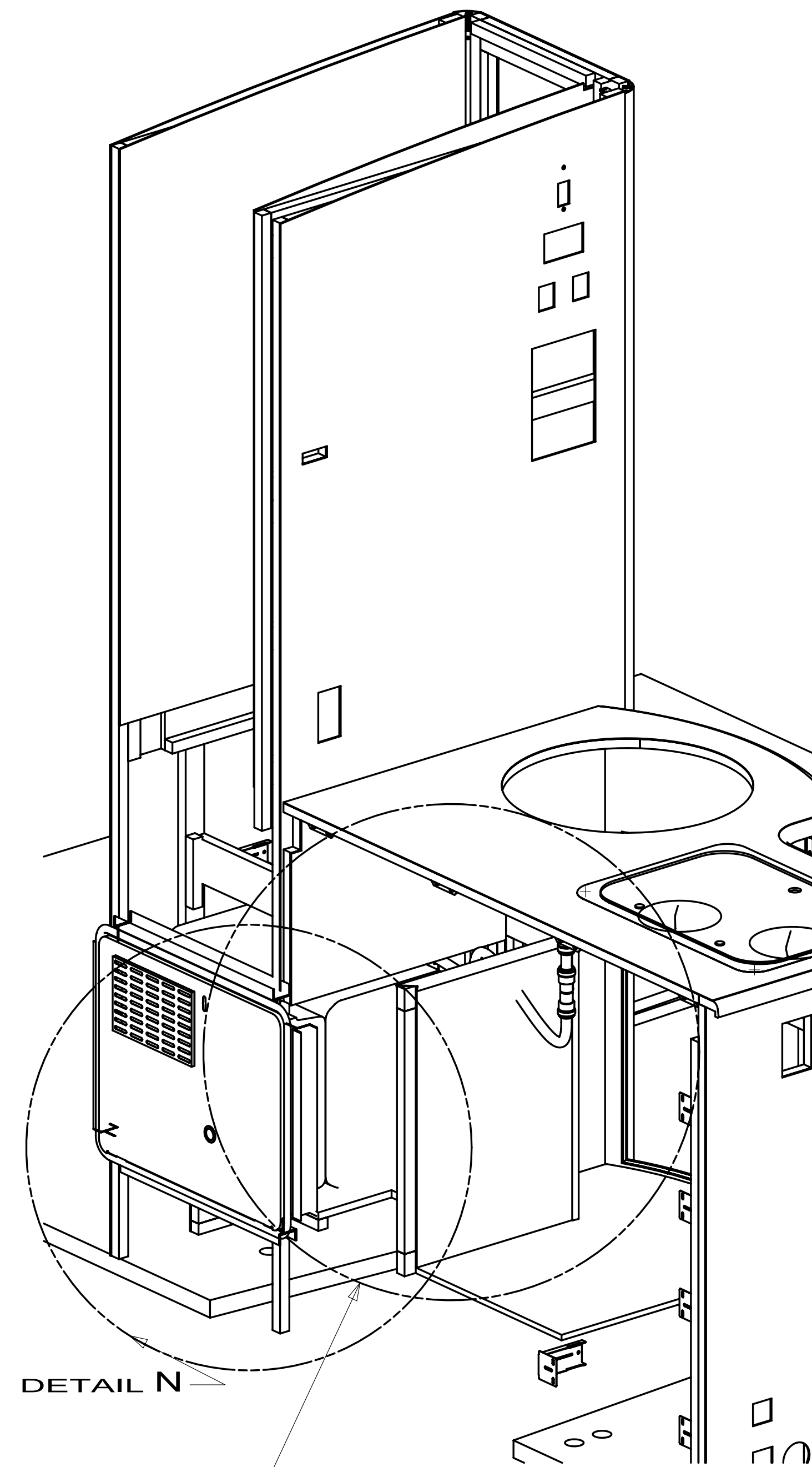
VIEW F
