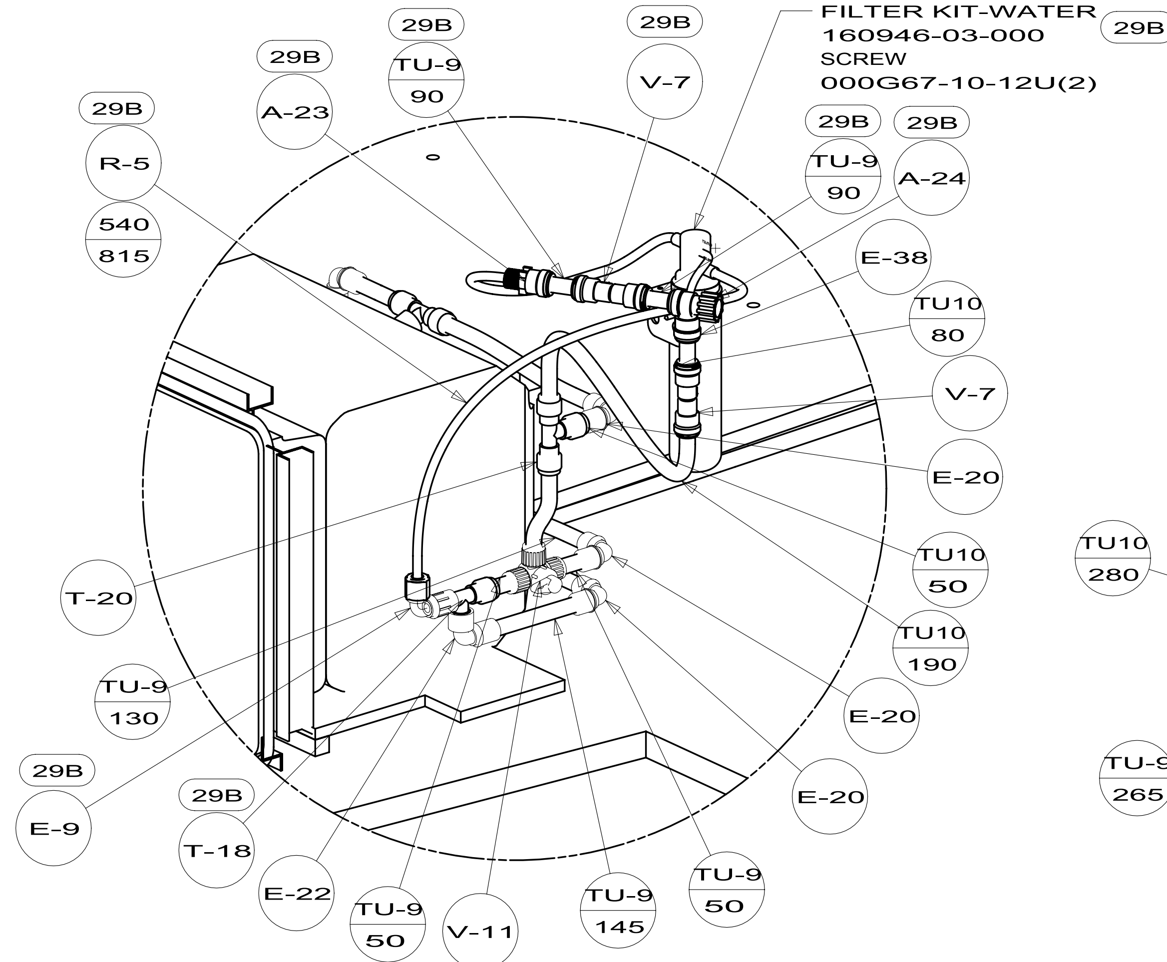
DETAIL G
