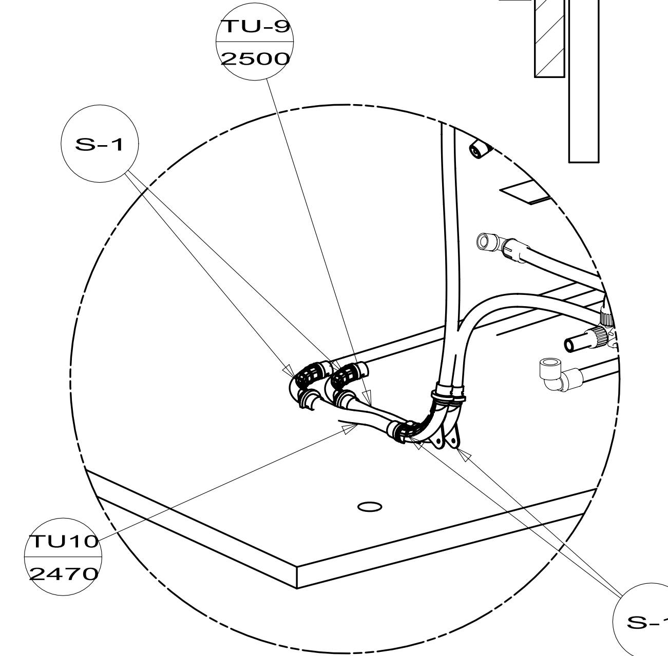
DETAIL N (SHOWN W/OUT WATER HEATER AND CABINETS)
