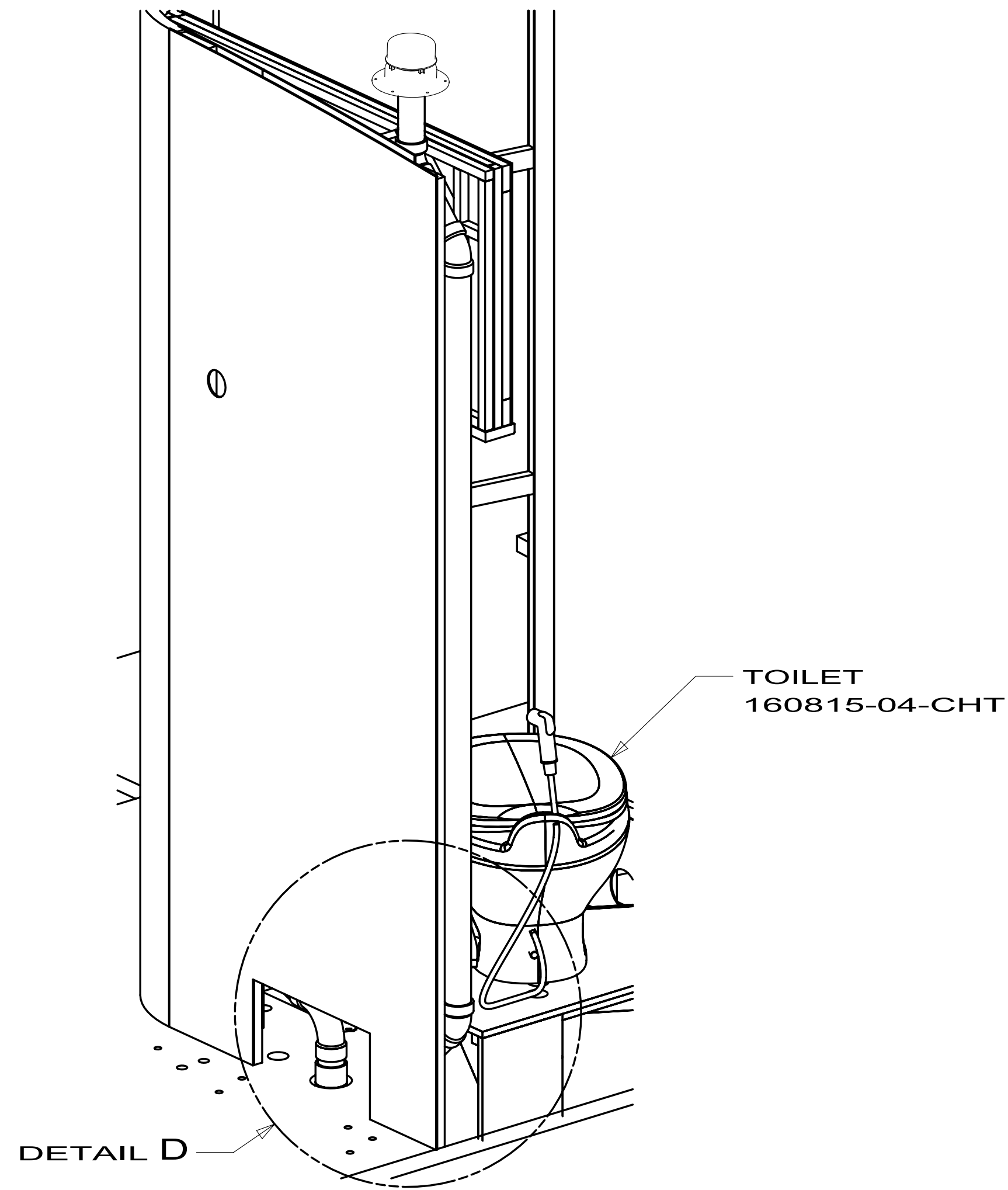
VIEW C
