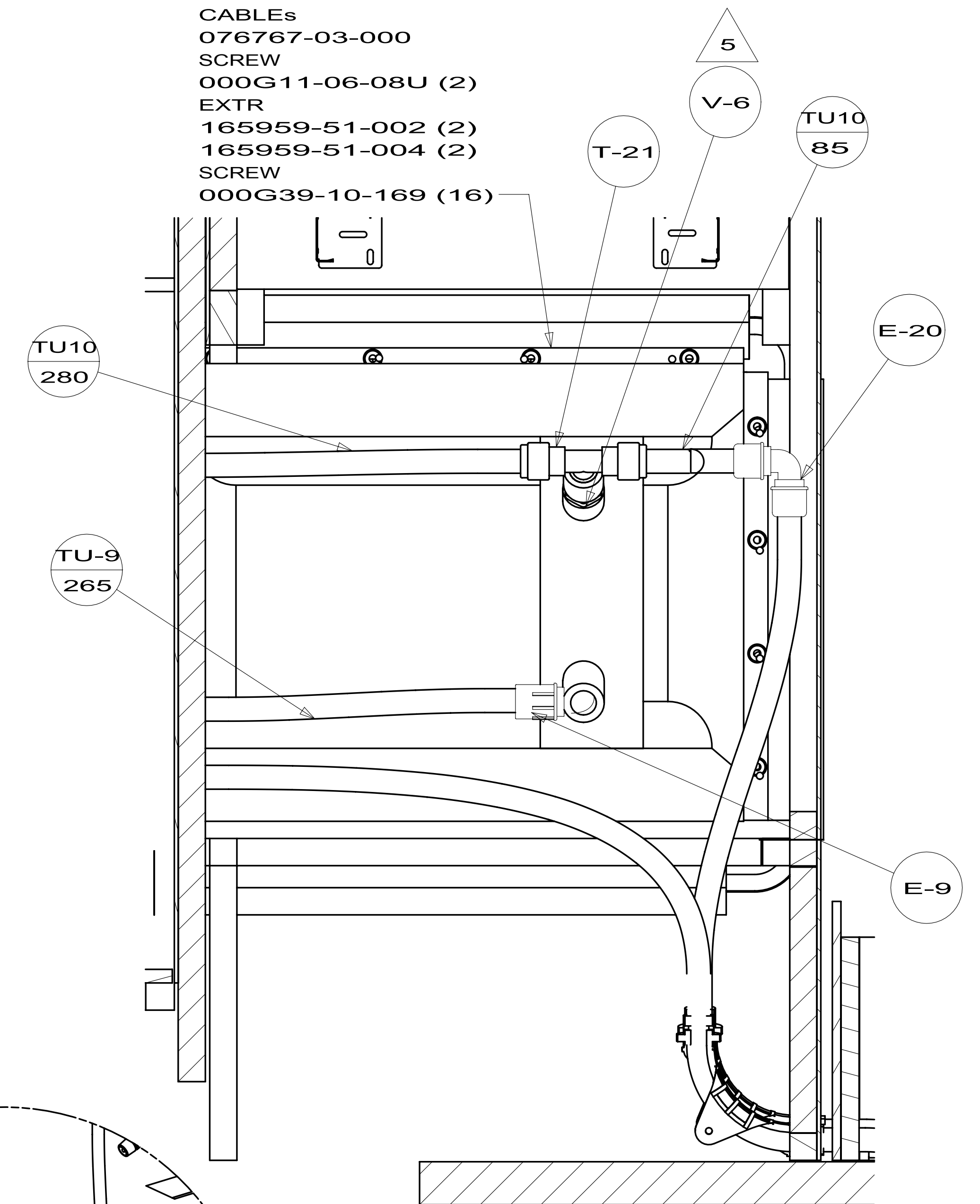
SECTION J-J
