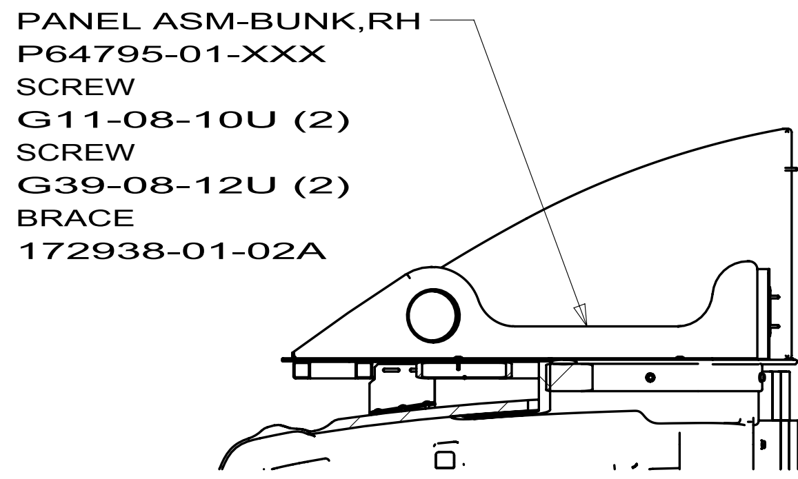
SECTION K-K
