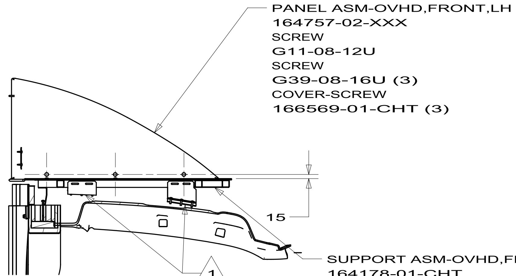
SECTION L-L
