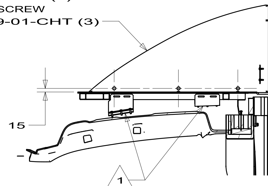
SECTION M-M
