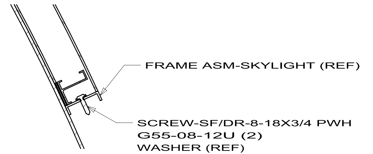
SECTION G-G
