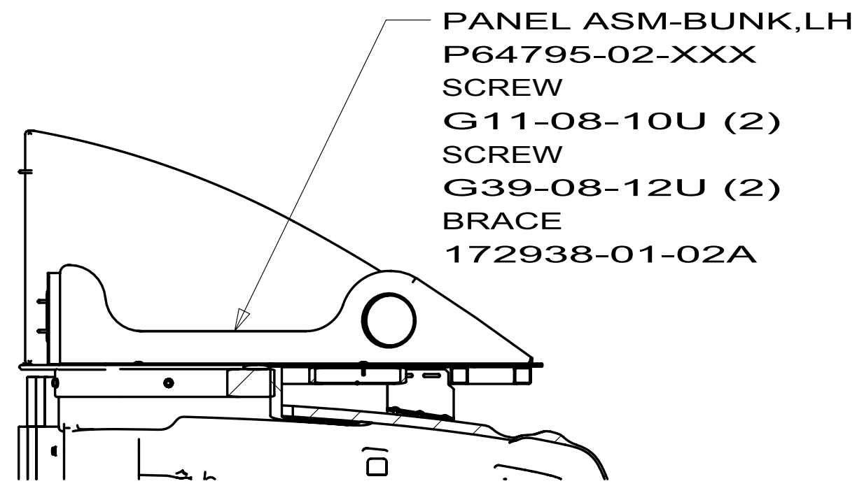
SECTION J-J
