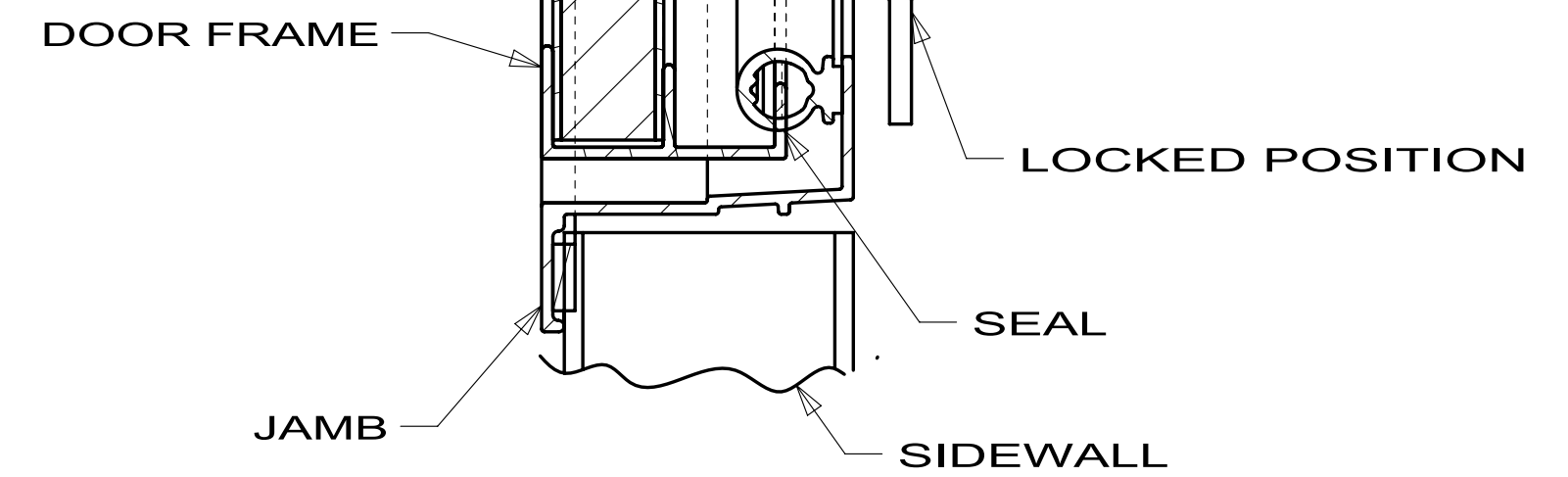
DETAIL V
