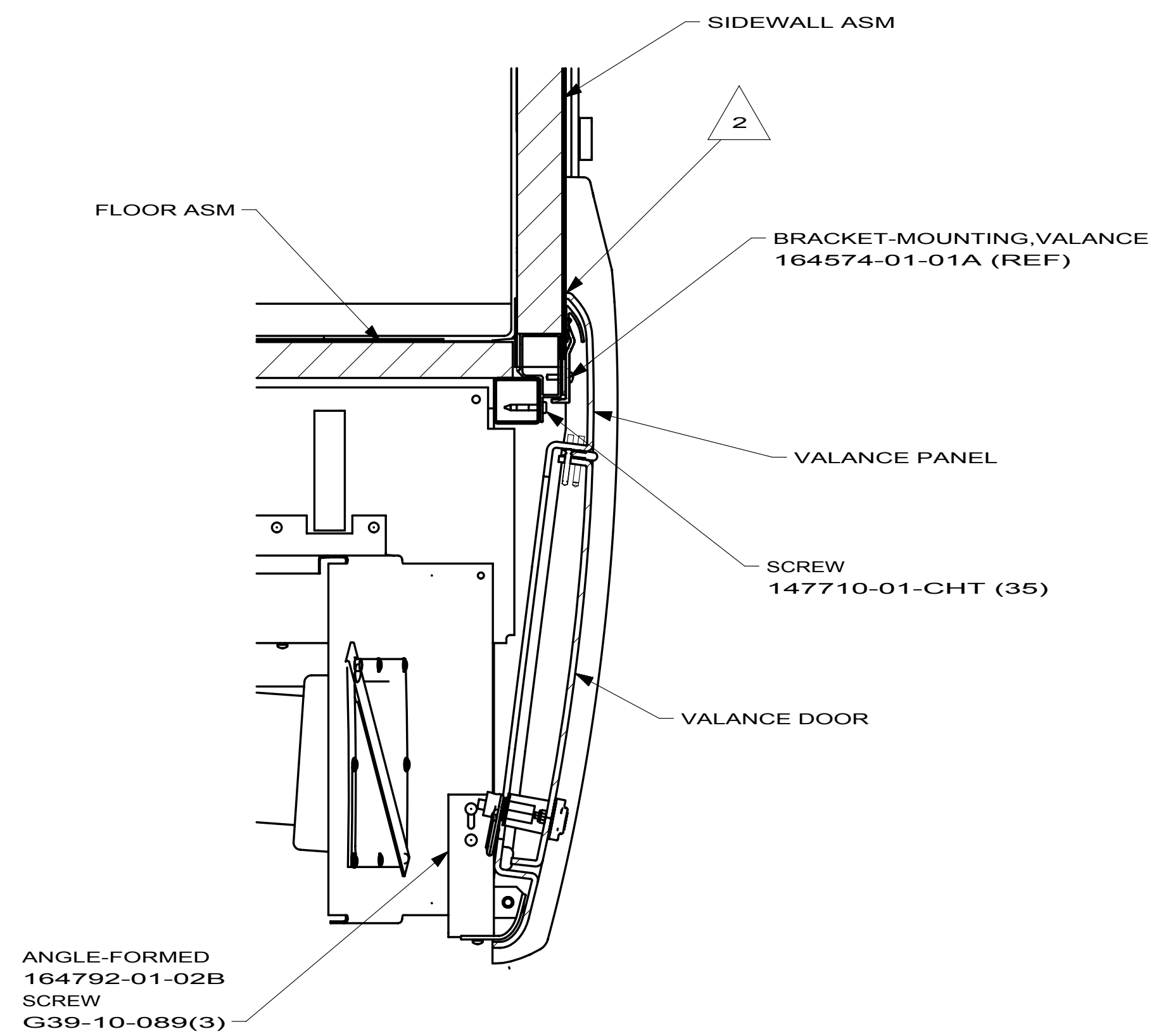
SECTION BE-BE
