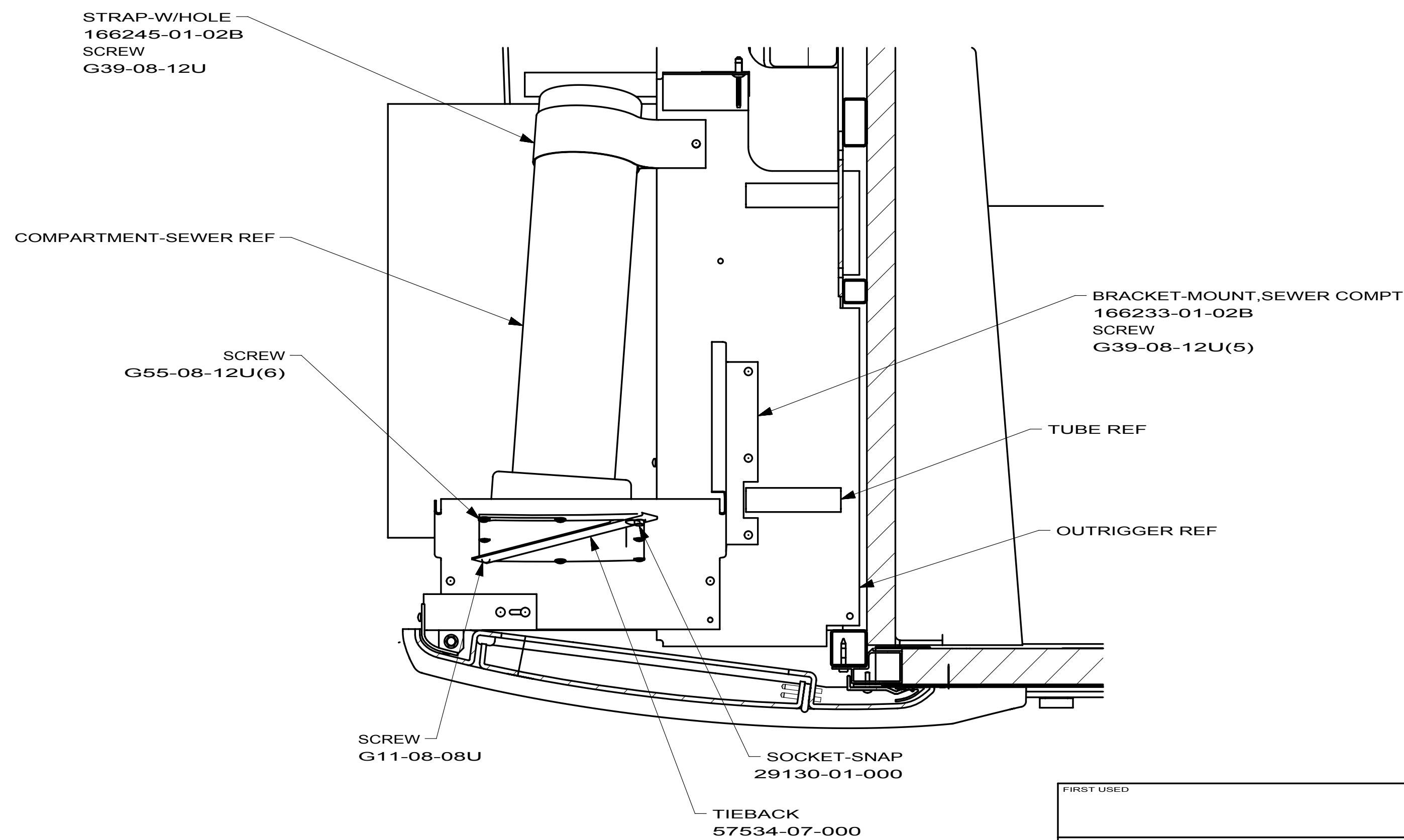
SECTION BM-BM
