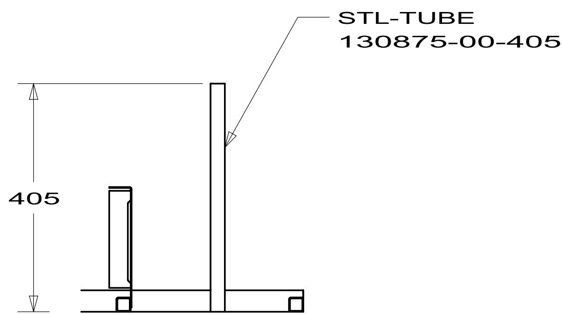
SECTION GH-GH
