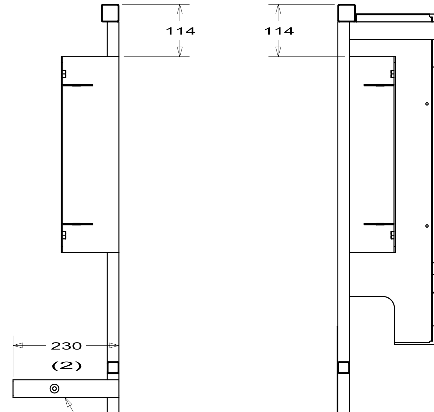
SECTION GD-GD
