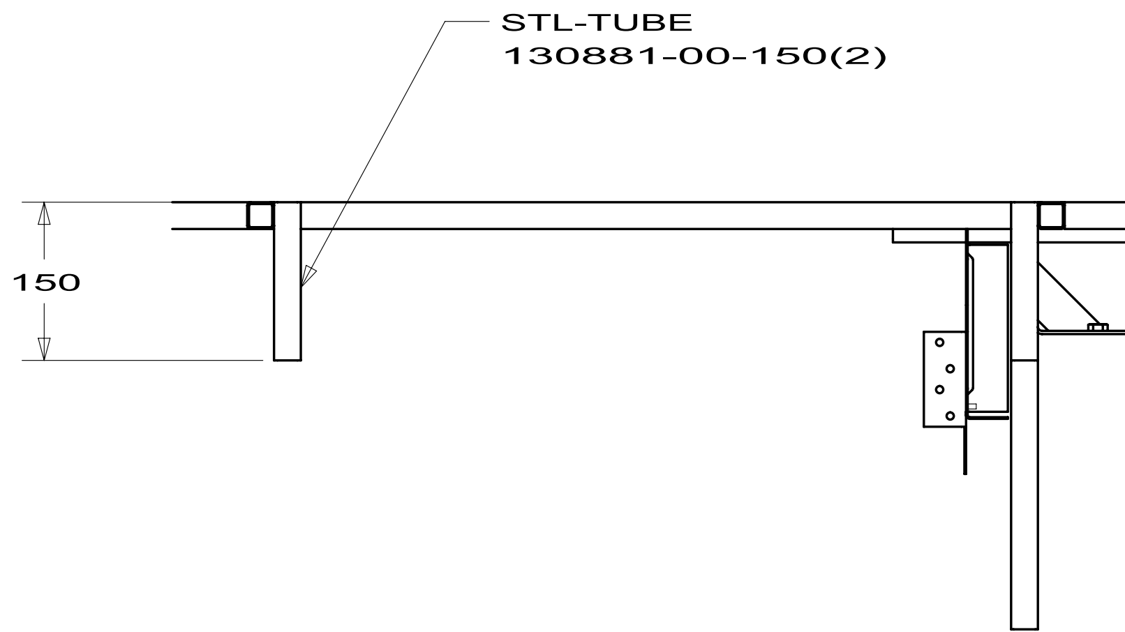
SECTION GF-GF
