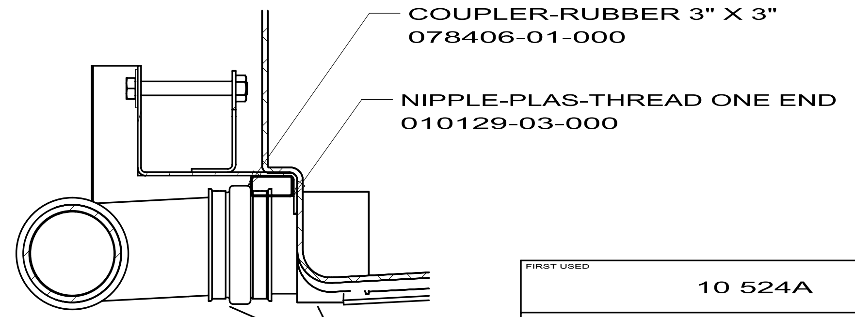
SECTION G-G
