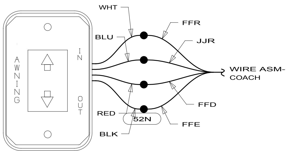
DETAIL EN (SUPPLIED WITH AWNING)
