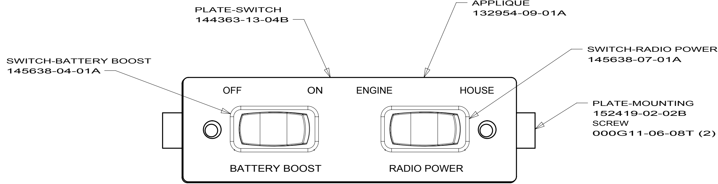
DETAIL CA
