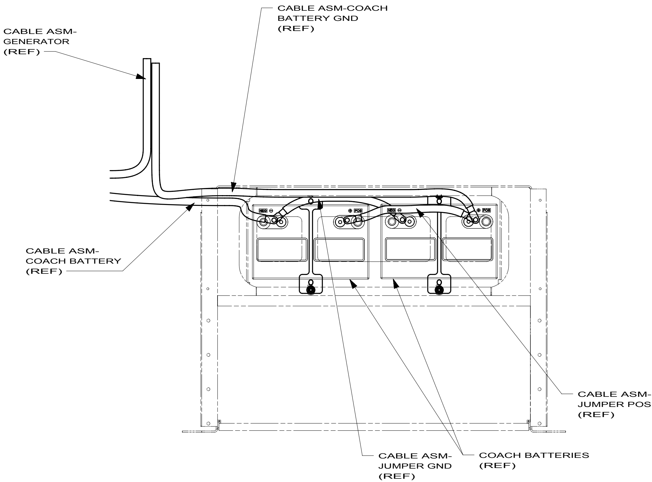
VIEW BA
