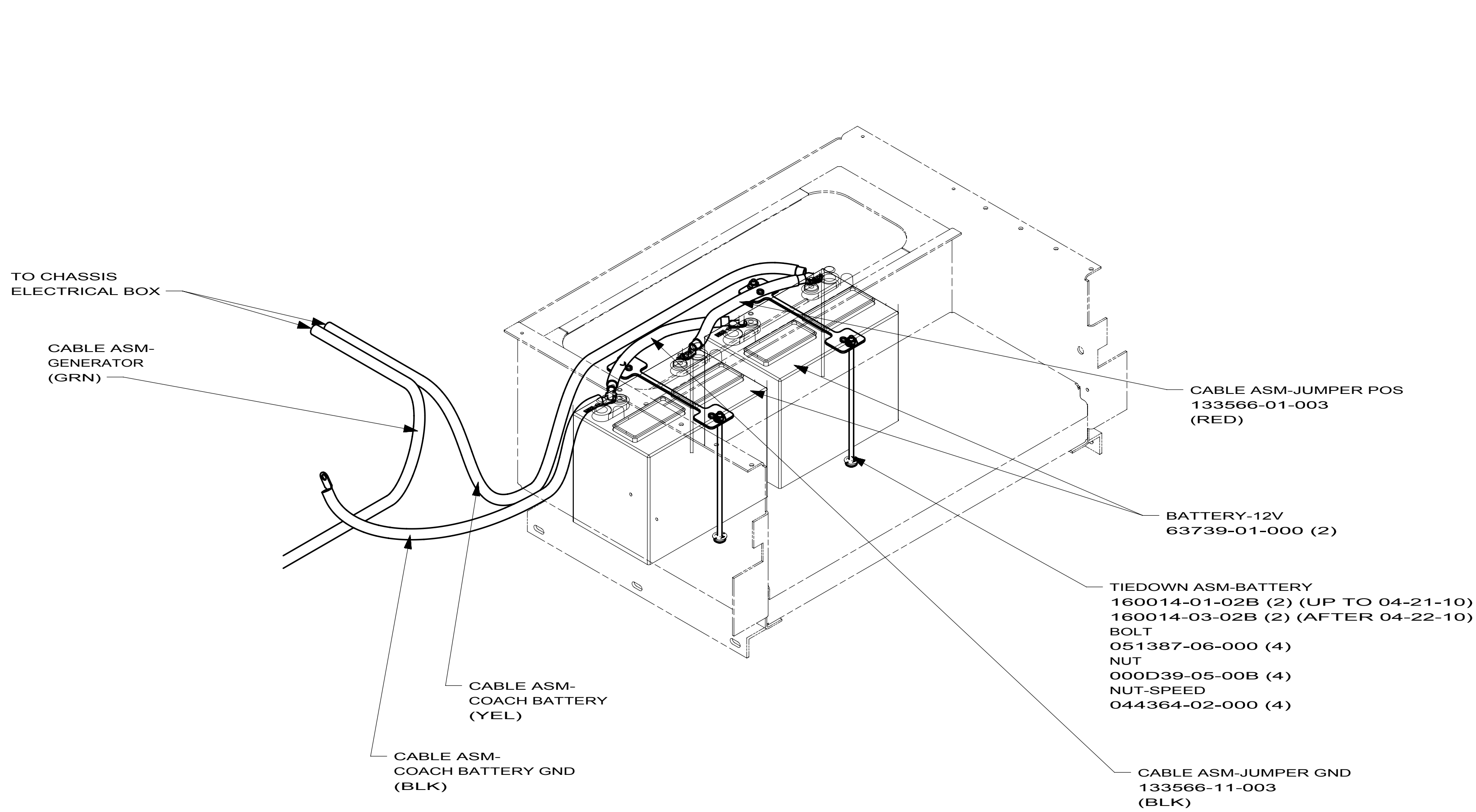
BATTERY BOX
