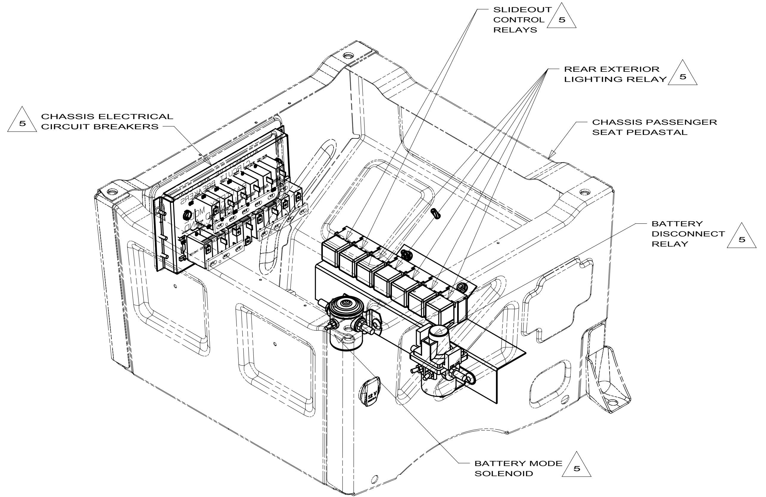
DETAIL CD
