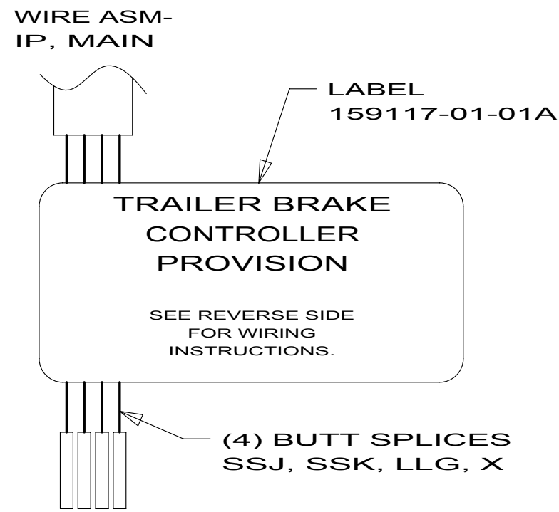
DETAIL CE
