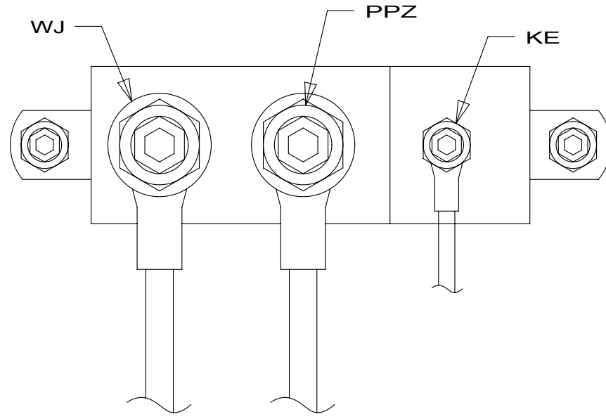
DETAIL CC 3
