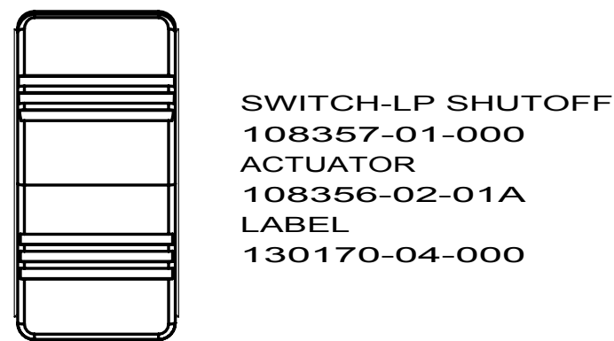
DETAIL CF
