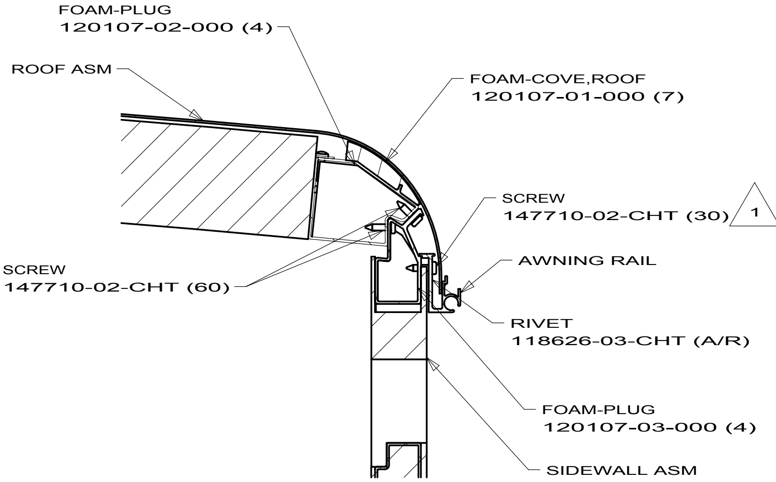
SECTION AC-AC
