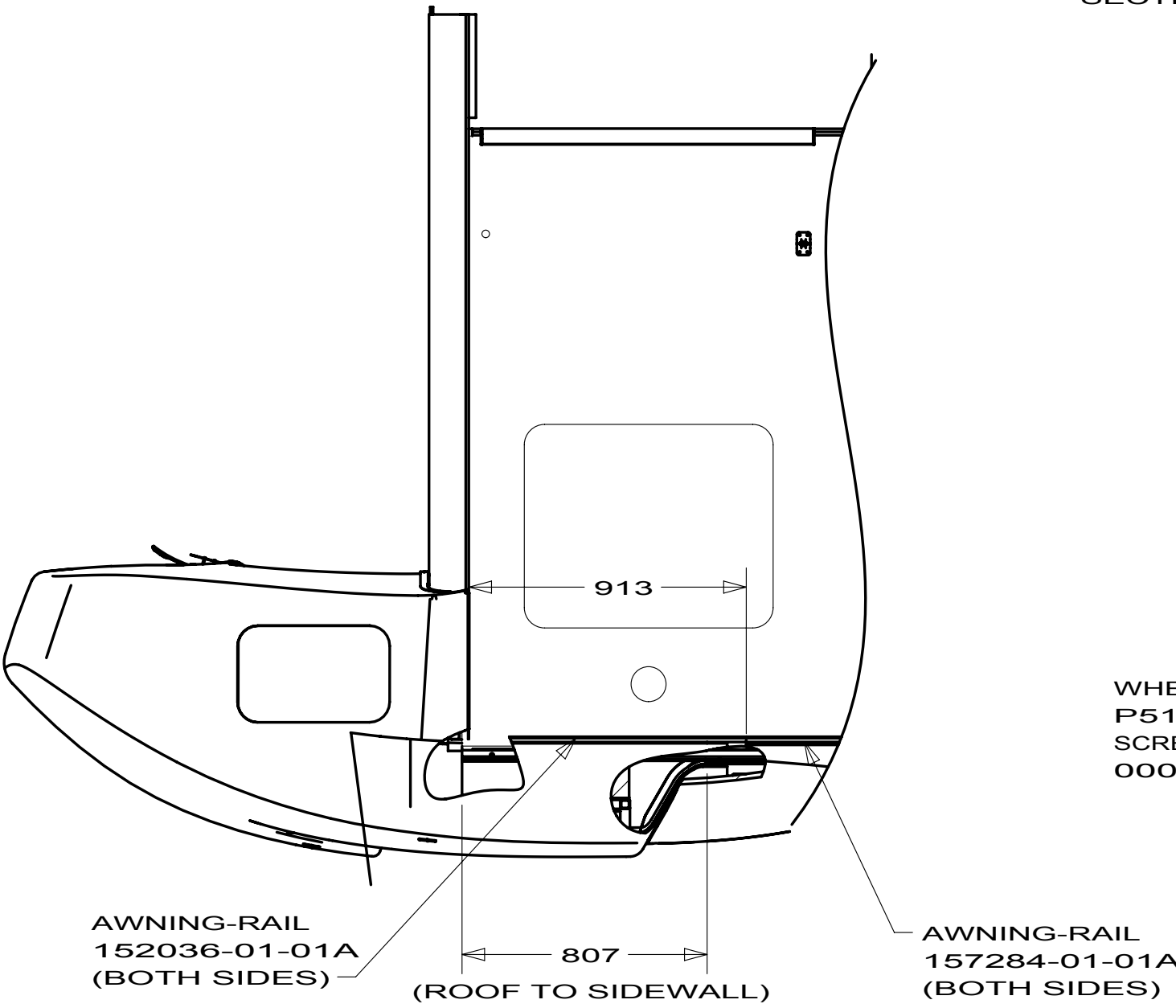
SECTION AF-AF
