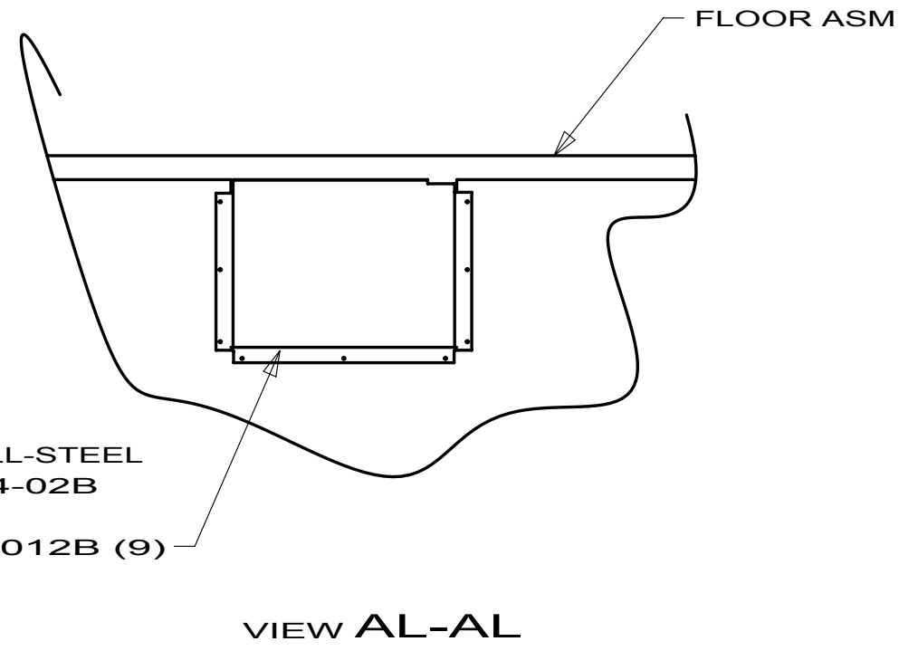
VIEW AL-AL
