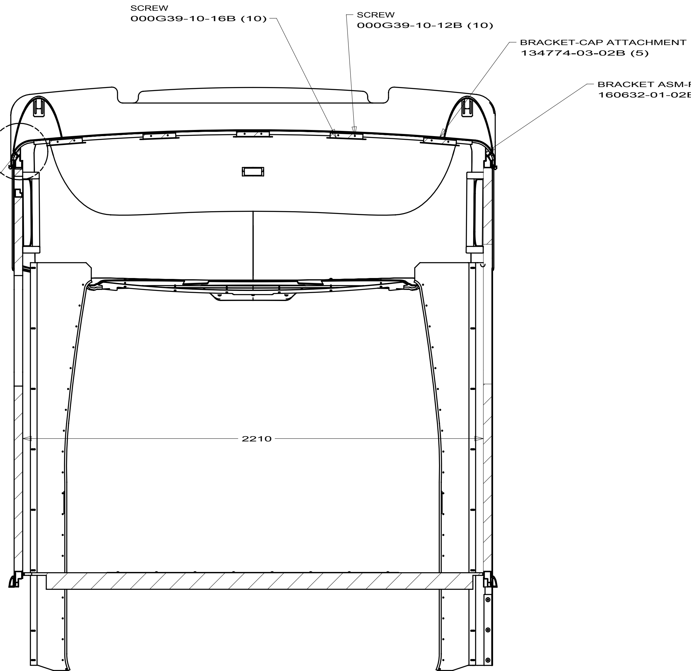
SECTION AH-AH
