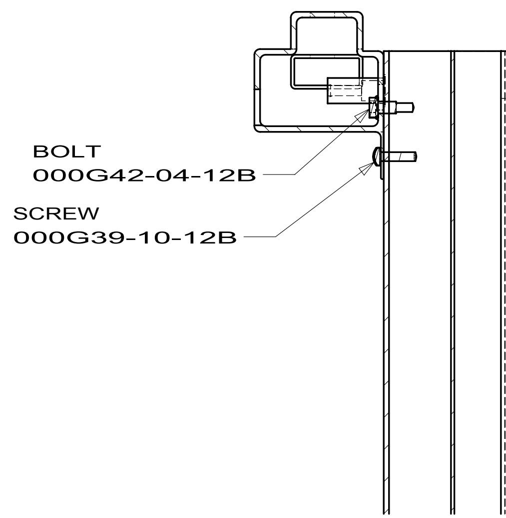
SECTION DA-DA SECTION DB-DB SIMILAR
