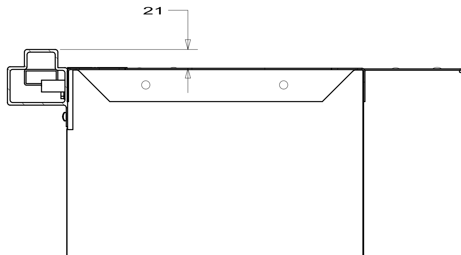
SECTION FD-FD
