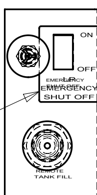
LABEL-WARNING-LPG CANADA 23769-01-000
