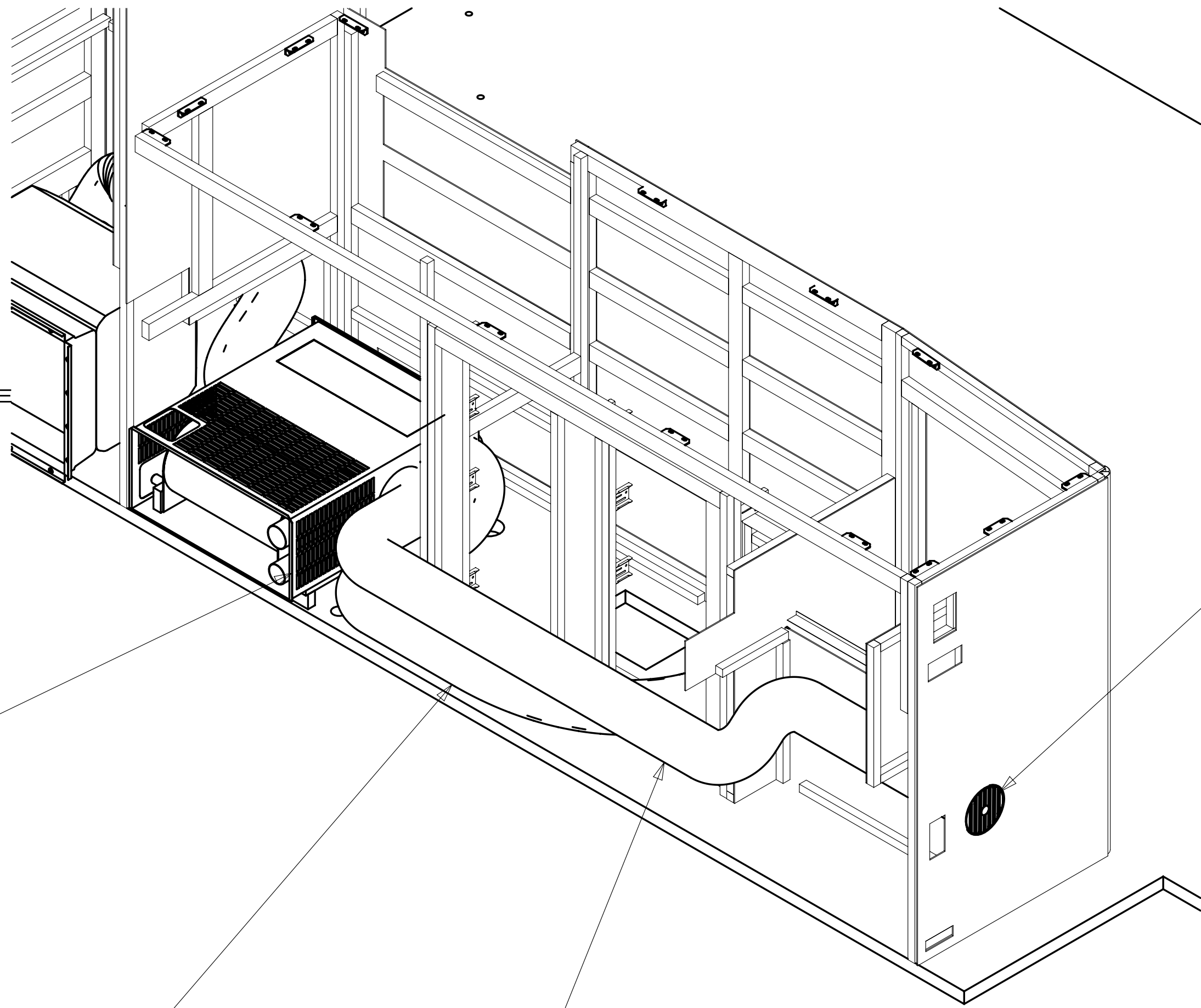
VIEW A
