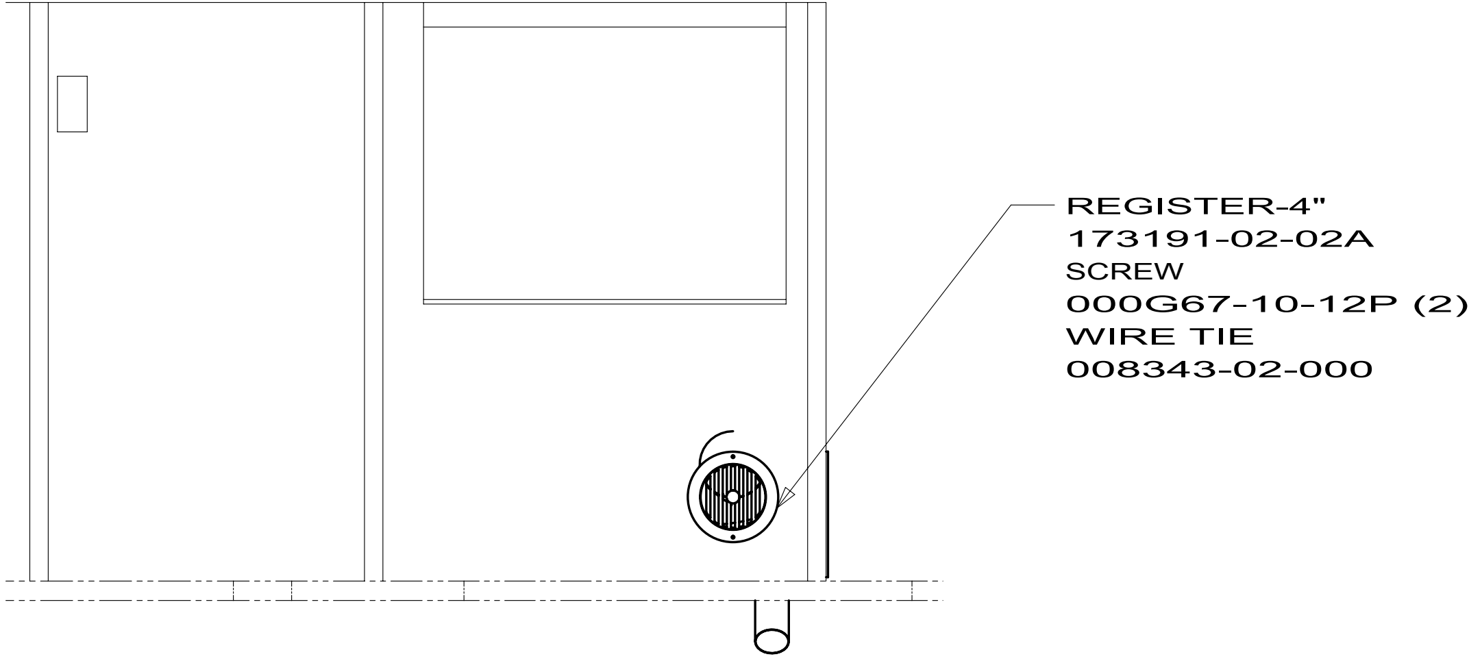
VIEW C
