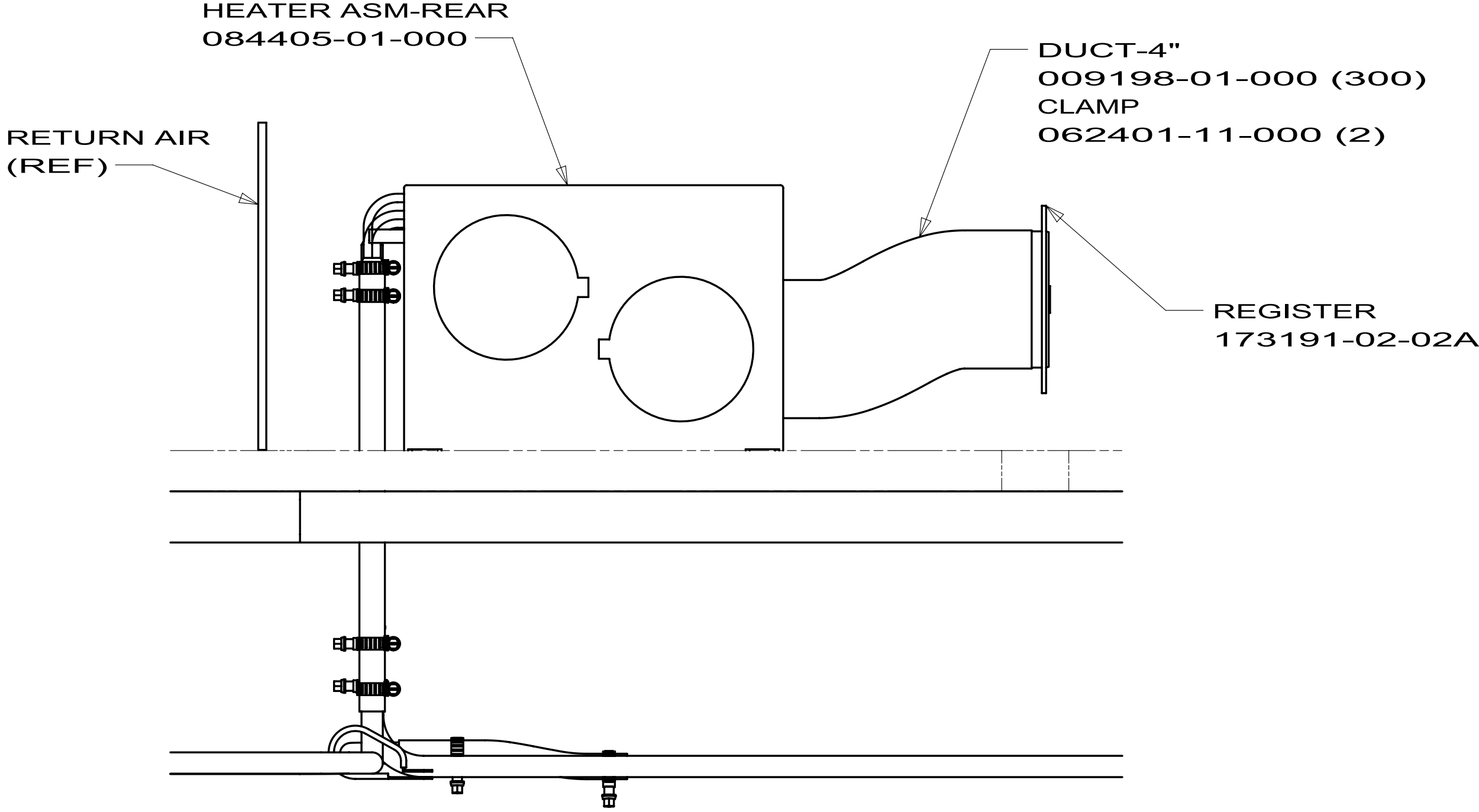
VIEW A
