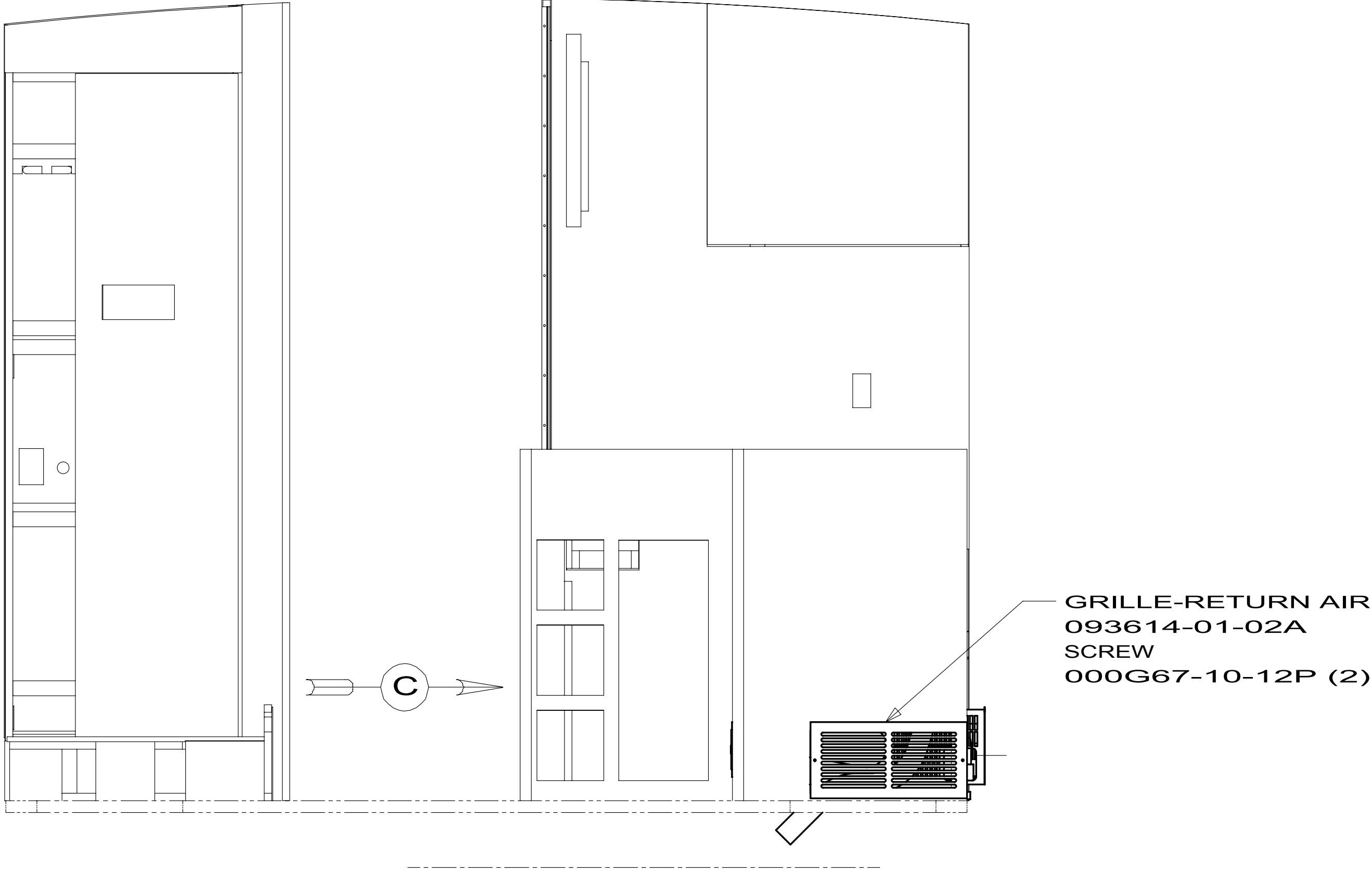
VIEW B
