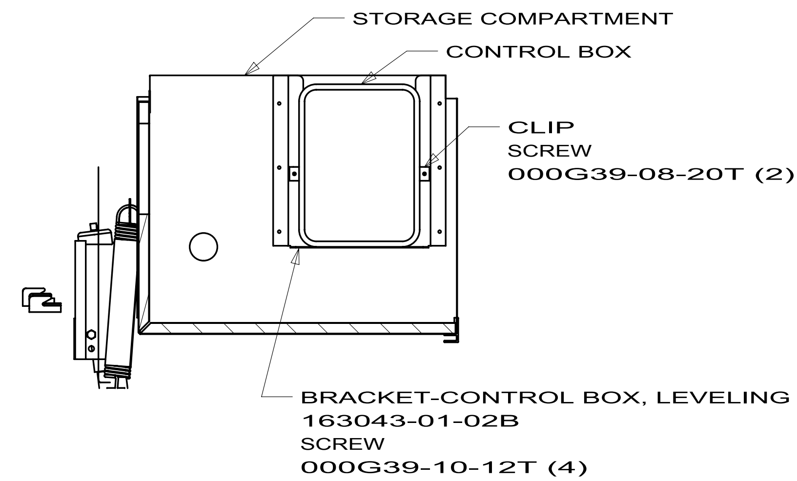
SECTION F-F
