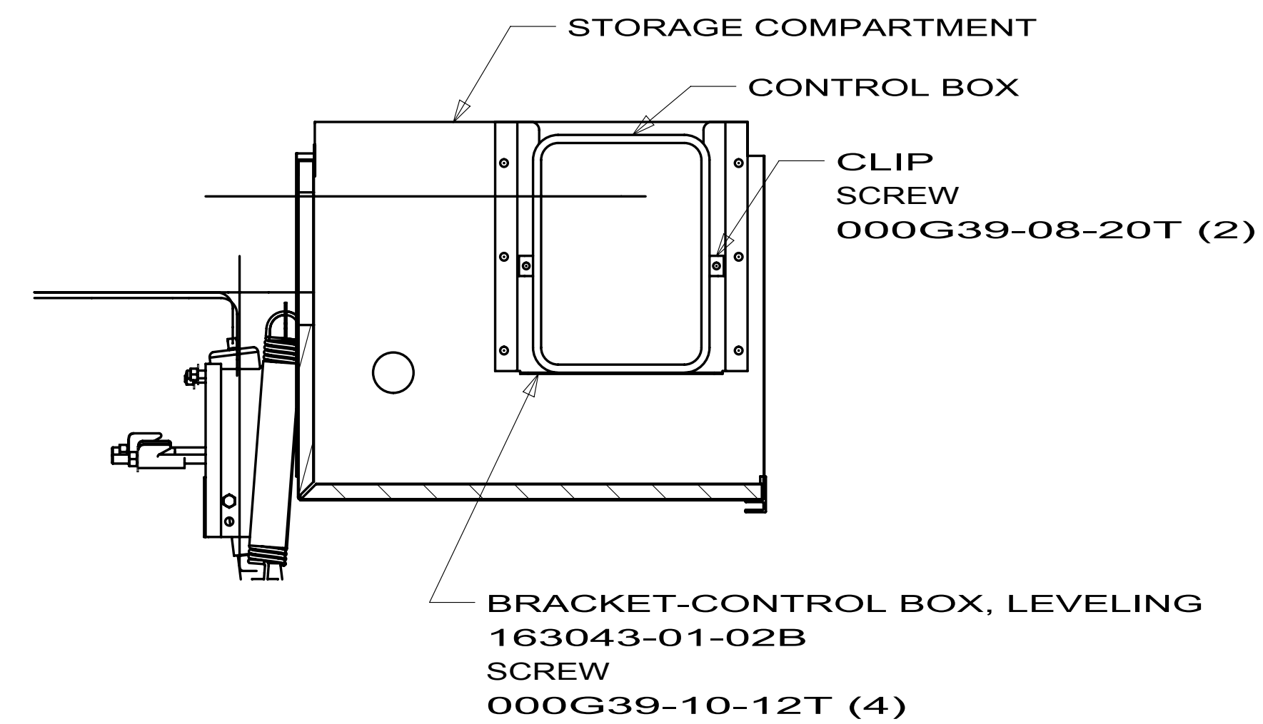
SECTION F-F
