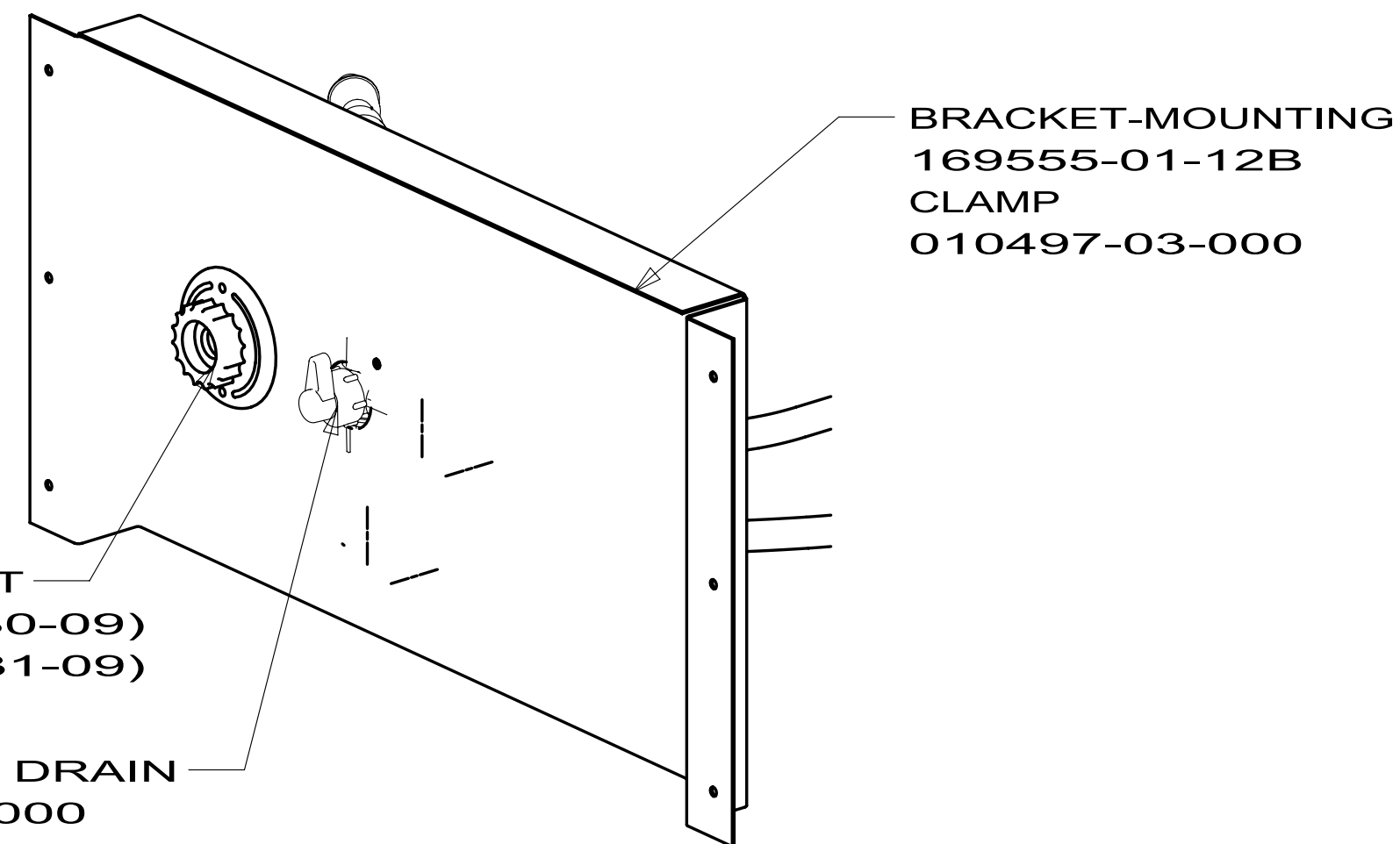
VIEW E
