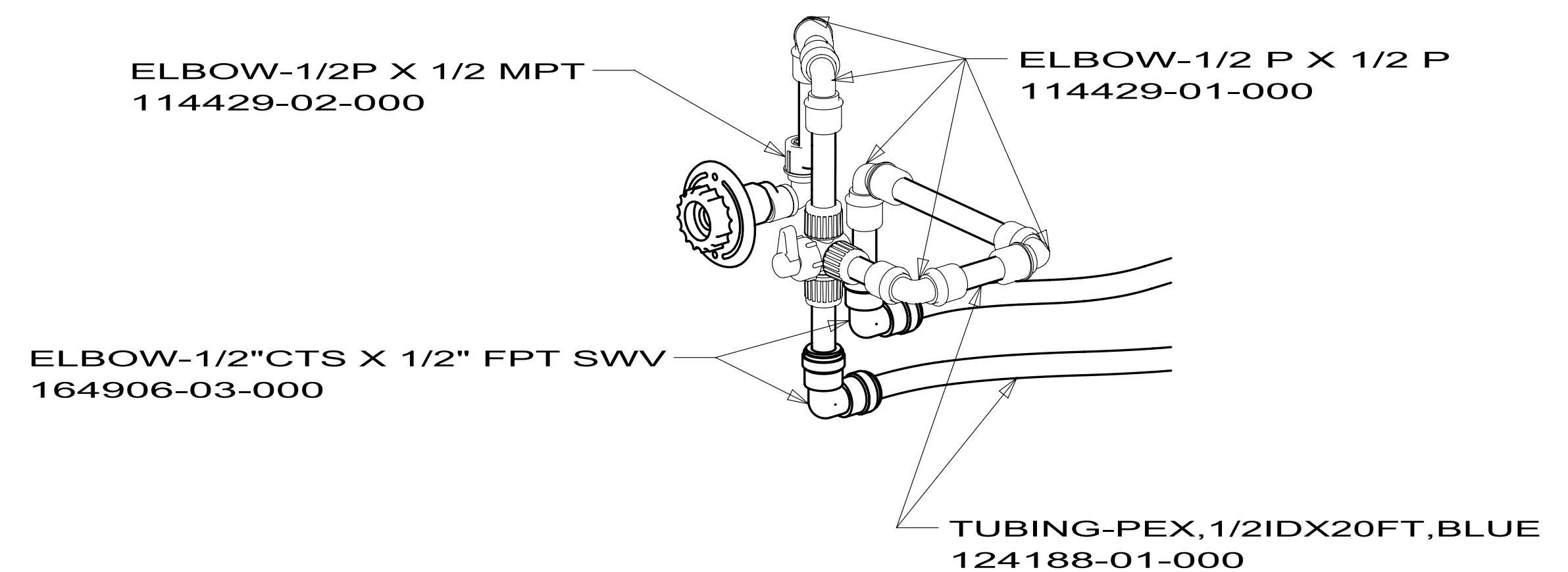
VIEW E (W/OUT BRACKET)
