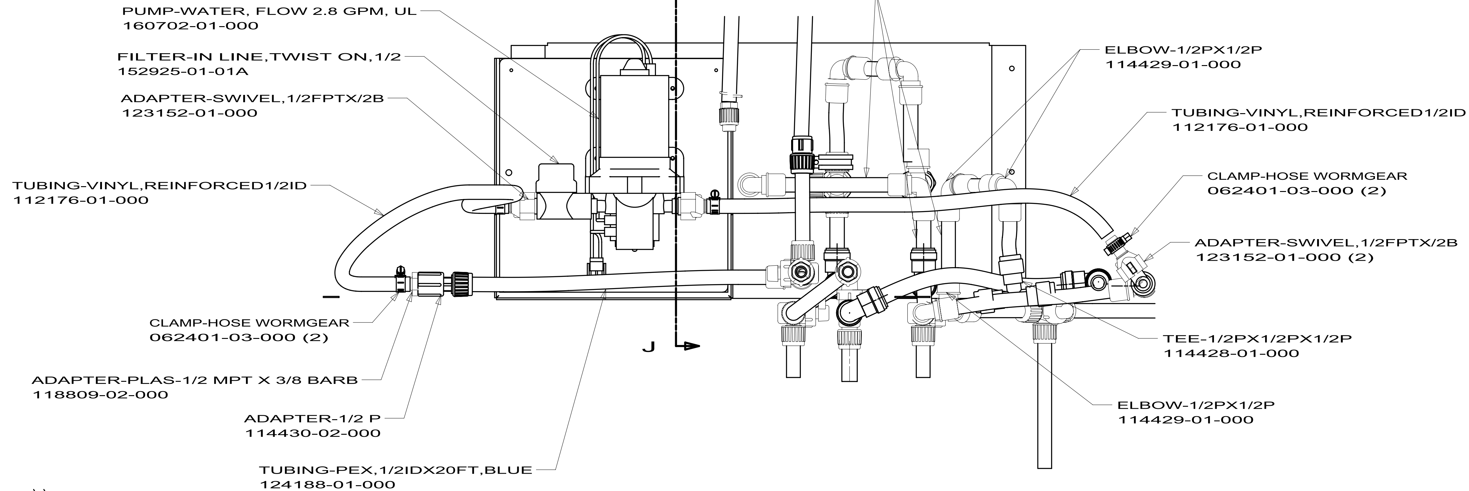
SECTION H-H (ROTATED)
