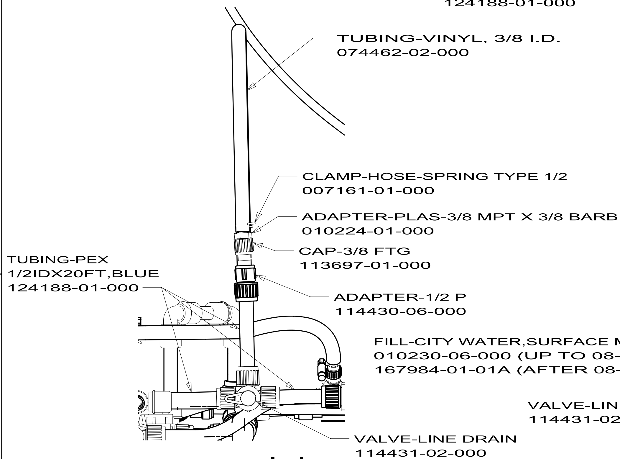
SECTION J-J
