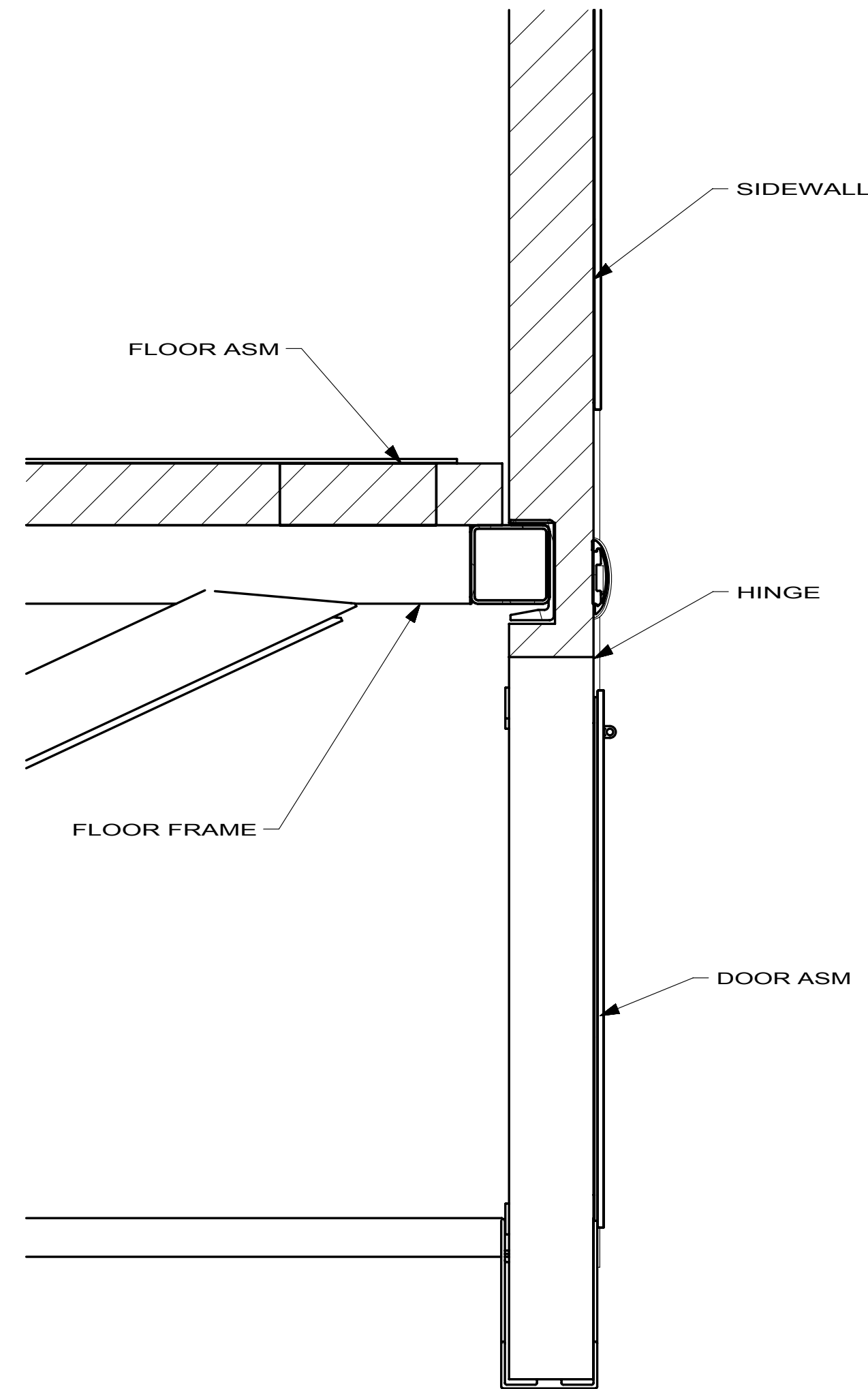
SECTION BA-BA
