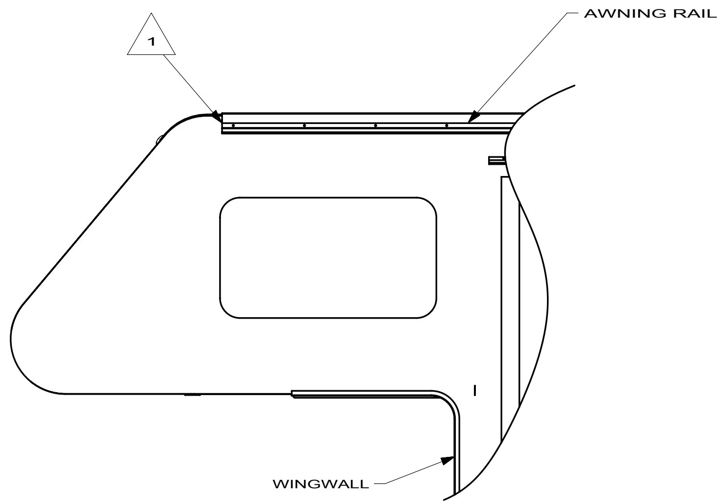
DETAIL AK
