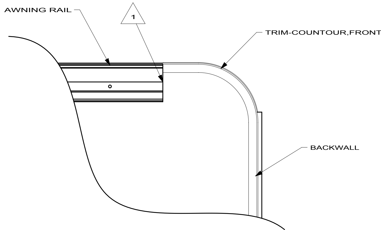
DETAIL AL
