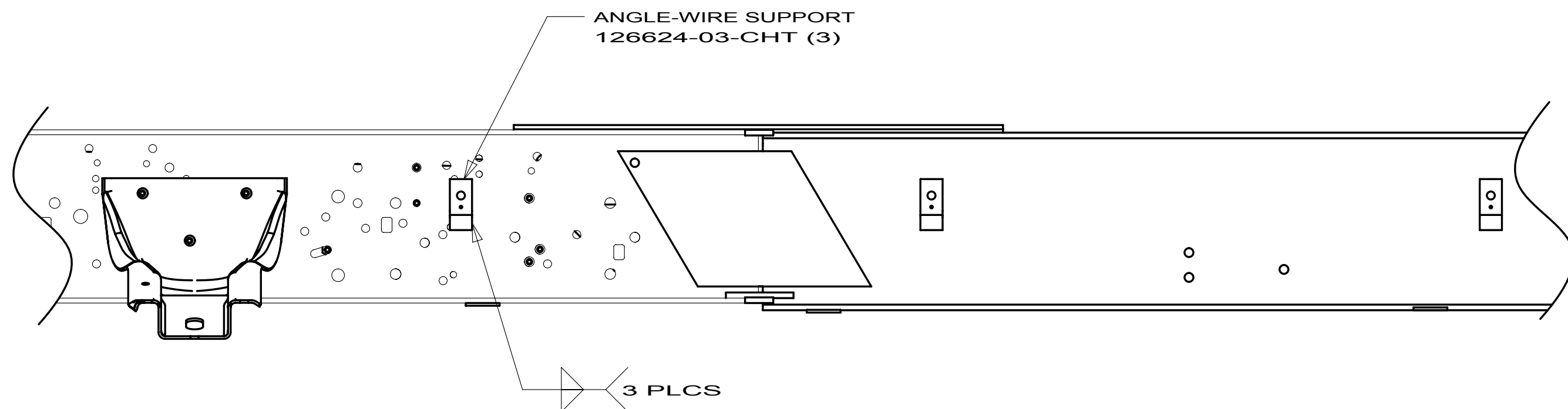
SECTION BB-BB
