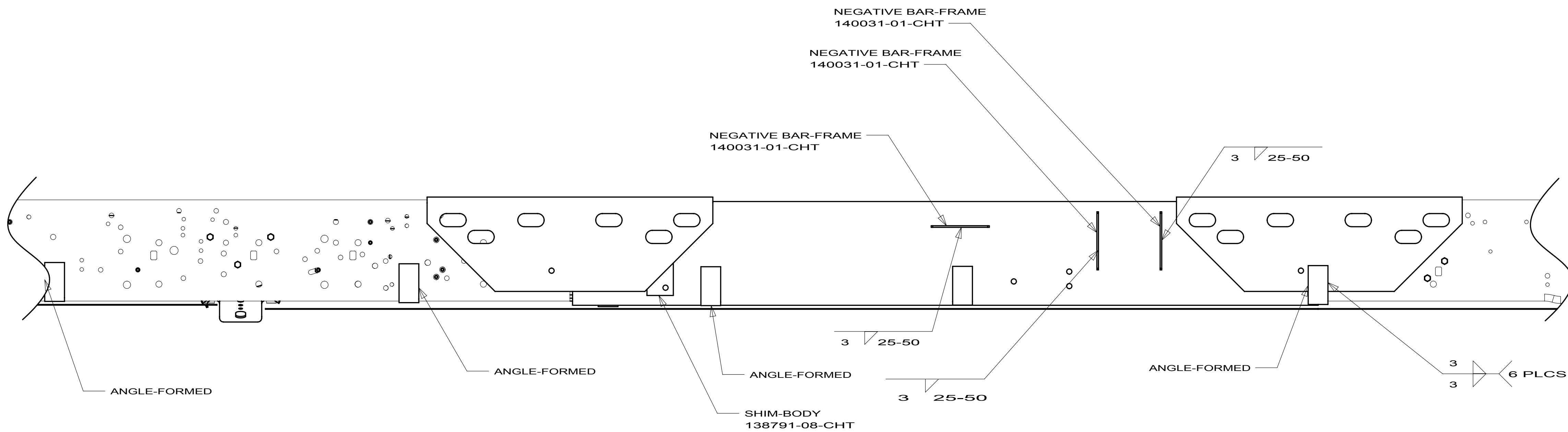
SECTION BA-BA
