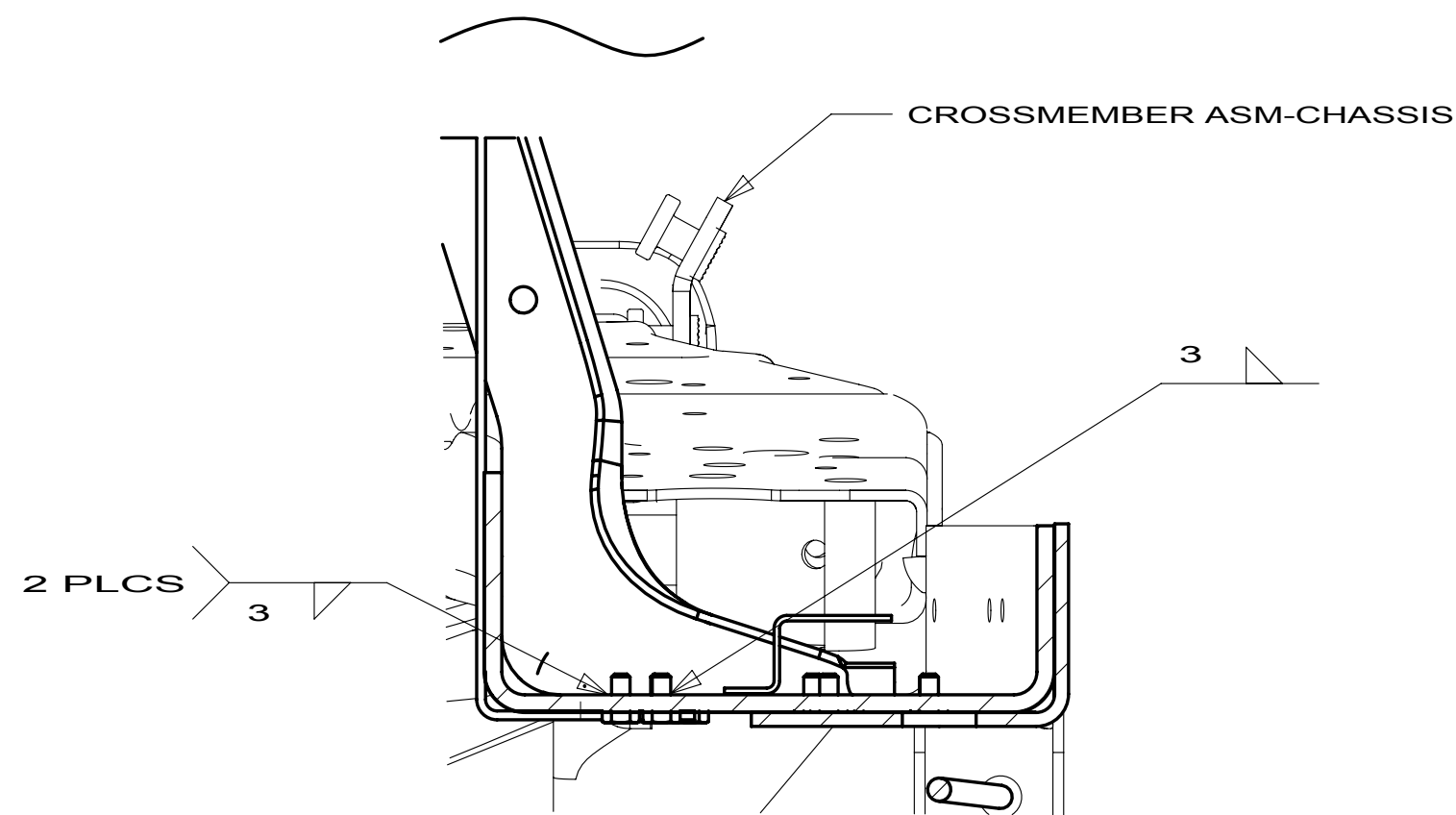
SECTION BF-BF
