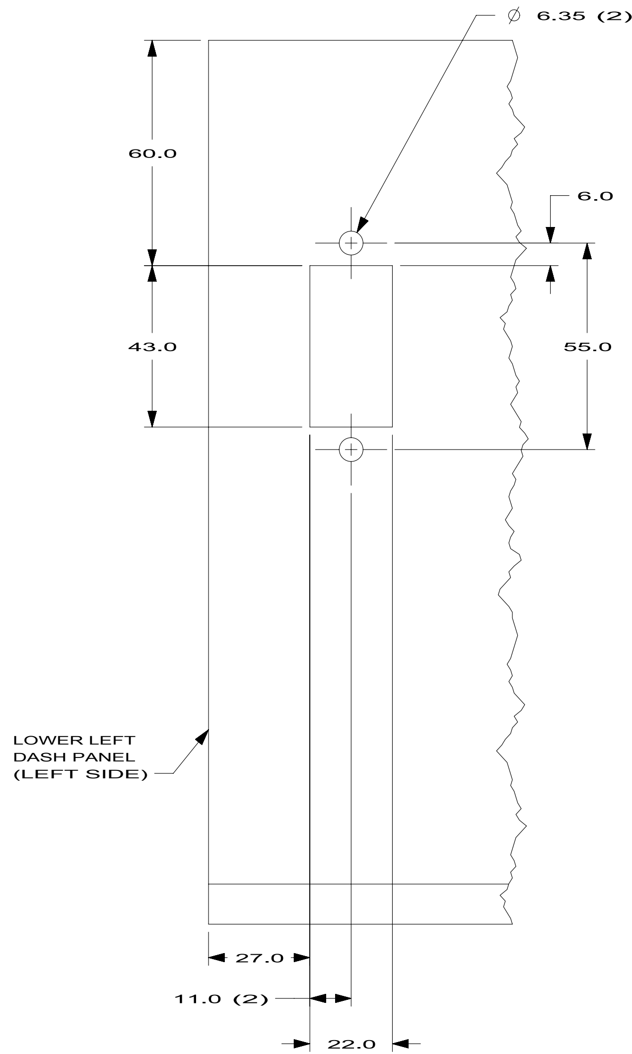
VIEW CB-CB
