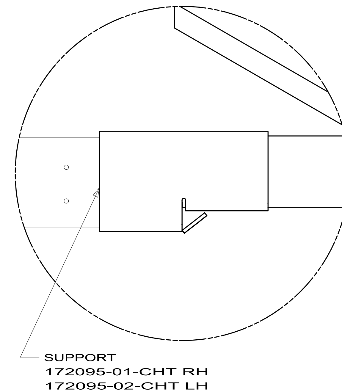
DETAIL BC
