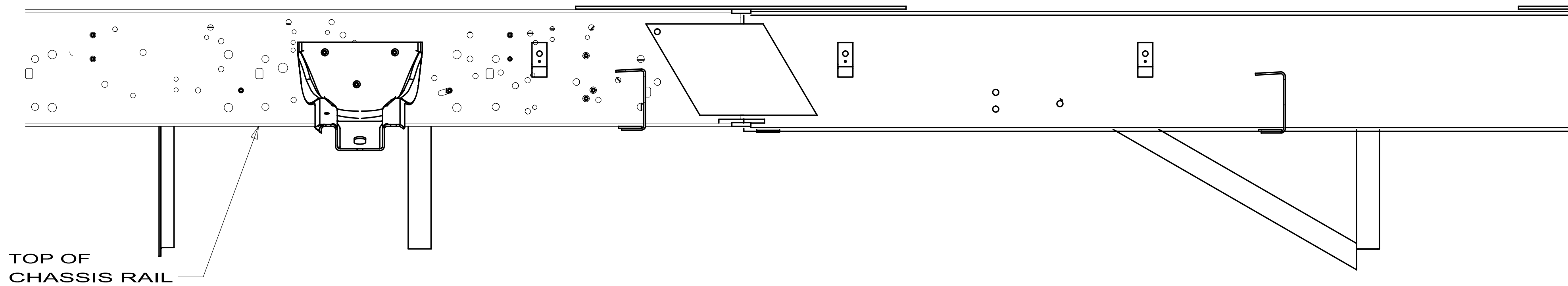
SECTION BF-BF
