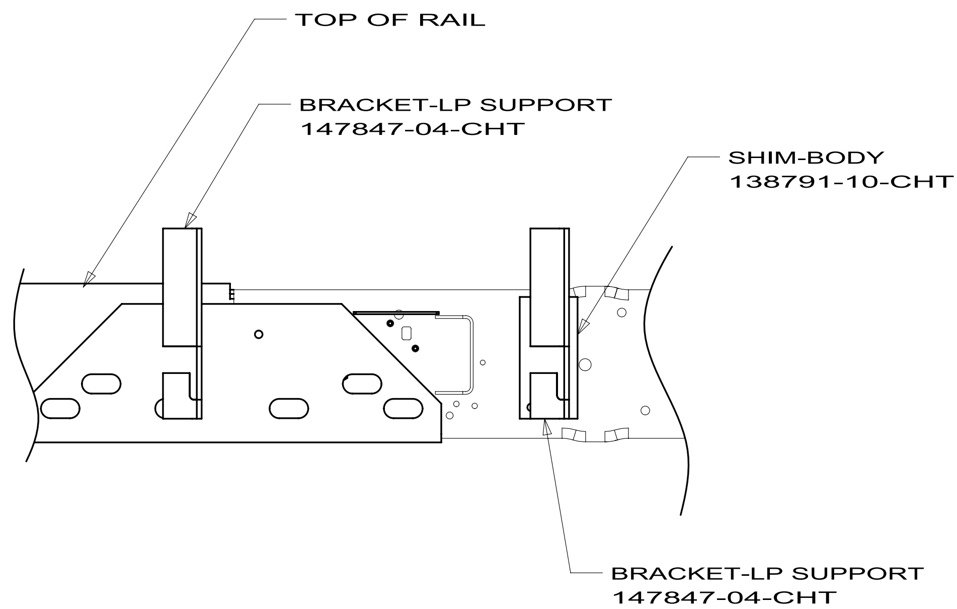
VIEW BB-BB
