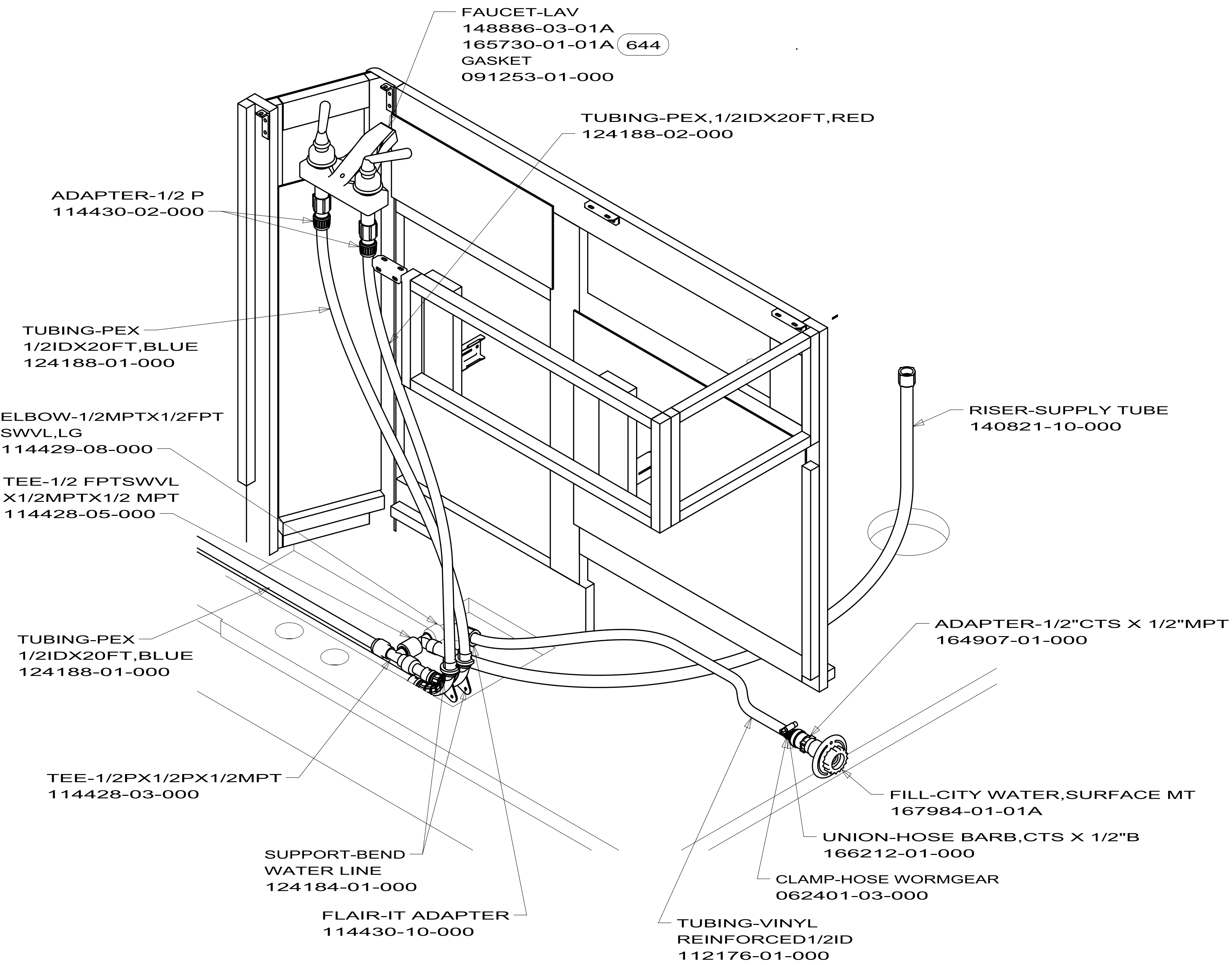
VIEW A
