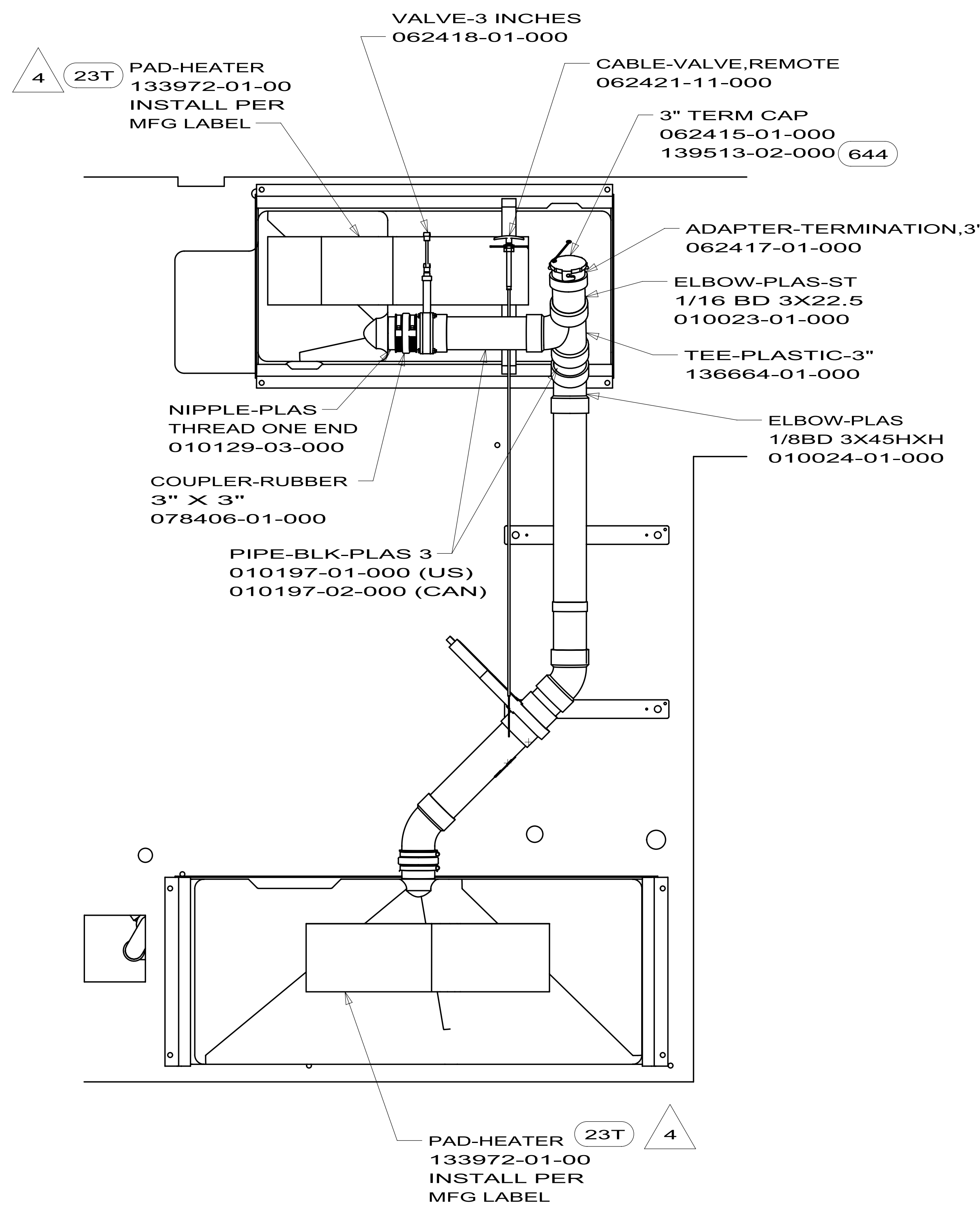
VIEW F
