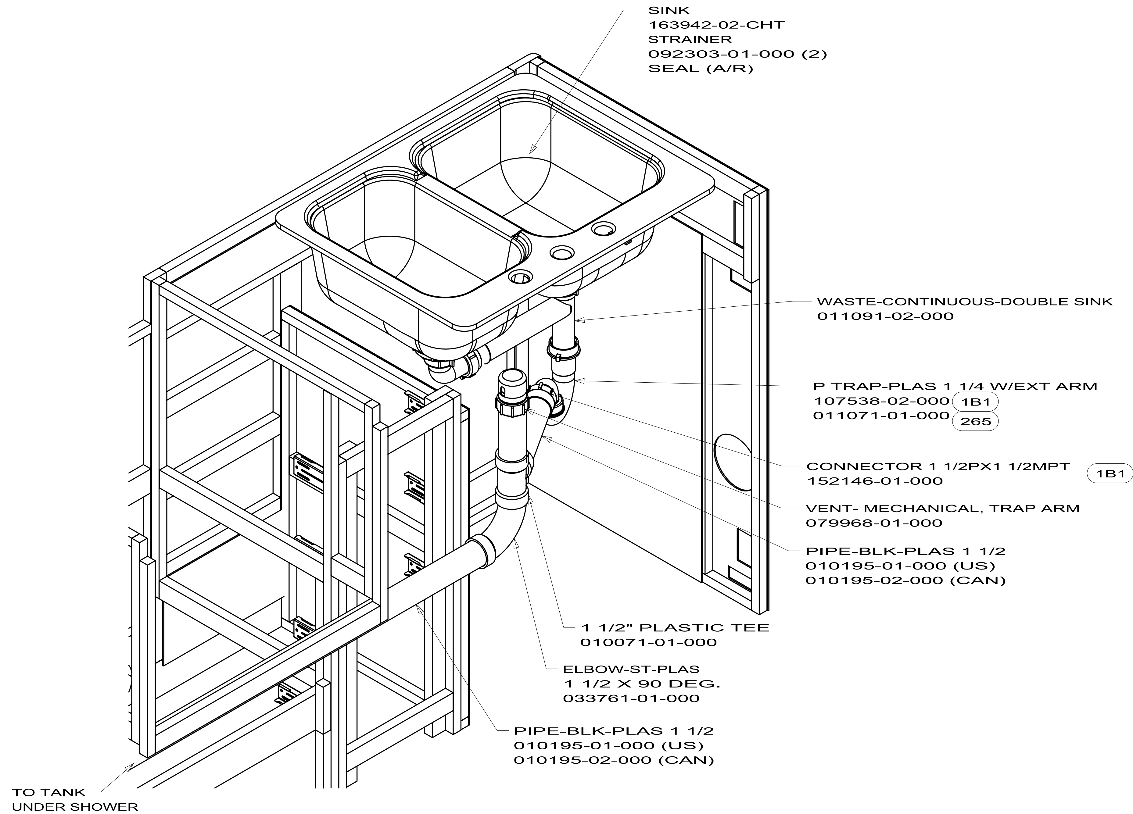
VIEW E
