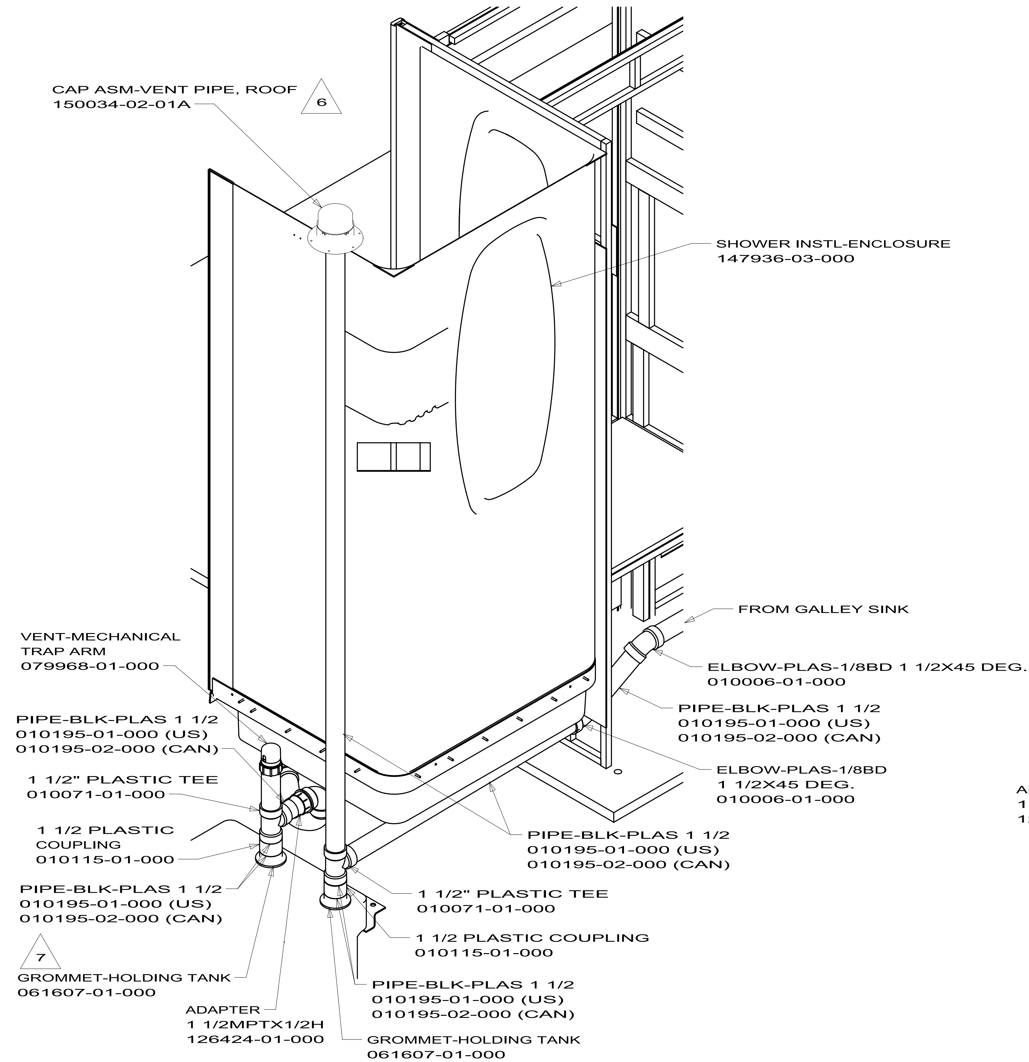
VIEW C
