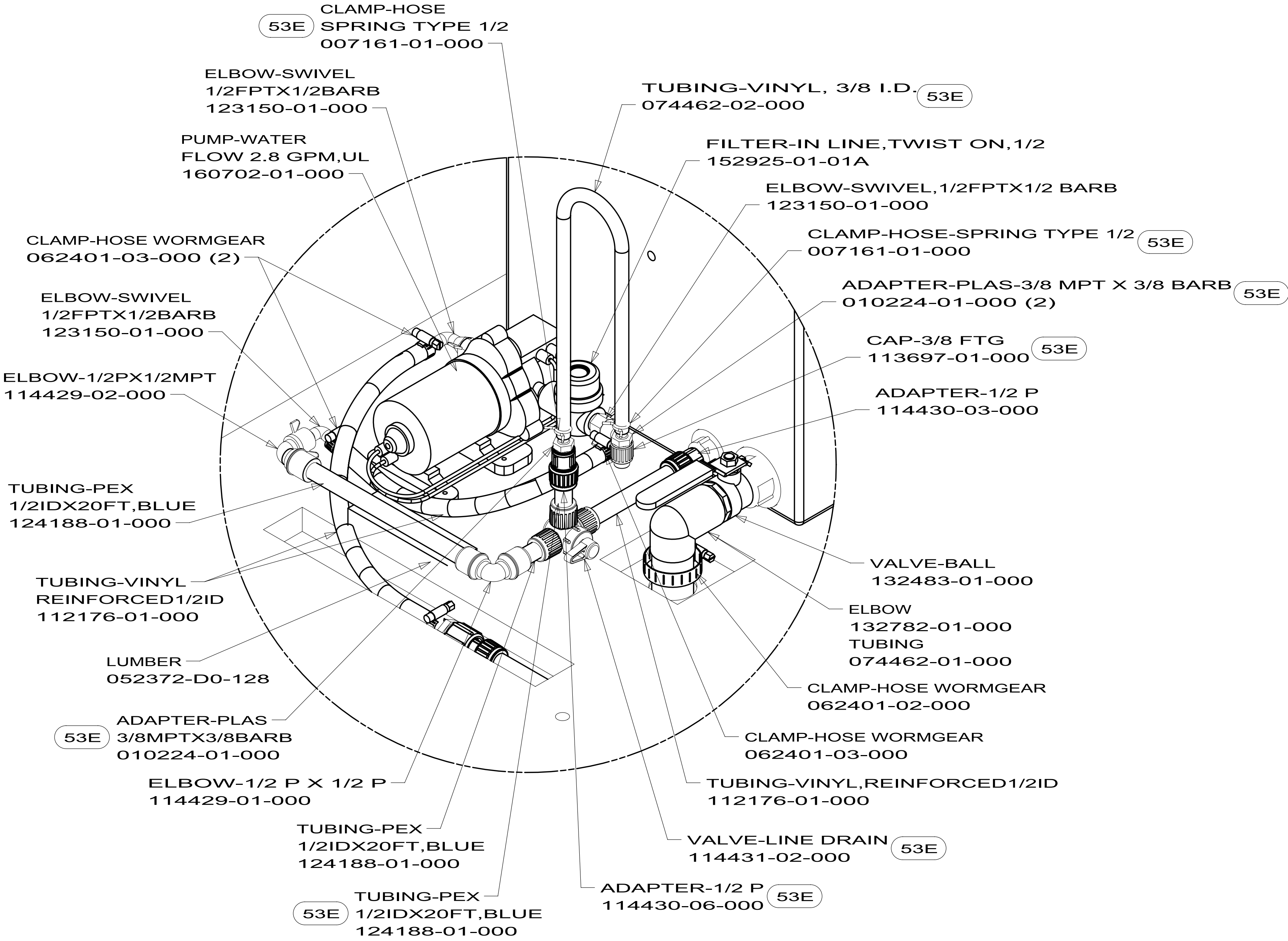
DETAIL F
