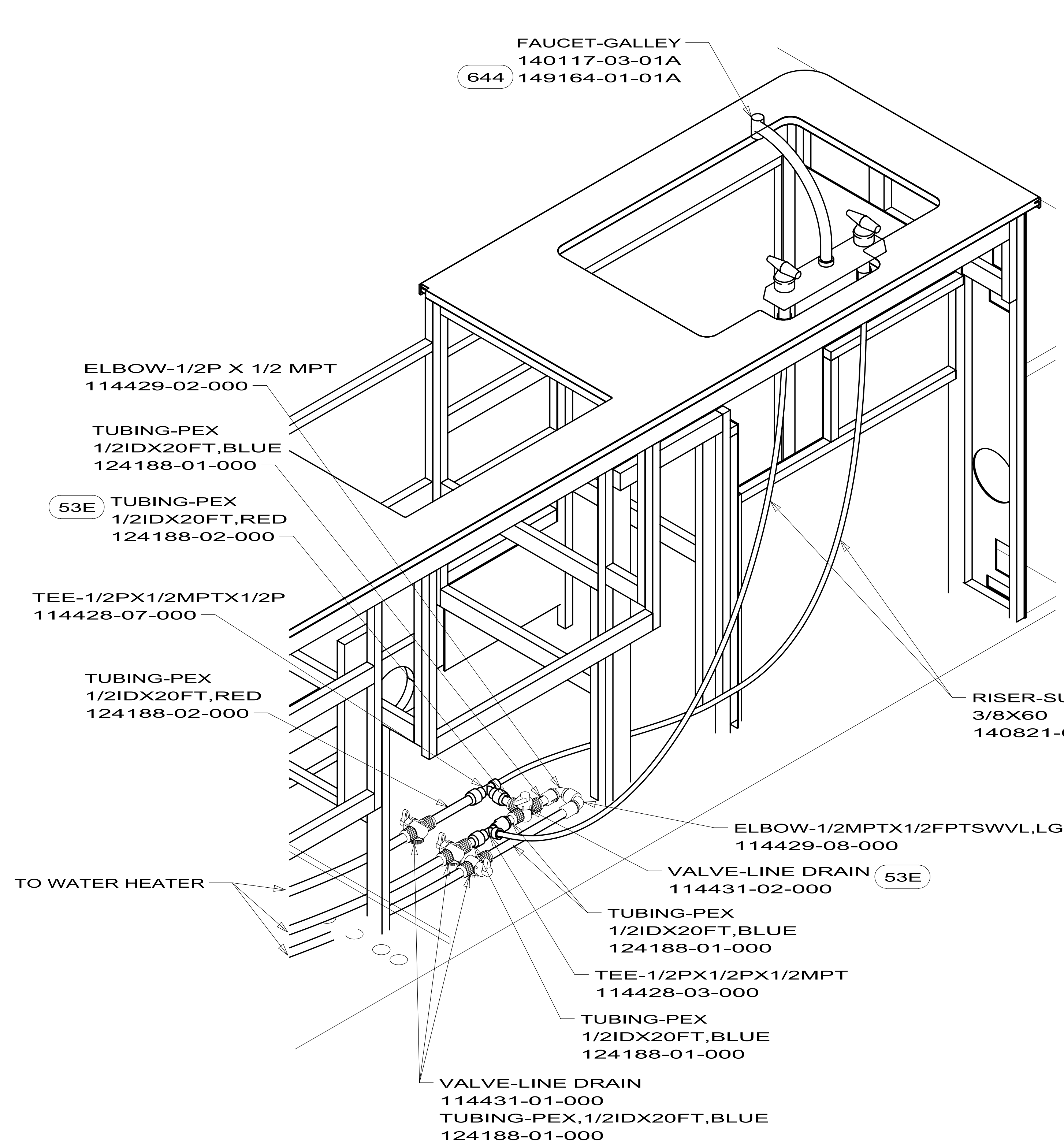
VIEW B
