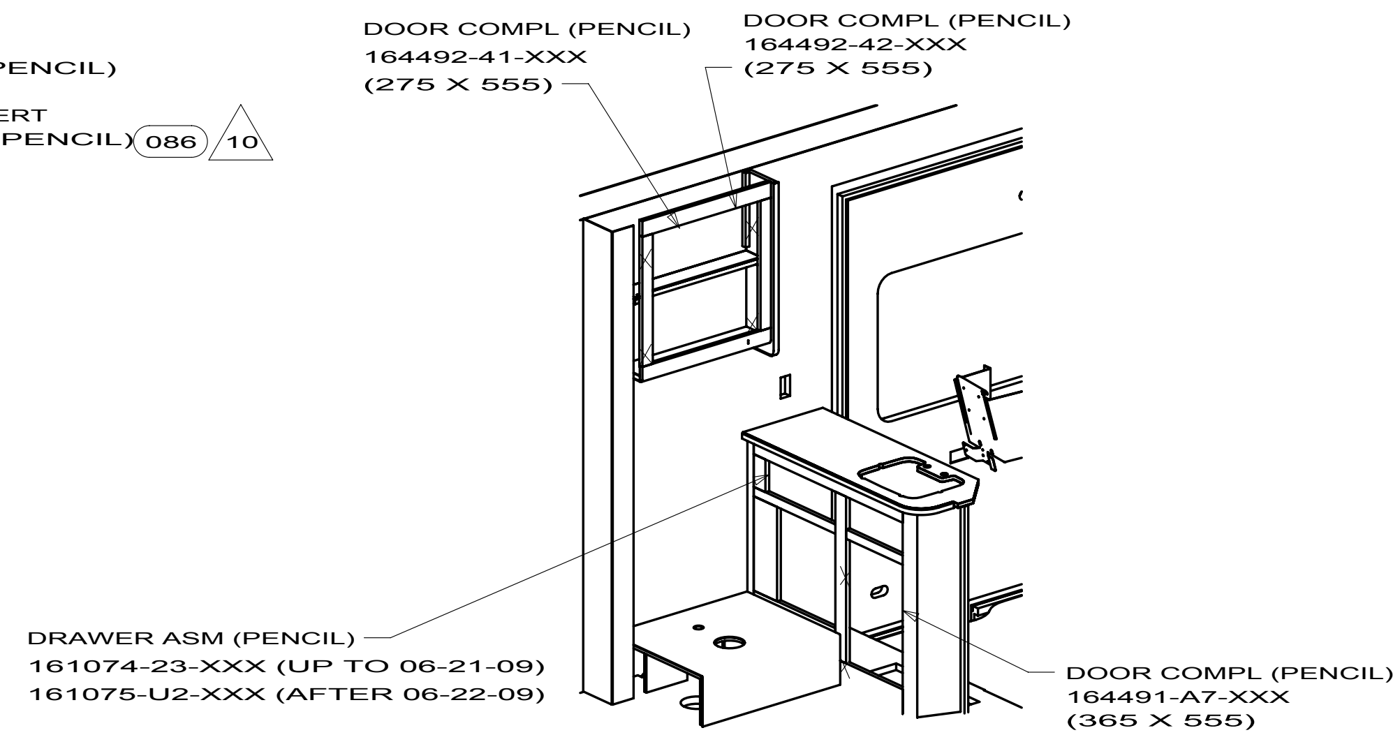
VIEW D
