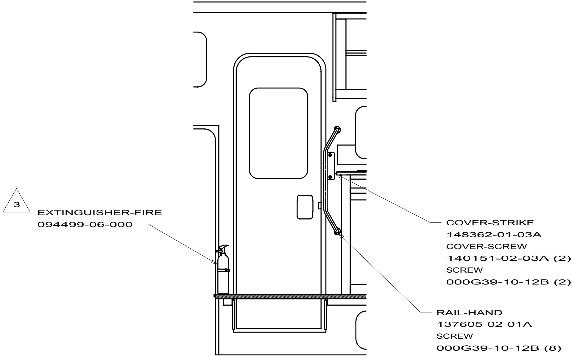
SECTION C-C
