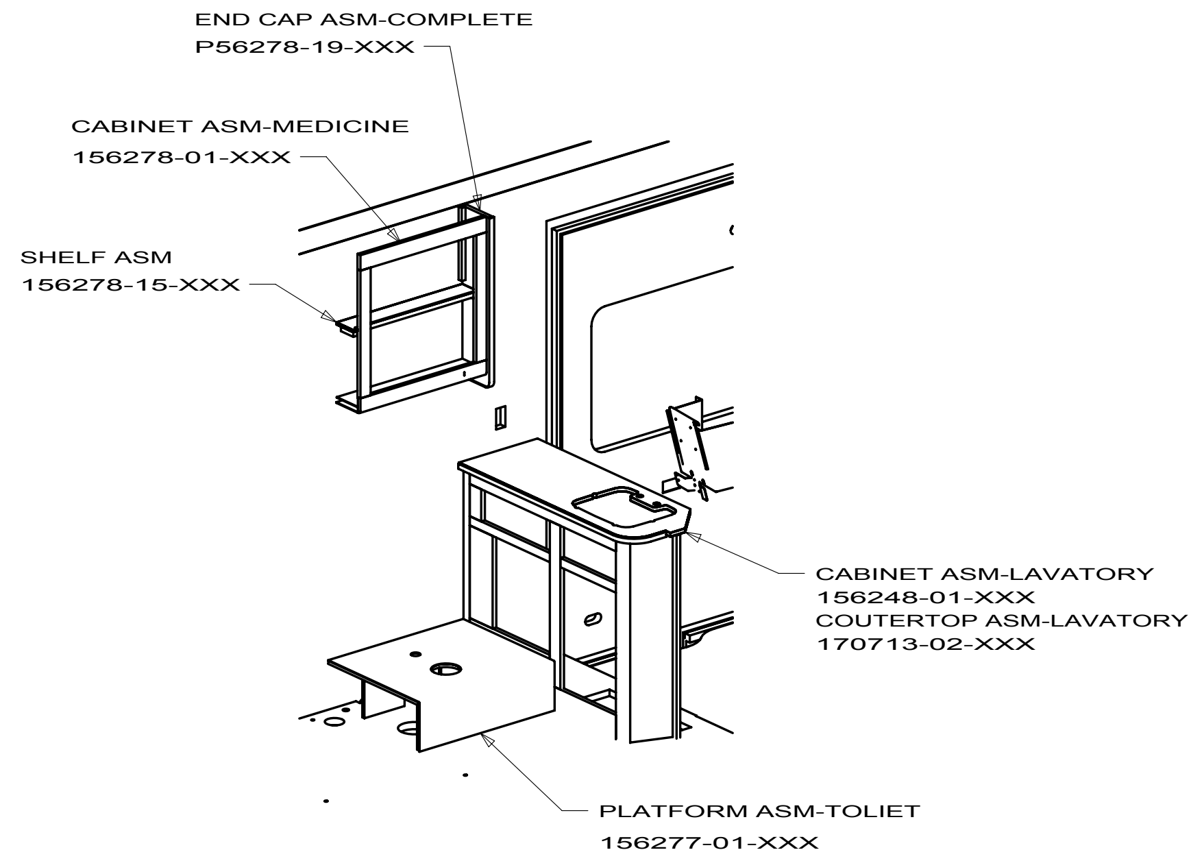
VIEW C
