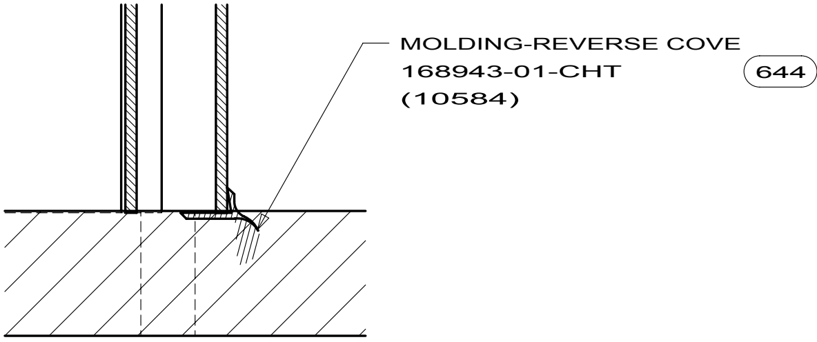
SECTION E-E
