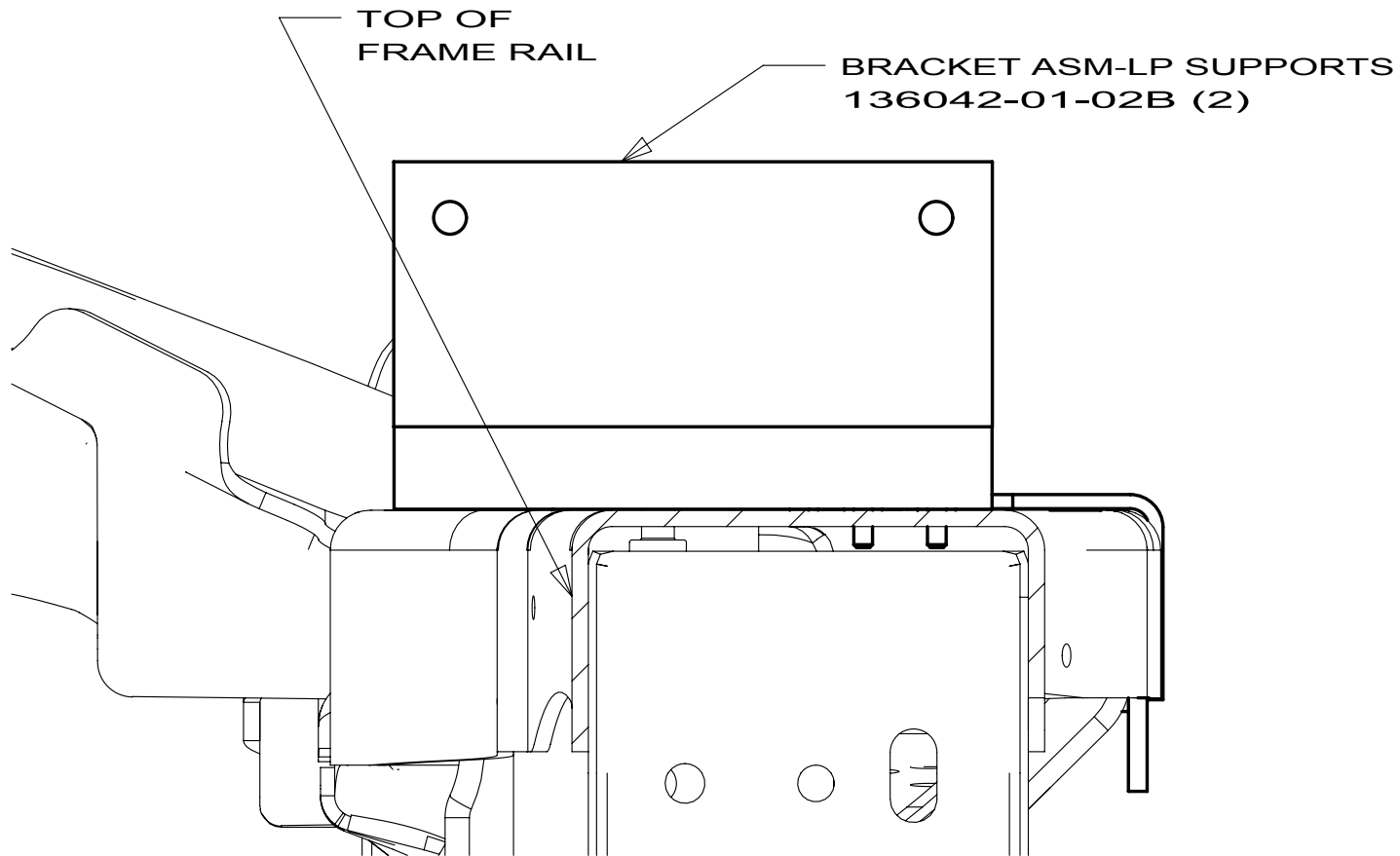
SECTION BC-BC
