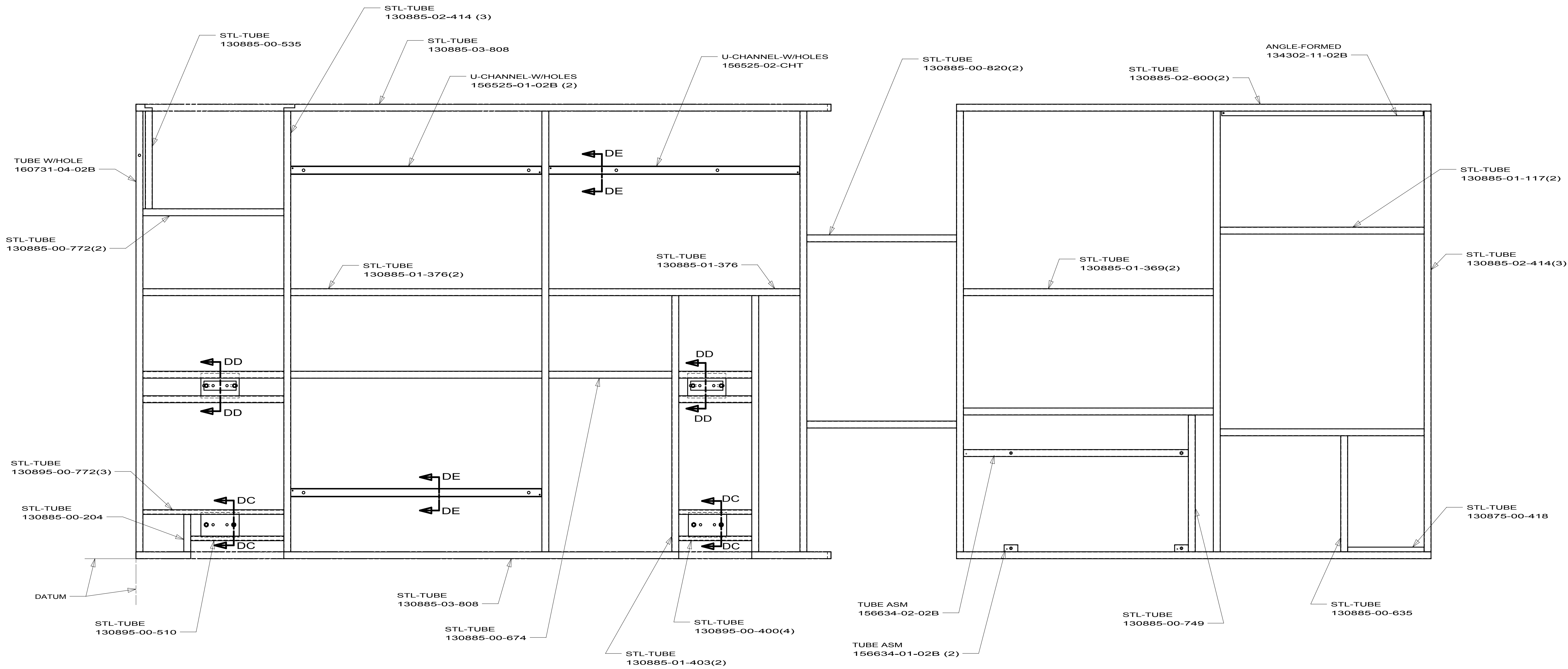
DETAIL DA FLOOR FRAME-LOWER 172910-13-02B
