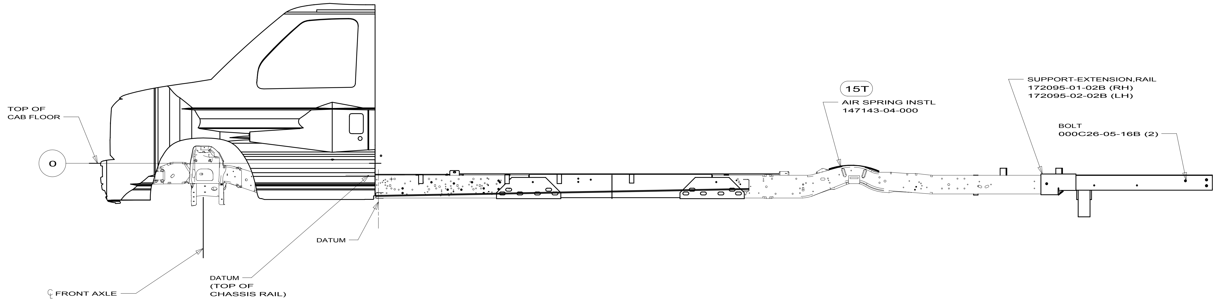
DETAIL AA RAIL ASM 172910-11-02B
