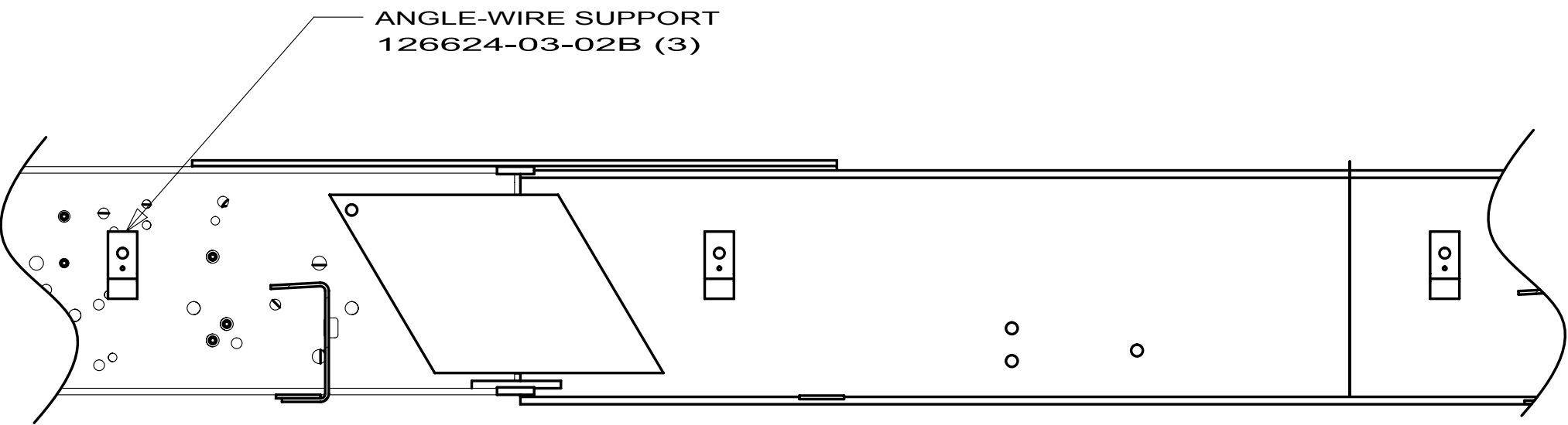
SECTION BB-BB
