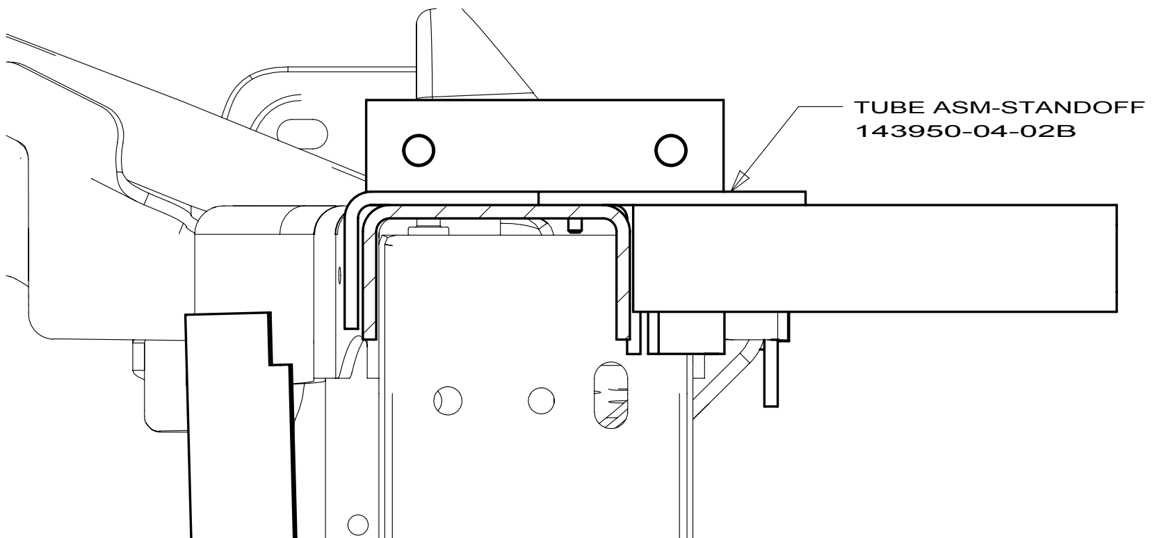
SECTION BD-BD
