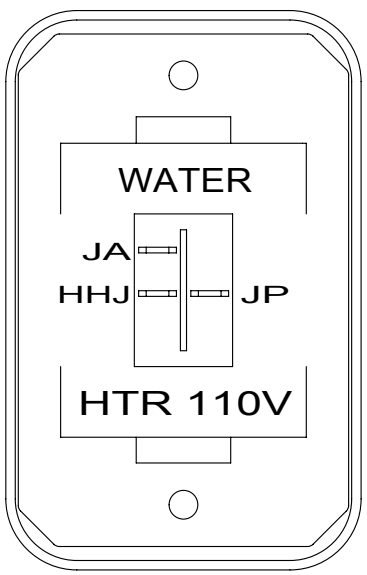
DETAIL CF 53B
