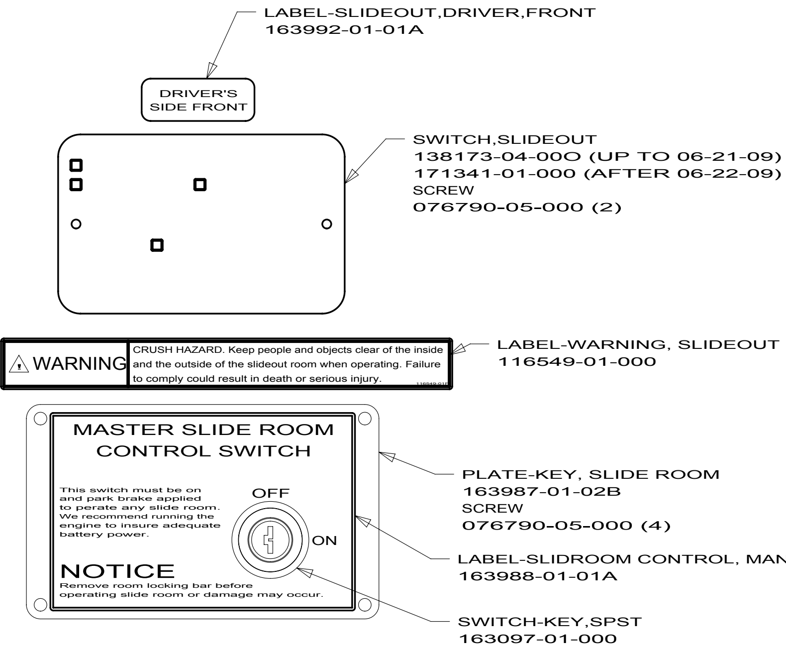
DETAIL CB 09T
