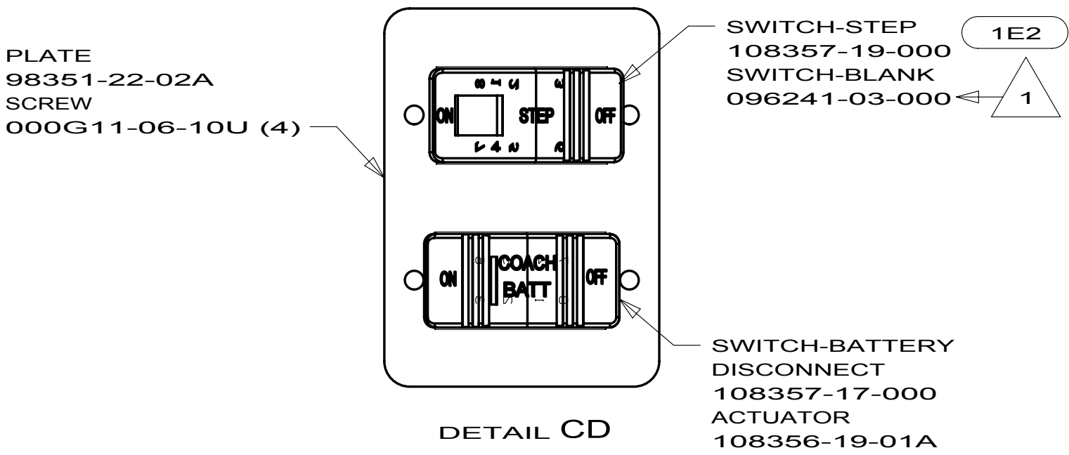
DETAIL CD
