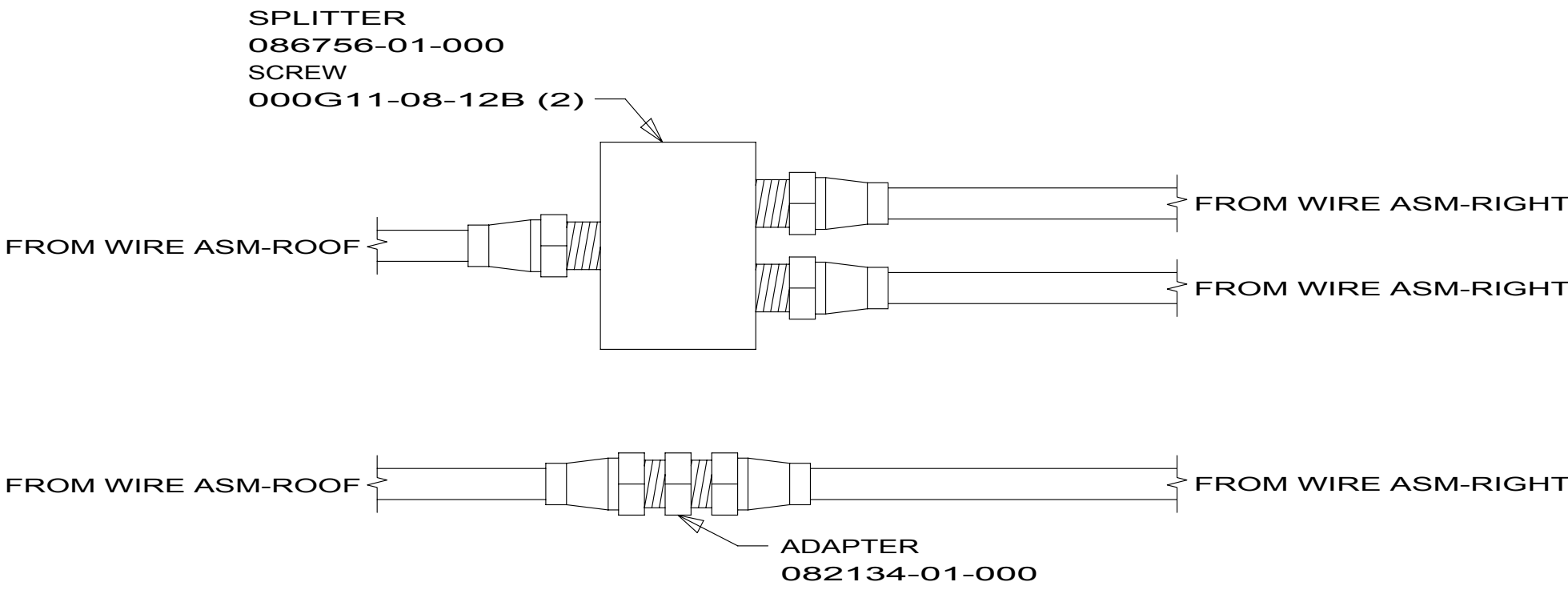
DETAIL CH
