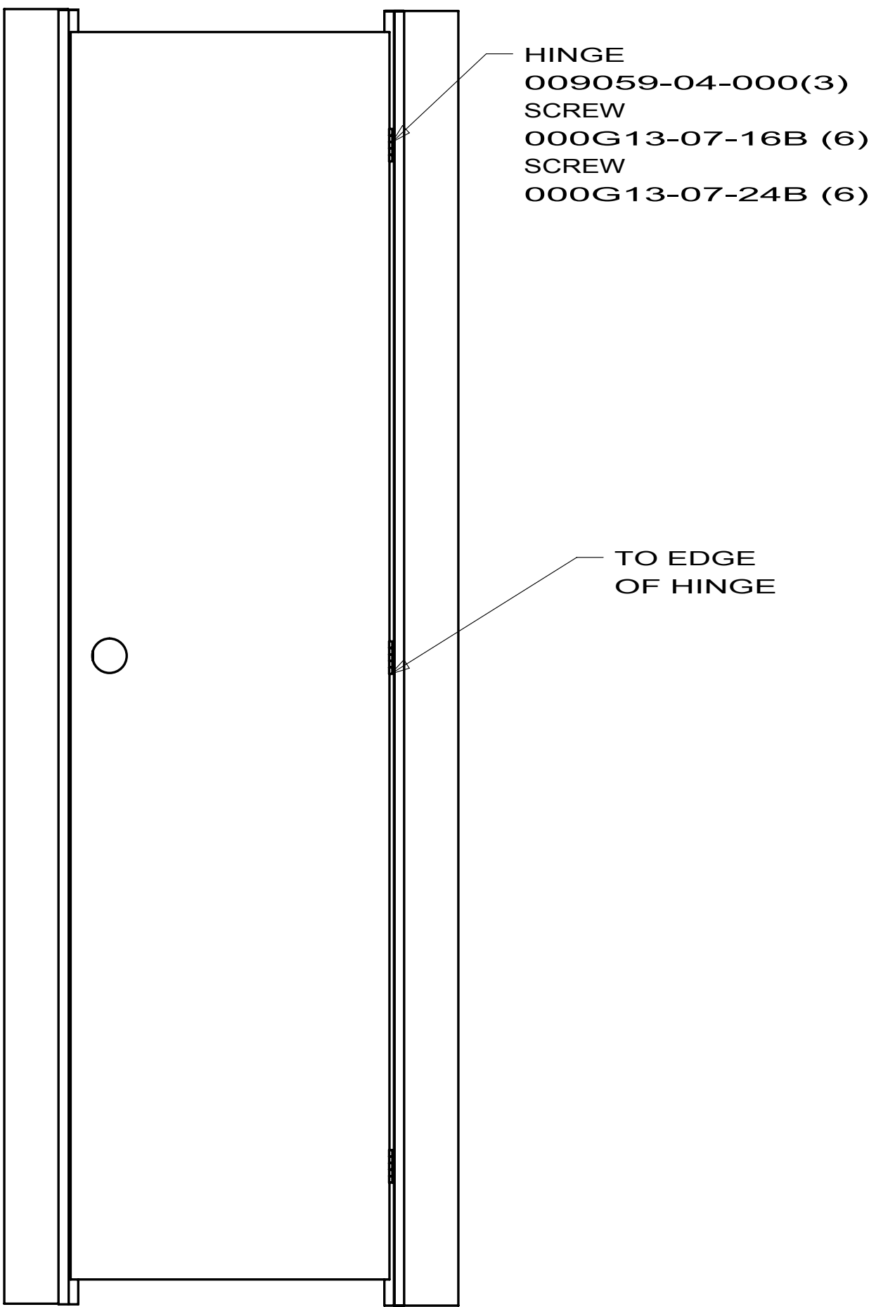
VIEW BL
