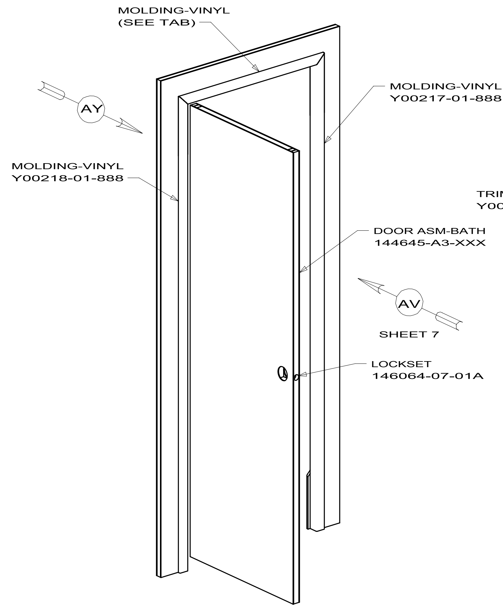
DETAIL AX
