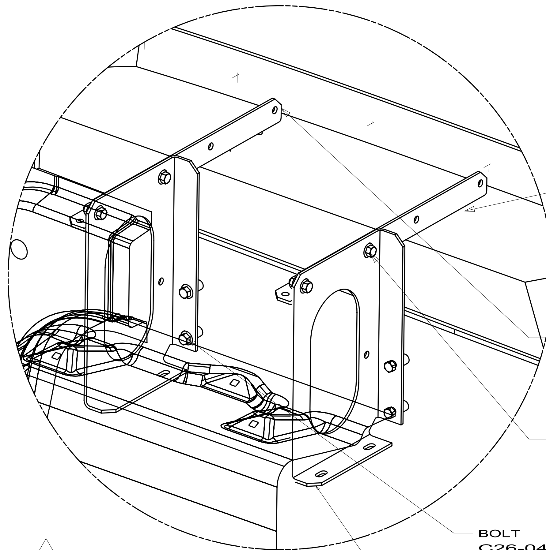
DETAIL CB
