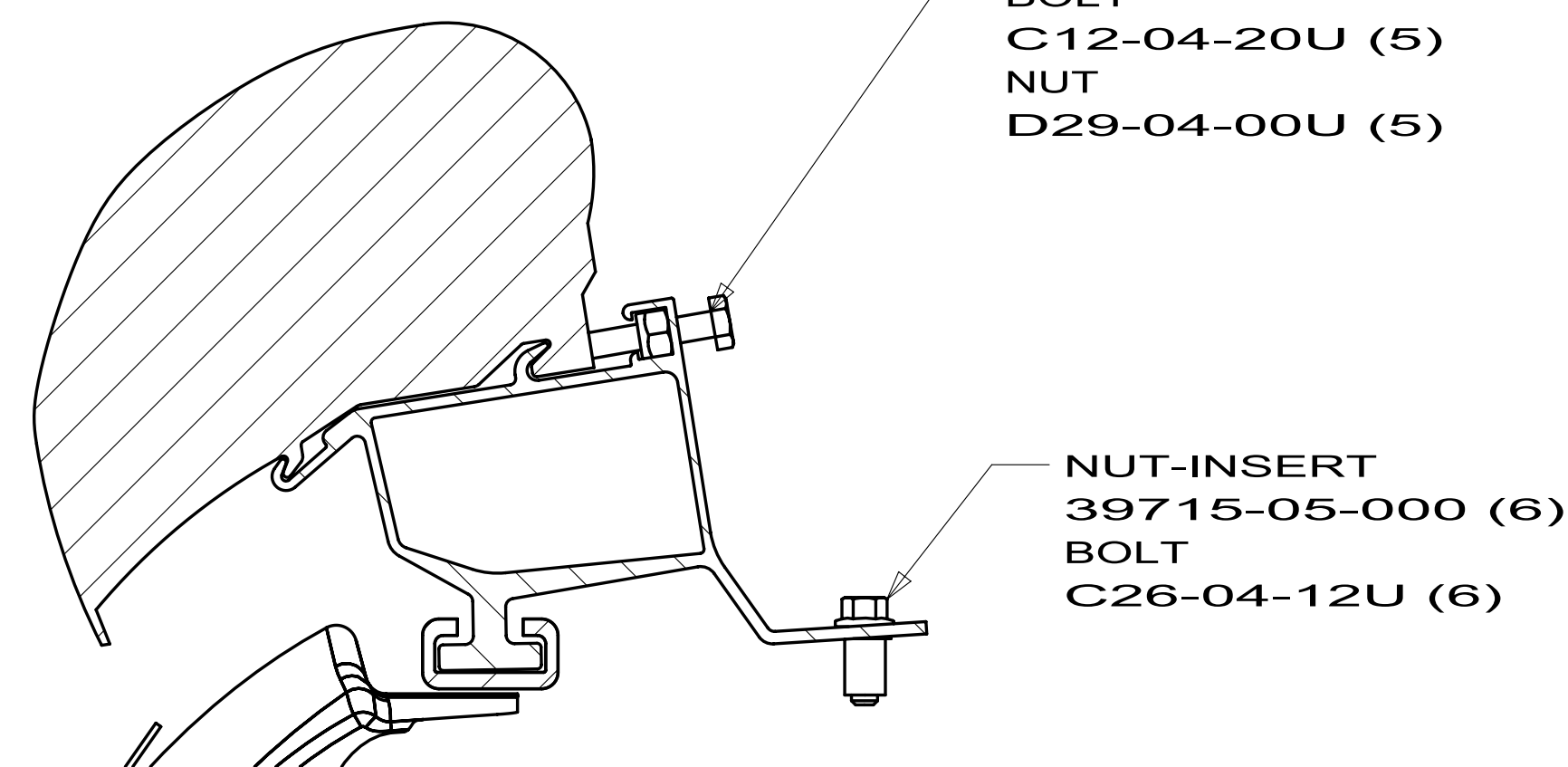
SECTION E-E
