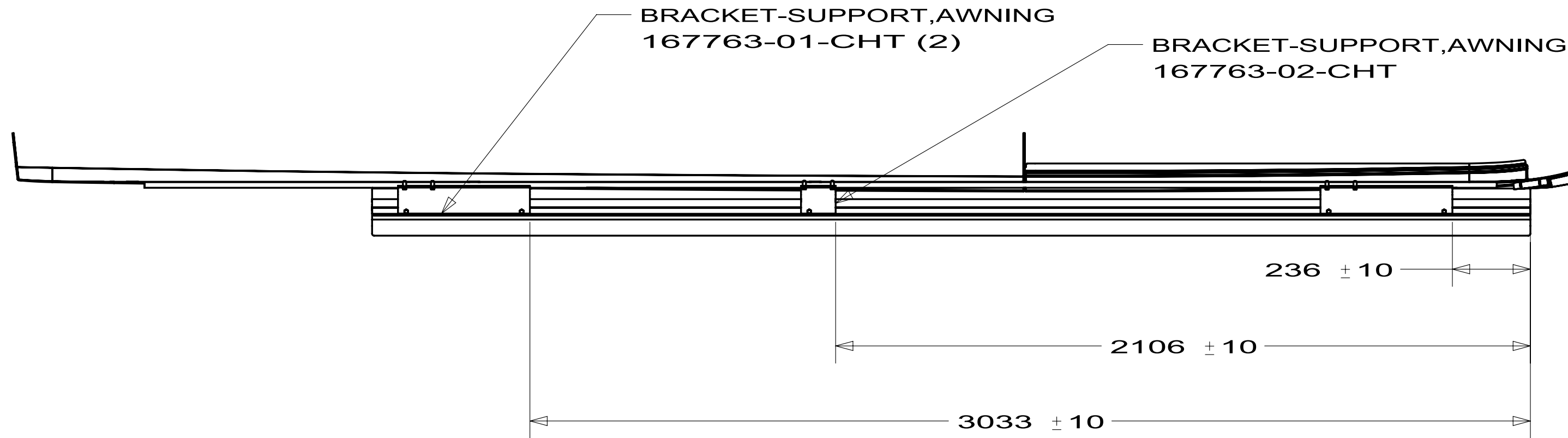
VIEW D
