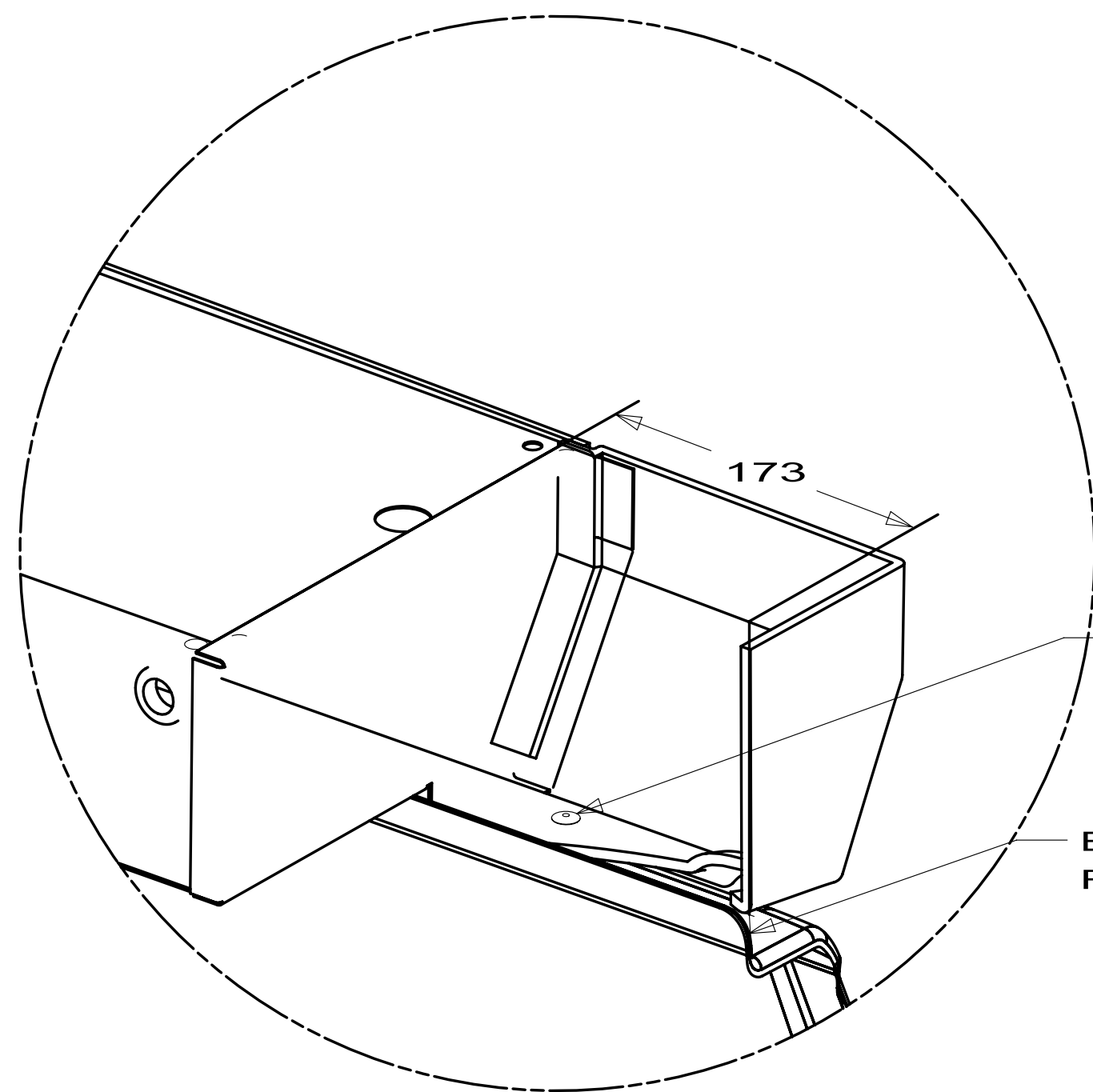
DETAIL C
