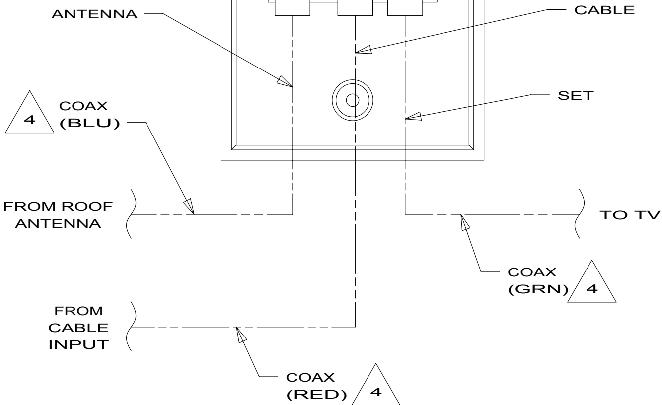
DETAIL BD
