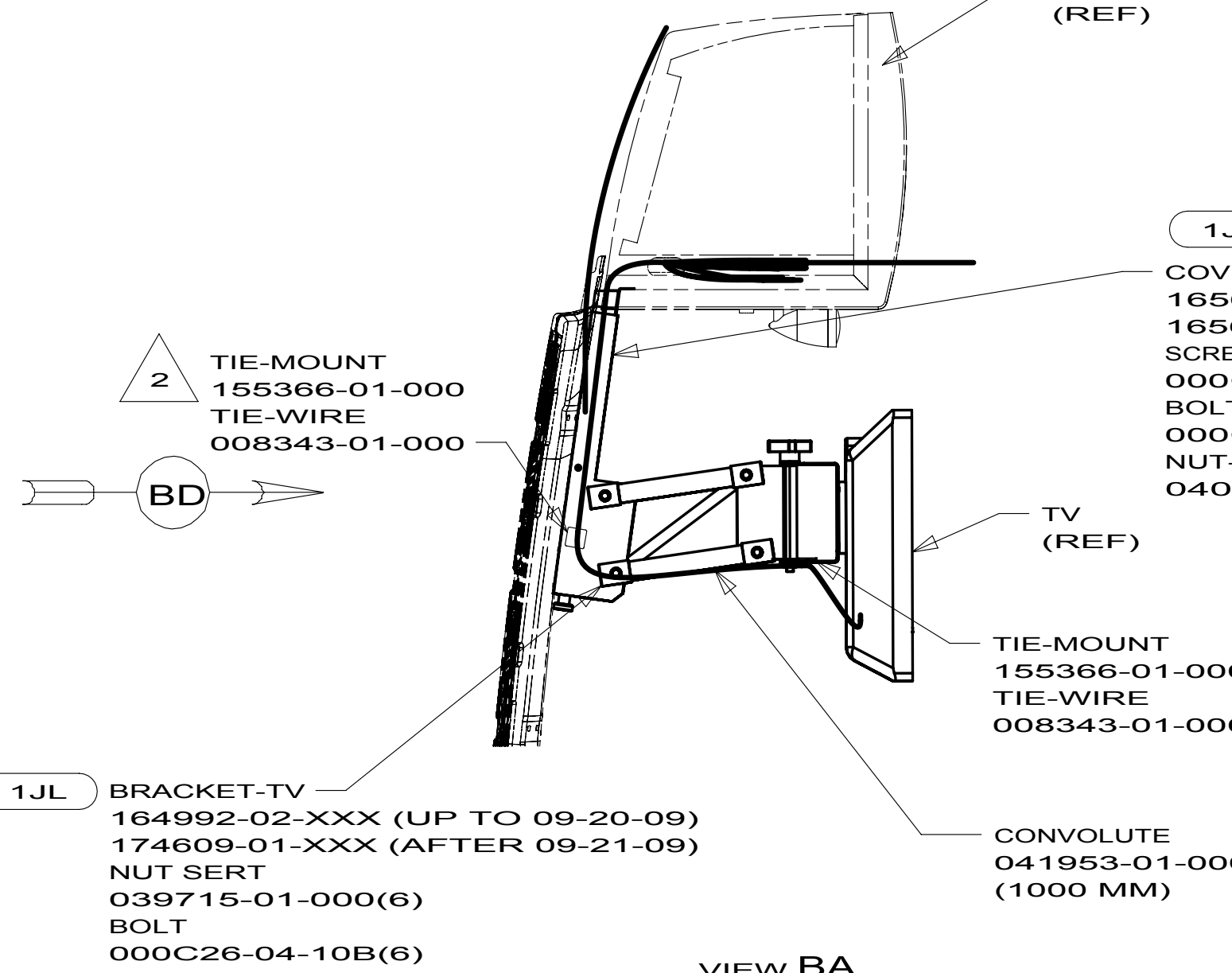
VIEW BA
