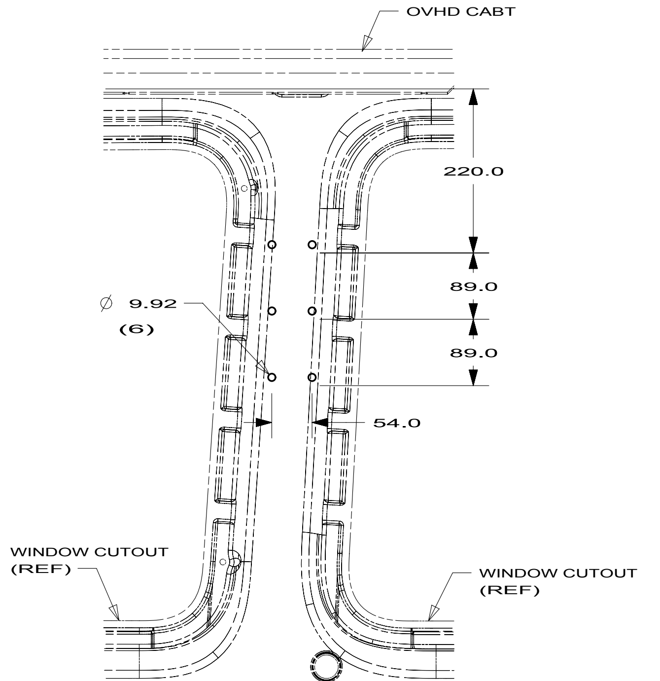
VIEW BB 1JL
