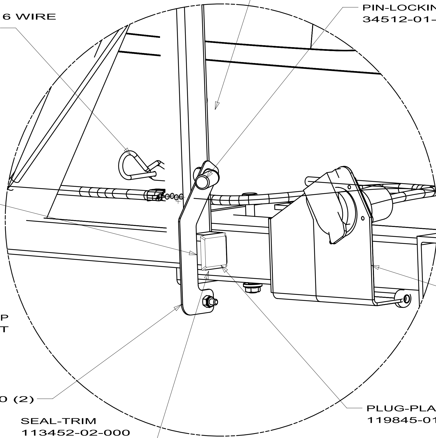
DETAIL BB
