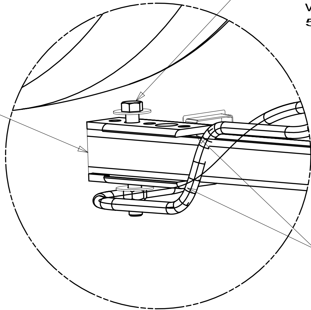
DETAIL BA
