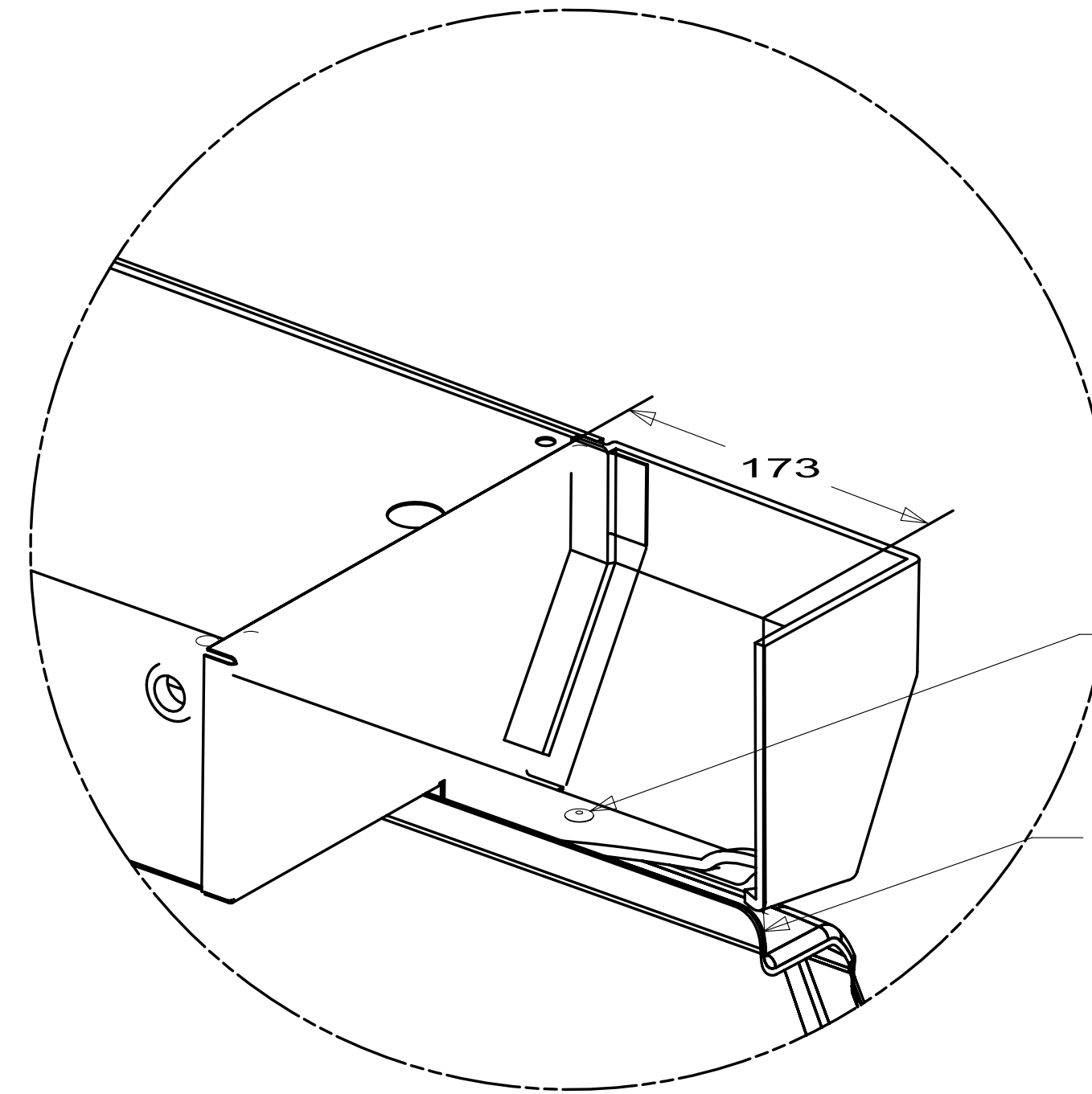
DETAIL C
