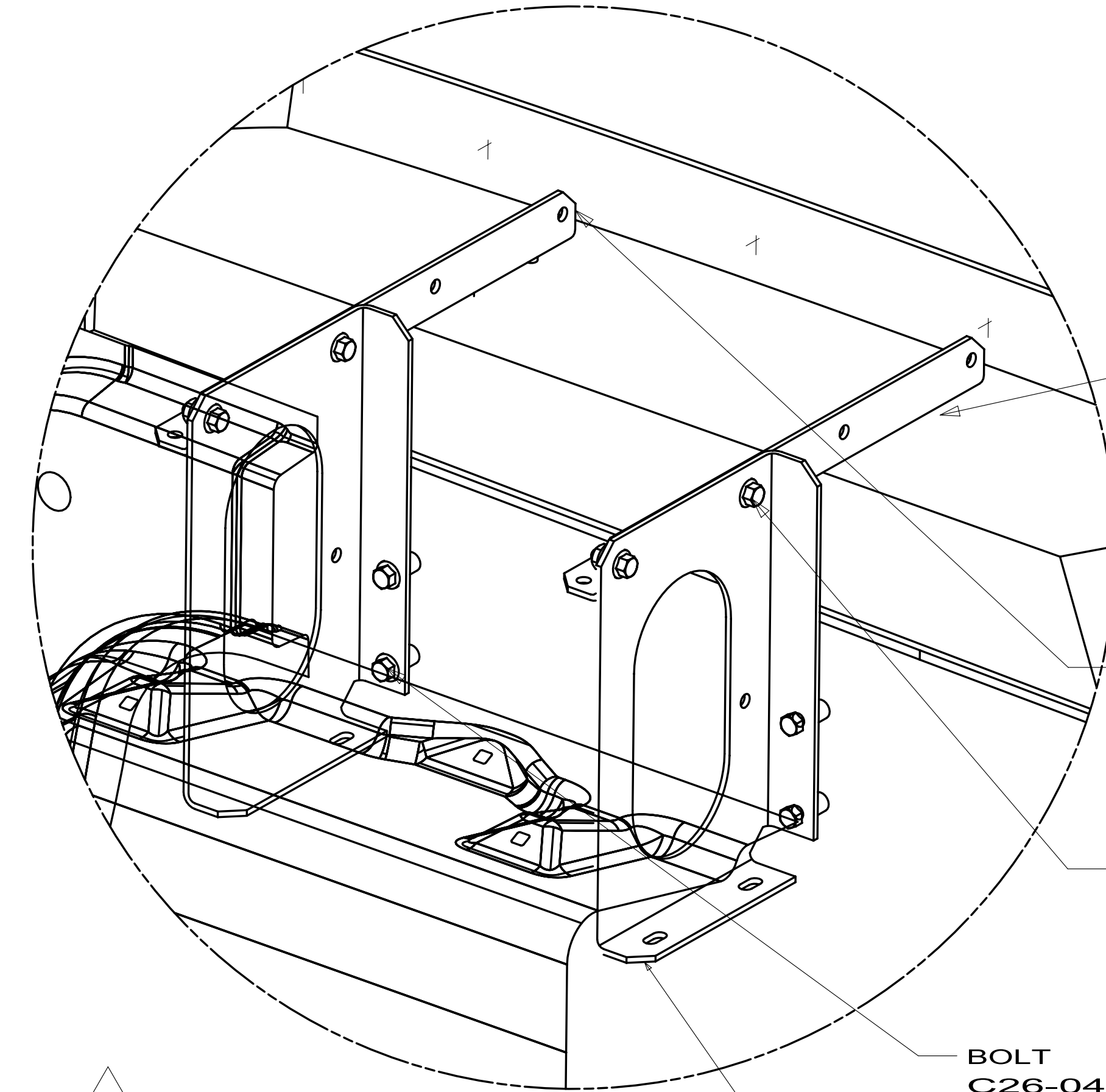
DETAIL CB
