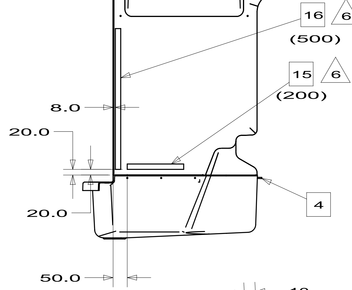
SHOWER PAN ASM M02673-21-Y27
