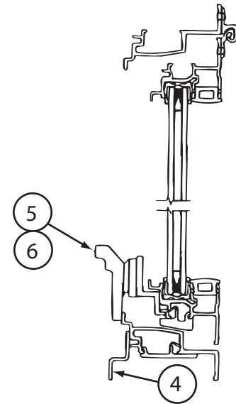
CROSS SECTION A-A
