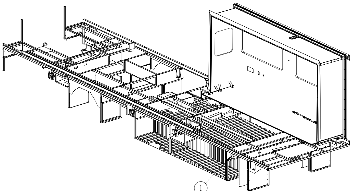
ACCESSORY INSTALLATION
