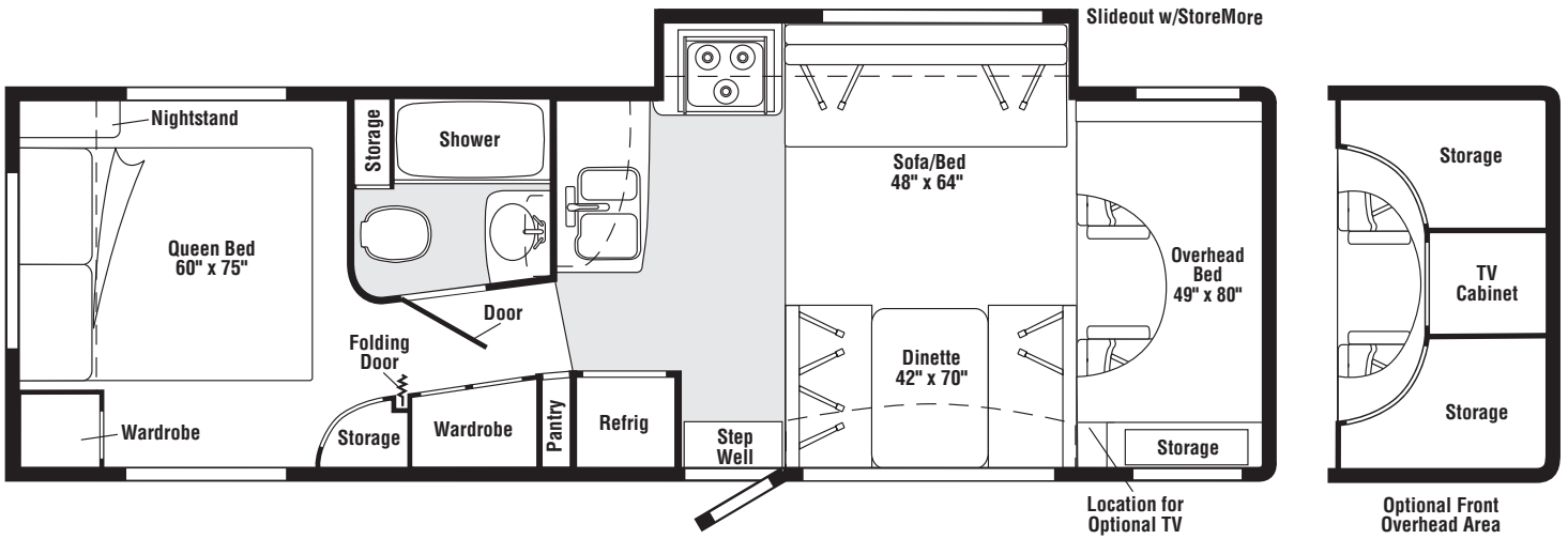
FLOORPLAN
