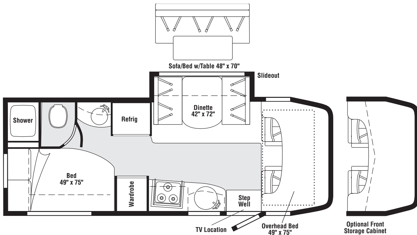
FLOORPLAN
