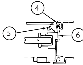
CROSS SECTION C-C
