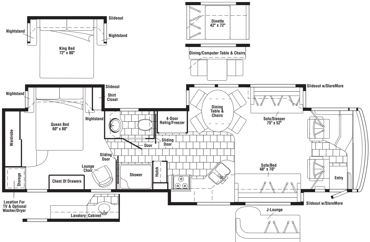
FLOORPLAN
