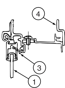
CROSS SECTION D-D
