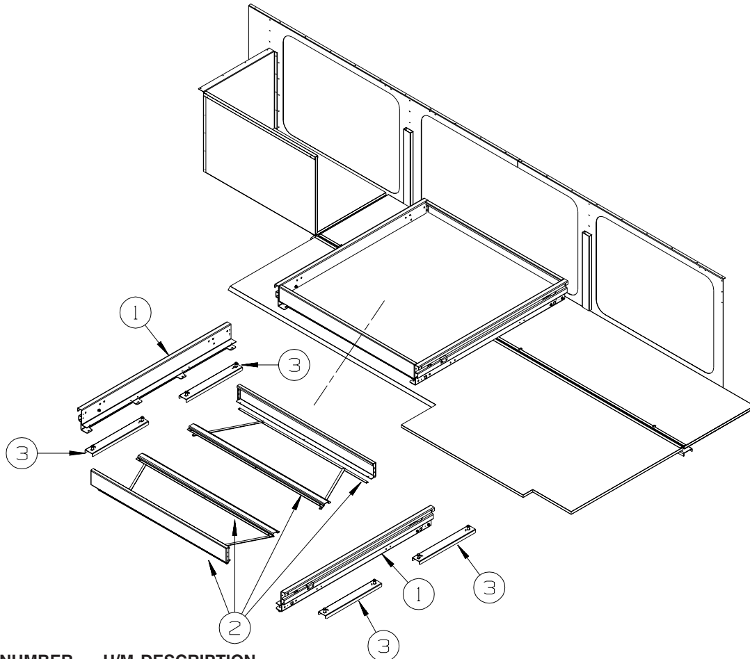
SLIDING TRAY
