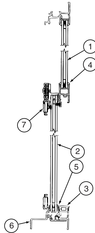
CROSS SECTION A-A
