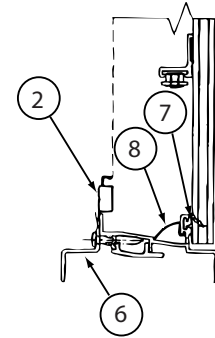
CROSS SECTION B-B
