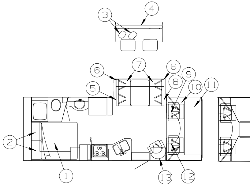
CUSHION LAYOUT
