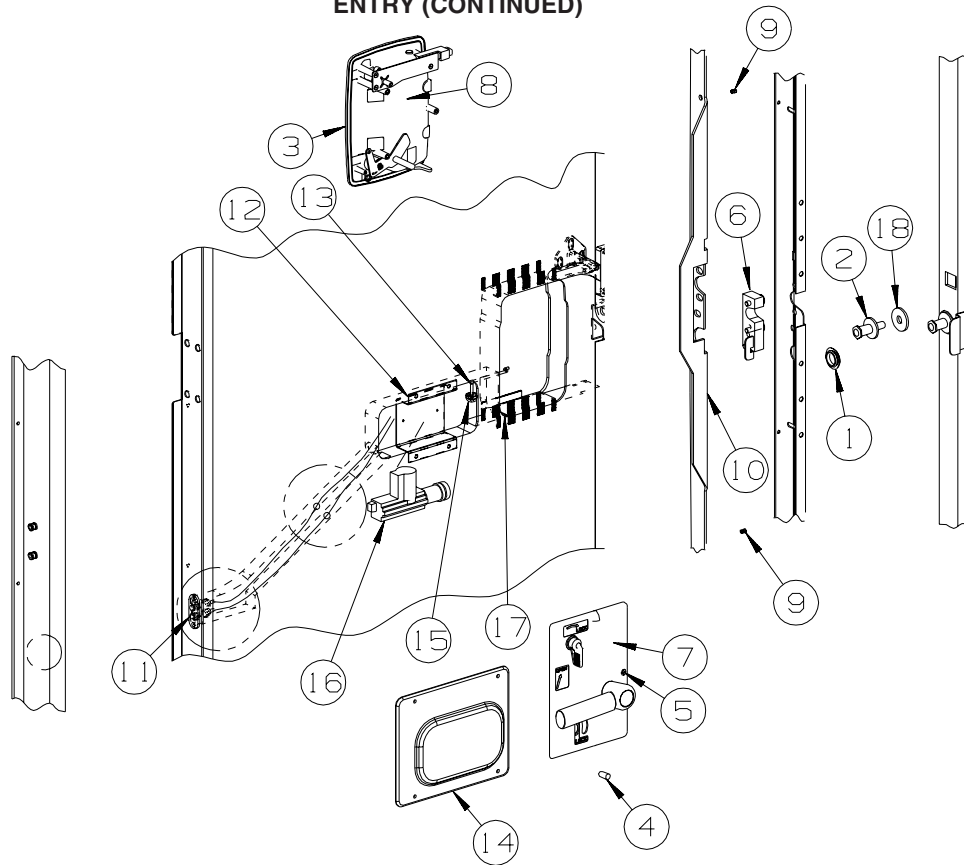
LATCH - ENTRY
