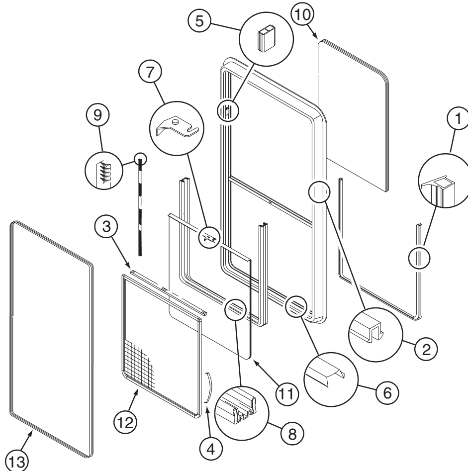
COMPONENT PARTS FOR WINDOW & VENT LAYOUT
