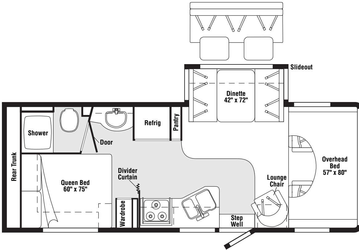
FLOORPLAN
