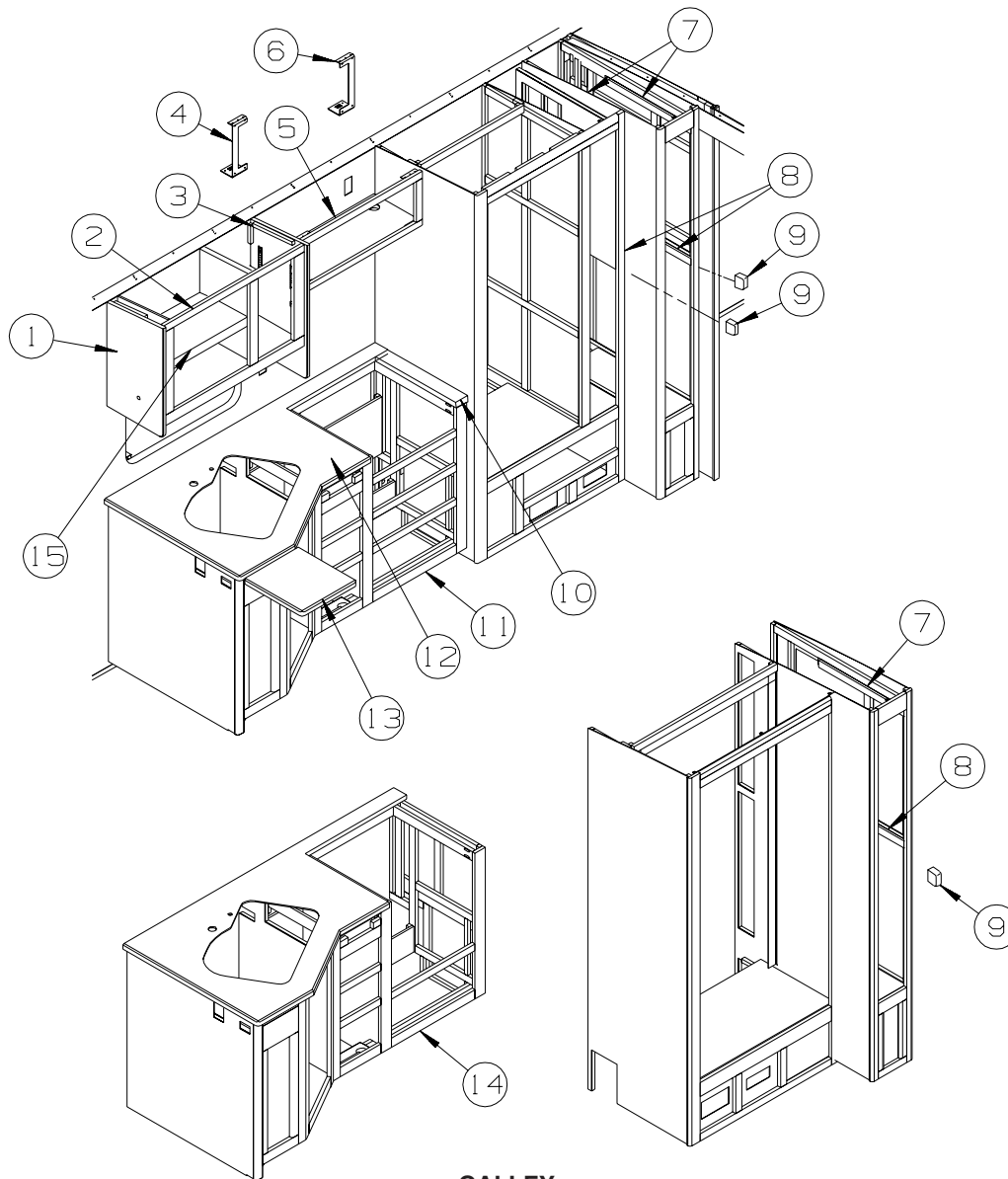
GALLEY
