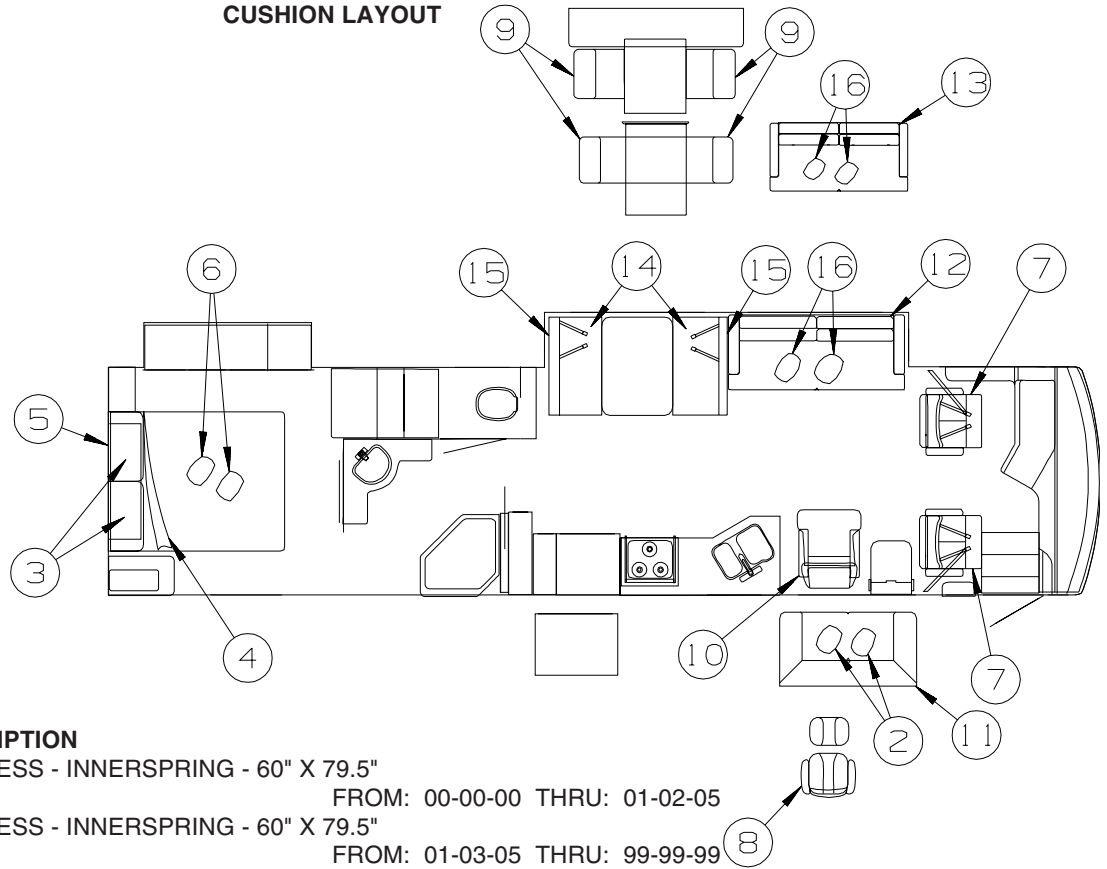
CUSHION LAYOUT
