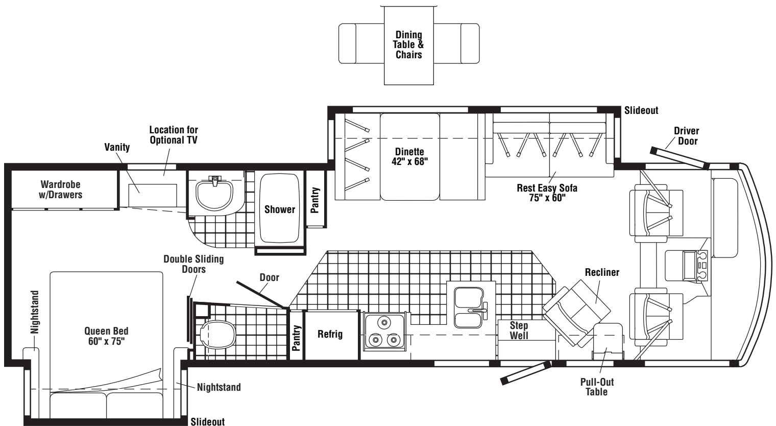
FLOORPLAN
