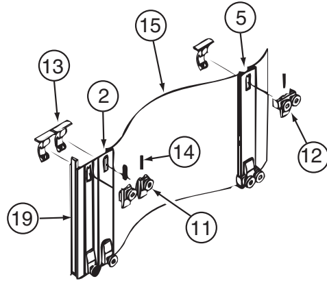
Roller Assembly Detail
