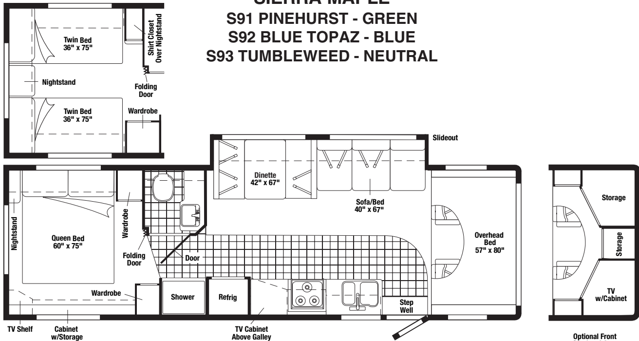
FLOORPLAN
