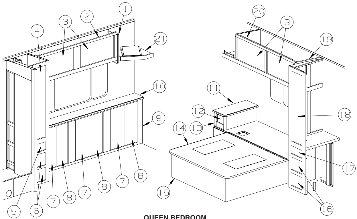
QUEEN BEDROOM
