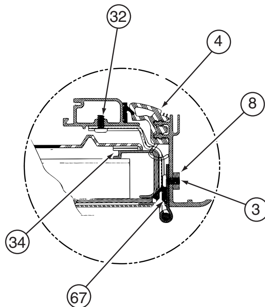
SECTION B-B
