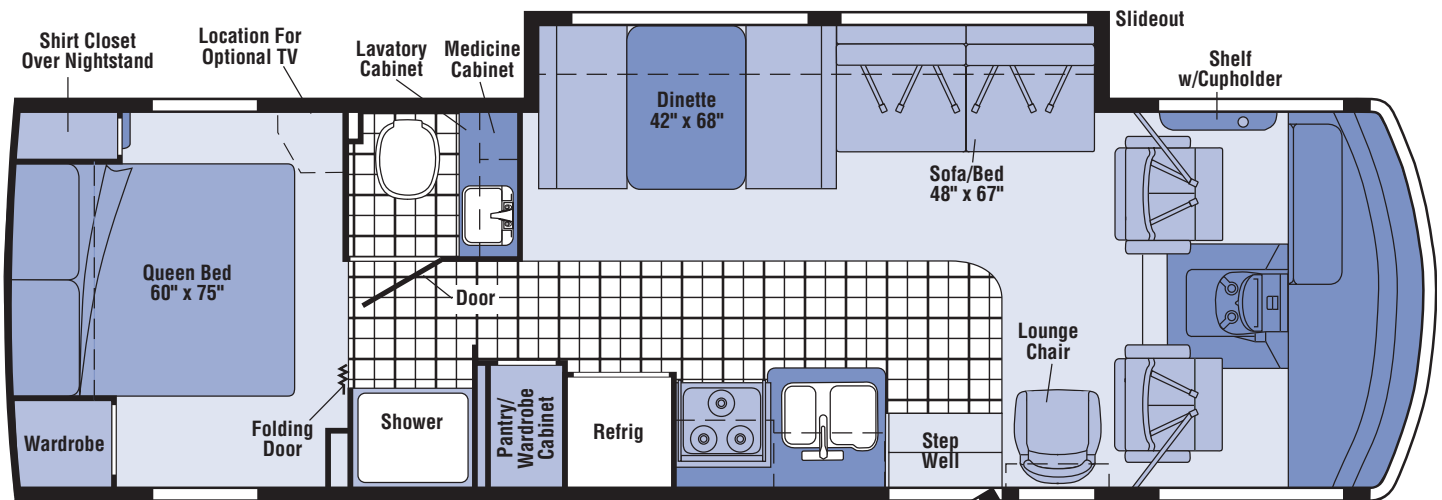
FLOORPLAN
